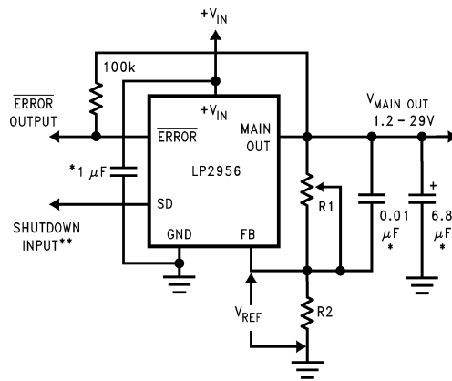
FIGURE 3. Adjustable Regulator
