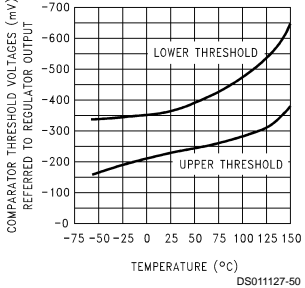
Dropout Detection Comparator Threshold Voltages
