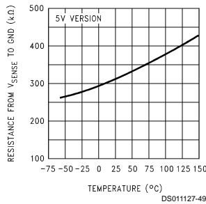
Divider Resistance
