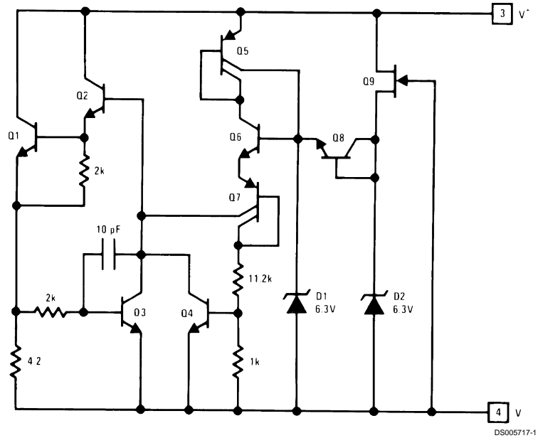
Temperature Stabilizer
