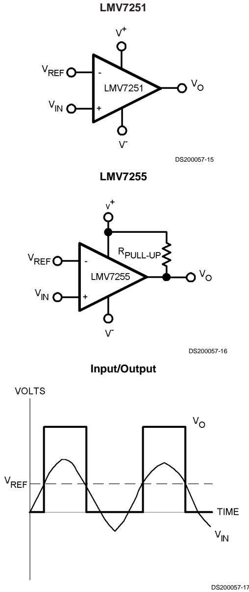
FIGURE 2. Basic Comparator
