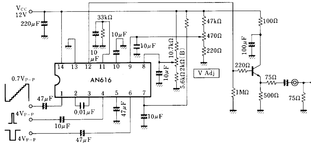
Test Circuit 4 ( V_{(r)} )
