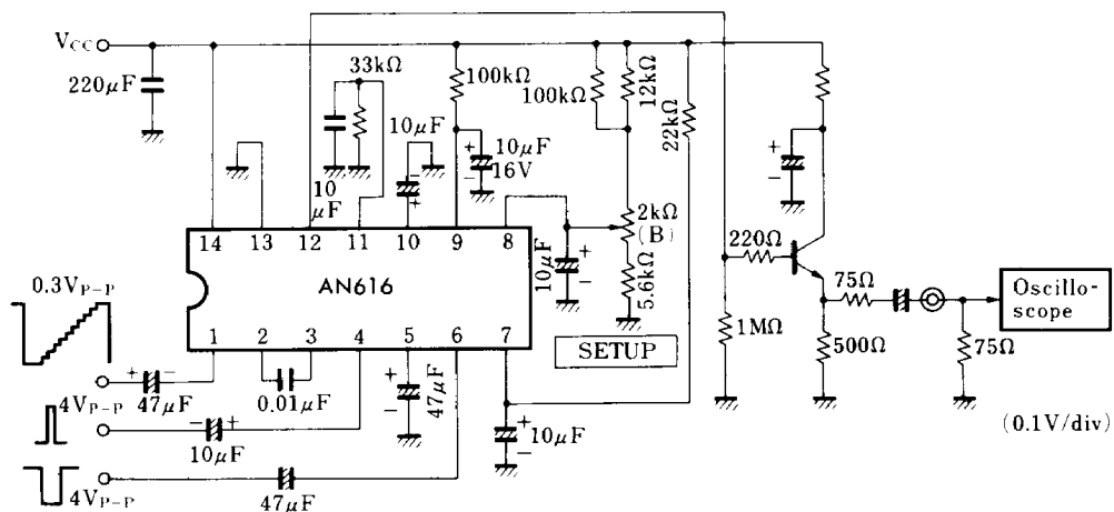
Test Circuit 1 (G V )
