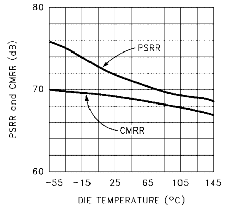
PSSR and CMRR vs Die Temperature
