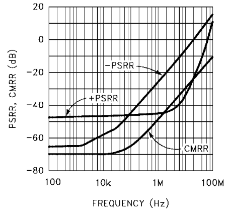
PSSR and CMRR vs Frequency
