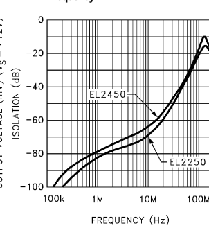
Channel to Channel Isolation vs Frequency
