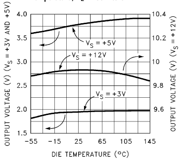
Positive Output Voltage Swing vs Die Temperature, R_L = 150Ω to GND
