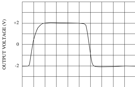
Large Signal Pulse Response (Split Supplies)
