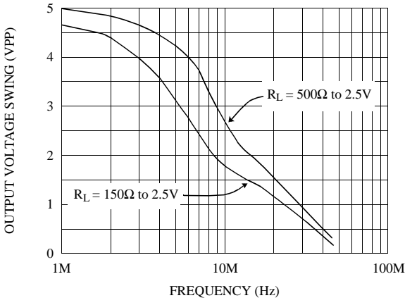
Output Voltage Swing vs. Frequency for THD < 1%
