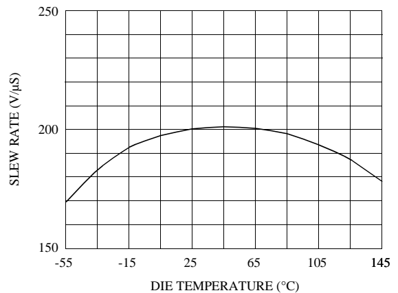
Slew Rate vs. Die Temperature
