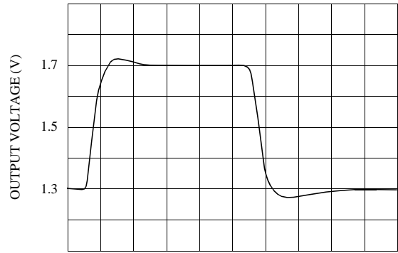
Small Signal Pulse Response (Single Supply)
