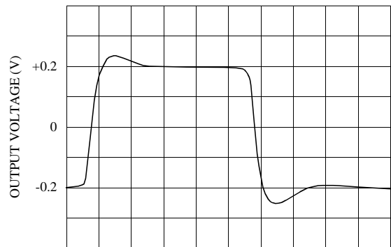
Small Signal Pulse Response (Split Supply)
