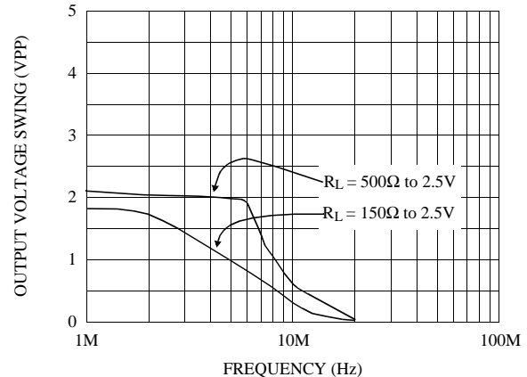
Output Voltage Swing vs. Frequency for THD < 0.1%
