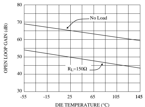
Open Loop Voltage Gain vs. Die Temperature
