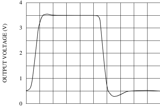
Large Signal Pulse Response (Single Supply)
