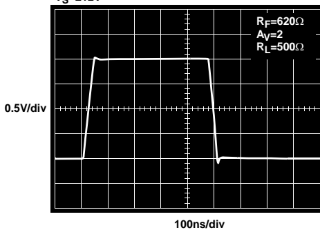
Large Signal Step Response V_S = \pm 12V
