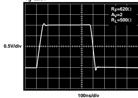
Large Signal Step Response V_S = \pm 2.5V
