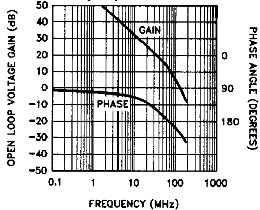
Open Loop Voltage Gain vs Frequency
