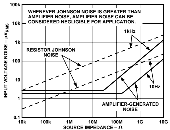
Figure 39. Total Noise vs. Source Impedance
