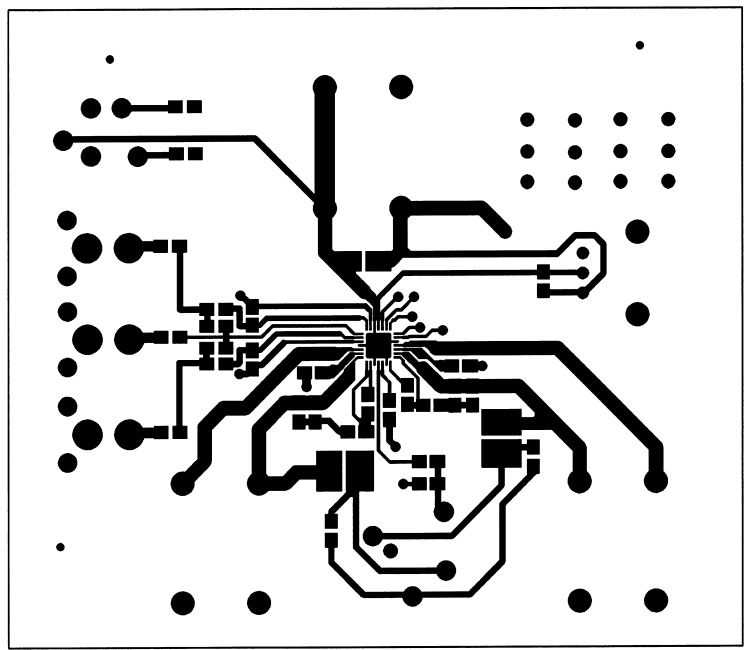
FIGURE 6. Recommended LQ PC Board Layout: Component-Side Layout
