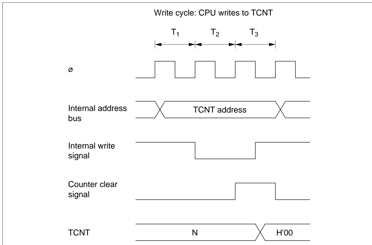
Figure 9.10 TCNT Write-Clear Contention
