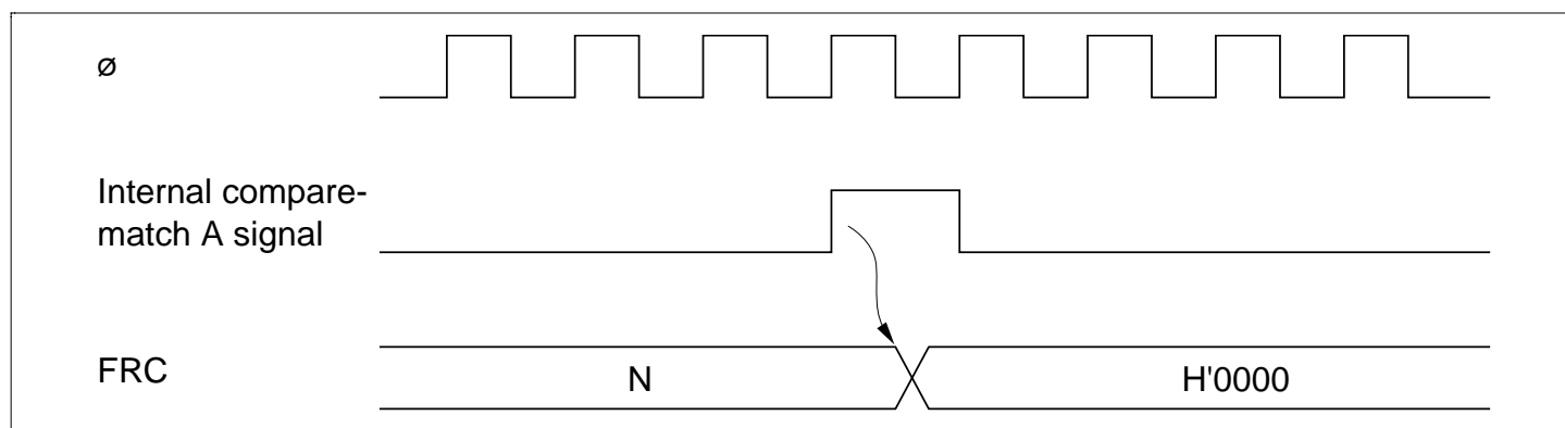
Figure 8.7 Clearing of FRC by Compare-Match A
