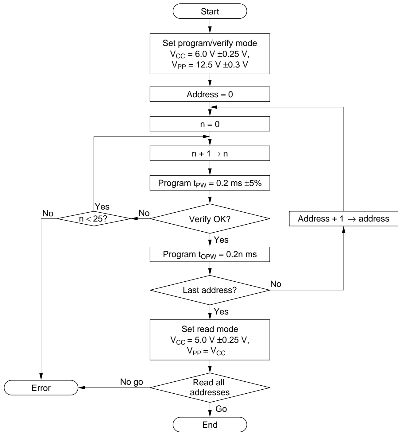
Figure 18.5 High-Speed Programming Flowchart
