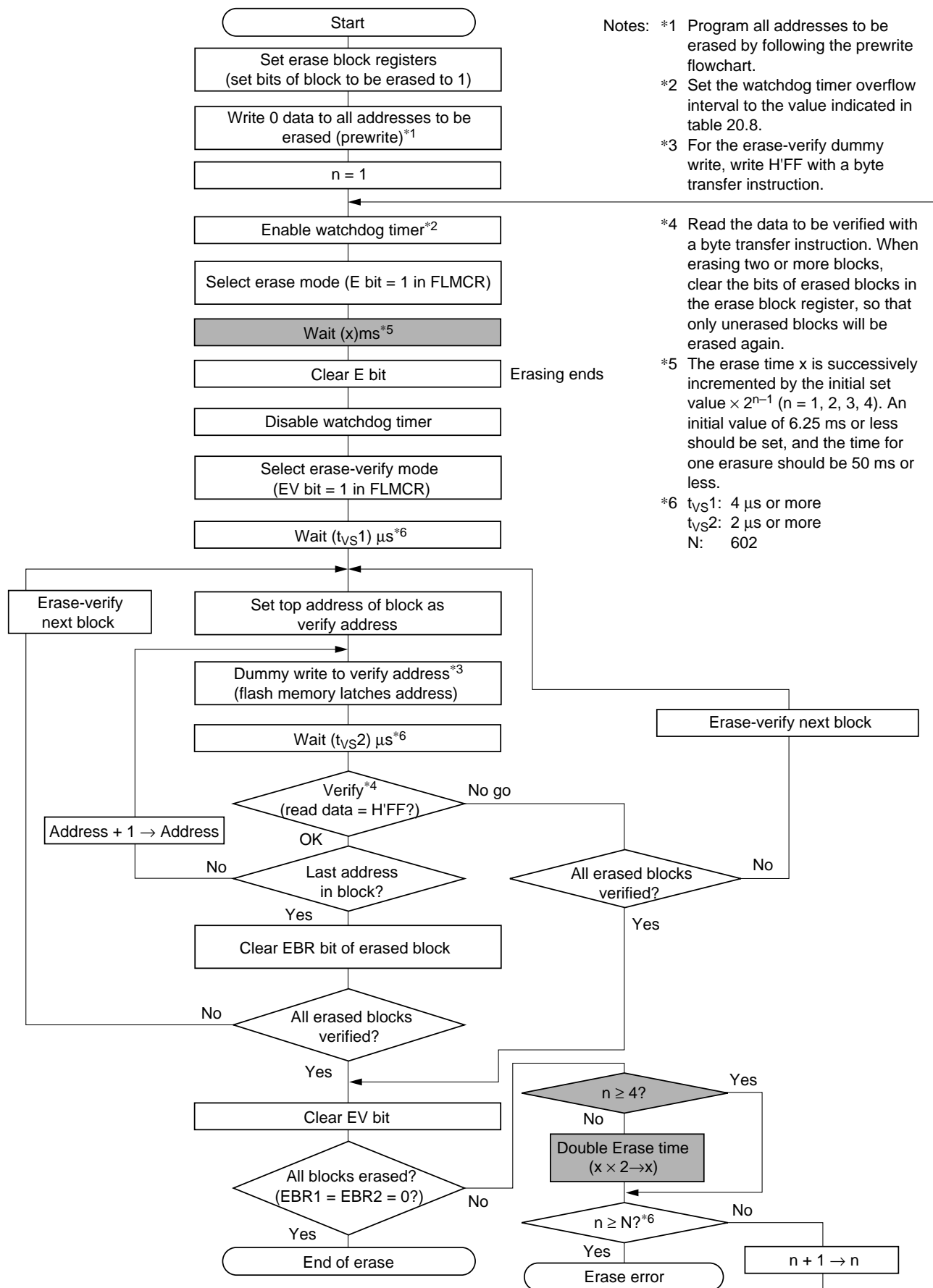
Figure 20.11 Multiple-Block Erase Flowchart
