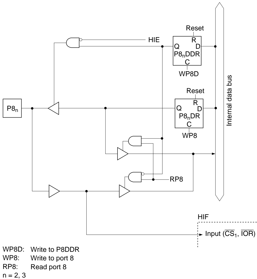
Figure C.8 (c) Port 8 Block Diagram (Pins P8 2 , P8 3 )
