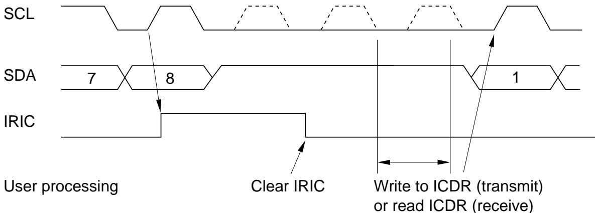
Figure 13.10 IRIC Set Timing and SCL Control
