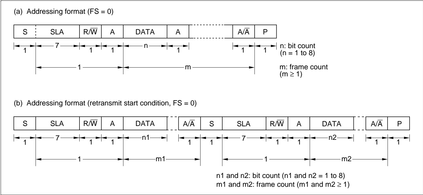
Figure 13.3 I 2 C Bus Data Formats (Acknowledge Formats)
