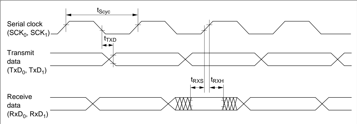
Figure 23.19 SCI Input/Output Timing (Synchronous Mode)
