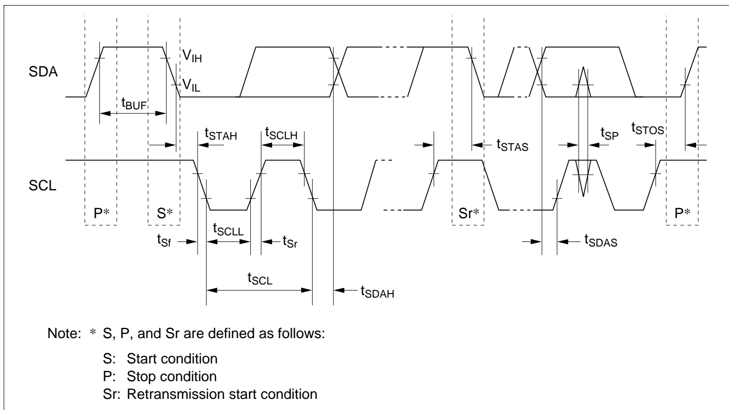
Figure 23.24 I 2 C Interface Input/Output Timing
