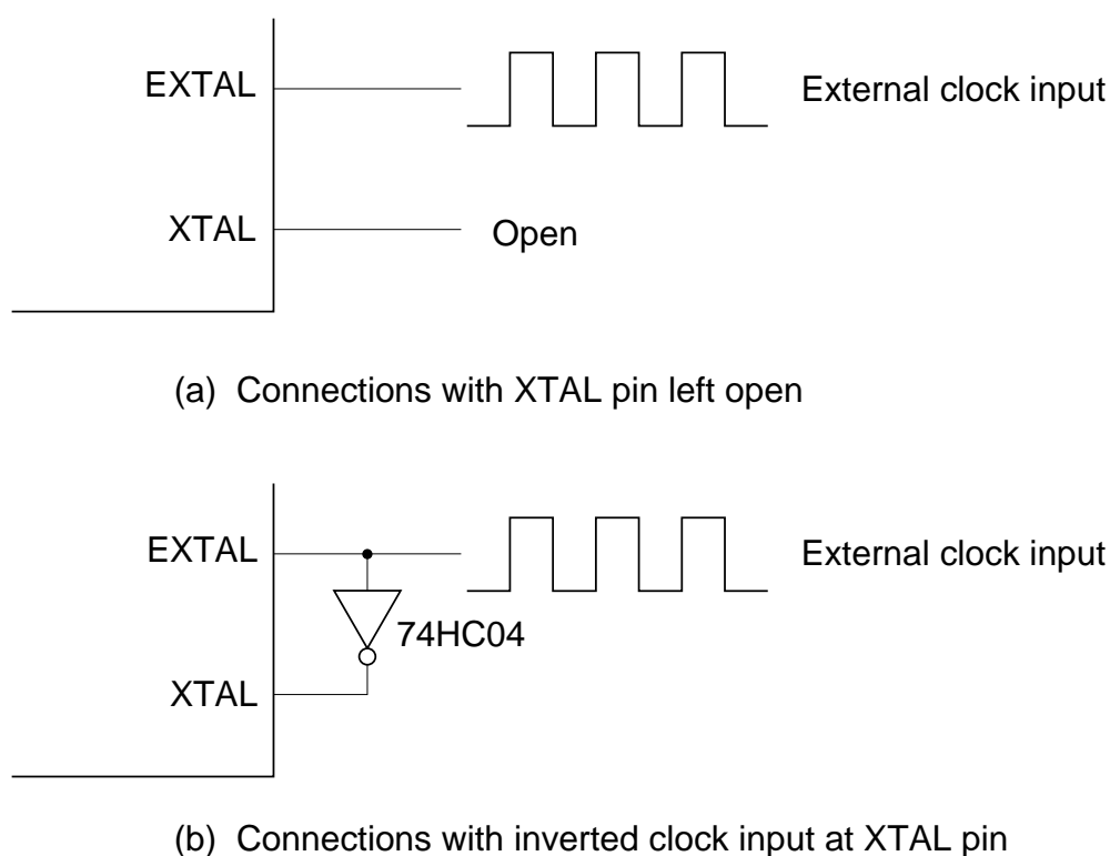
Figure 6.5 External Clock Input (Example)
