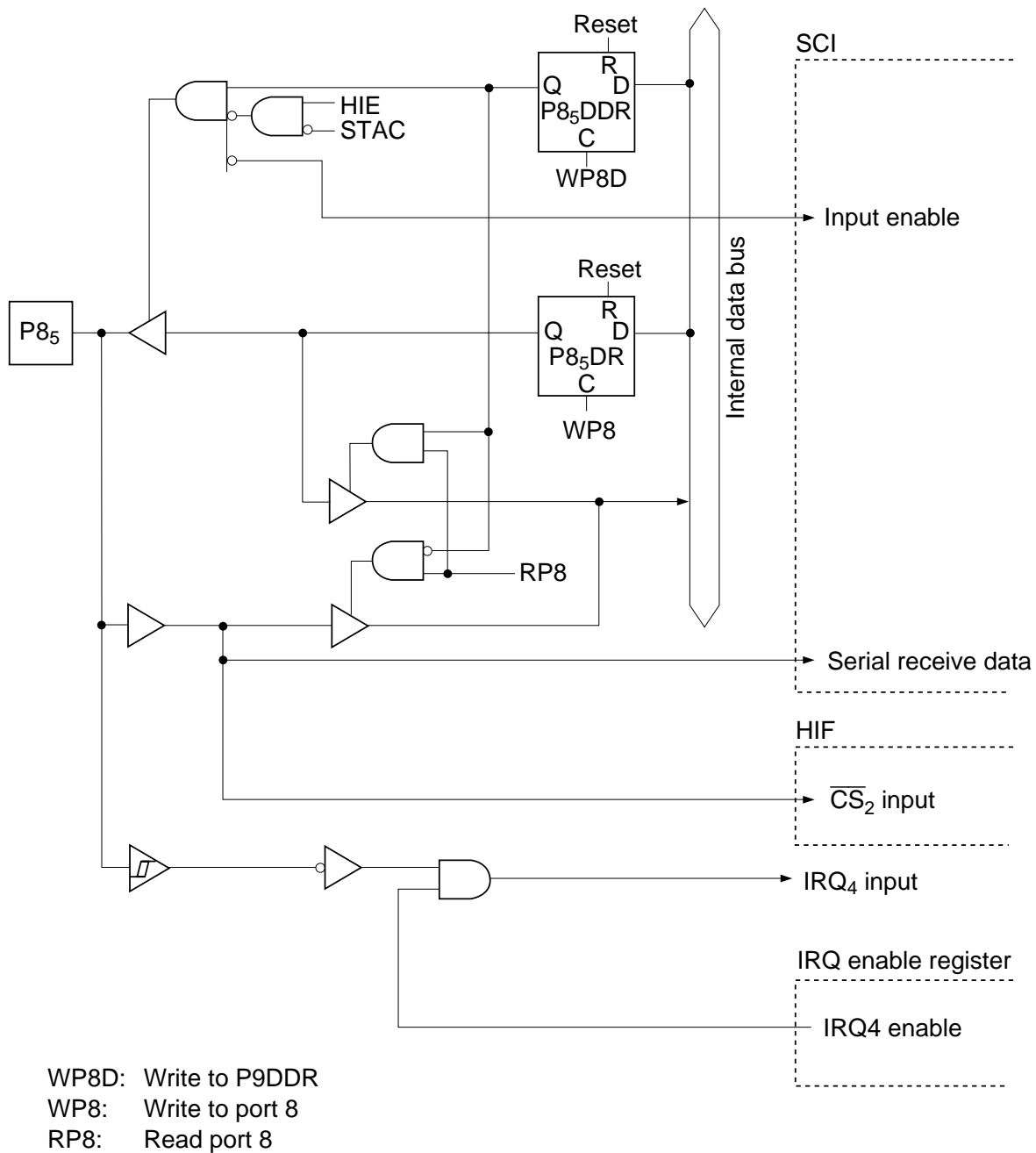
Figure C.8 (e) Port 8 Block Diagram (Pin P8 5 )
