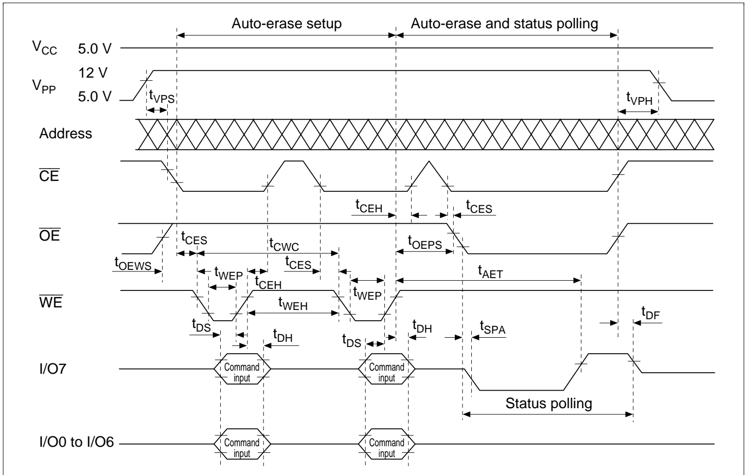
Figure 19.17 Auto-Erase Timing
