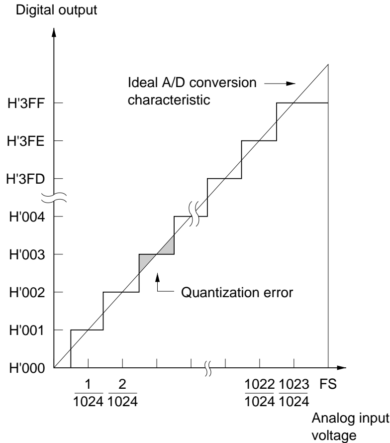
Figure 15.8 A/D Conversion Accuracy Definitions (1)
