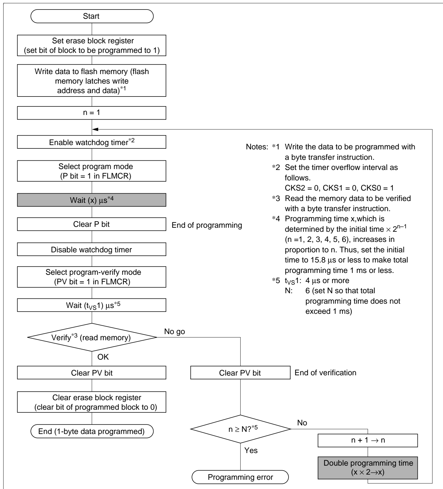
Figure 20.8 Programming Flowchart
