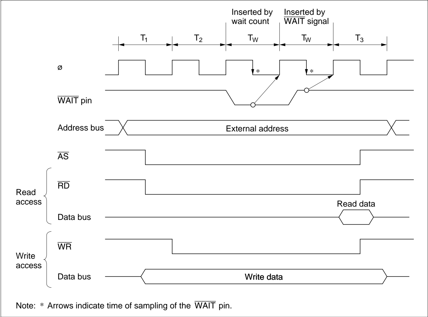
Figure 5.3 Pin Wait Mode
