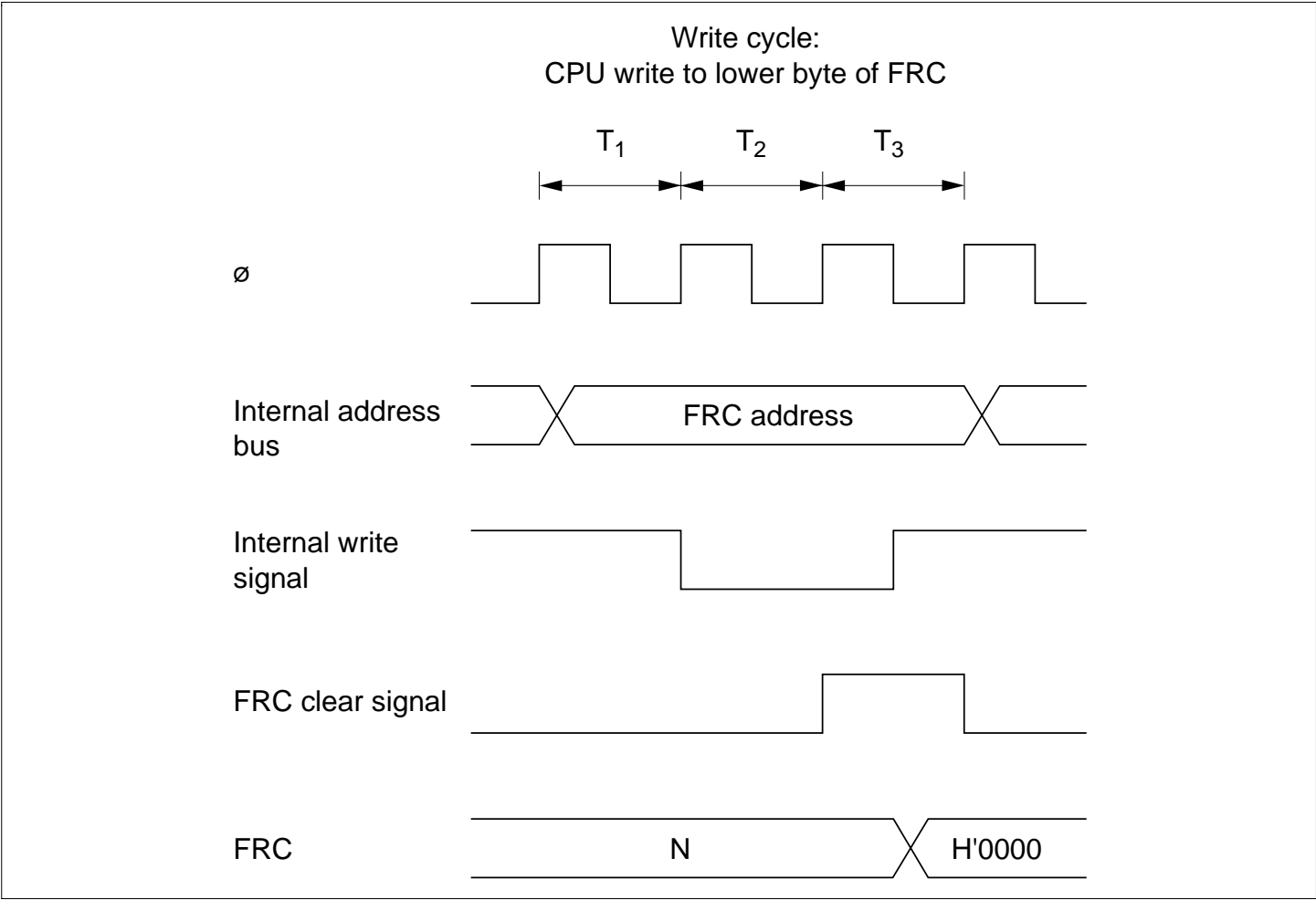
Figure 8.16 FRC Write-Clear Contention
