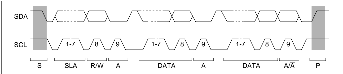
Figure 13.5 I²C Bus Timing
