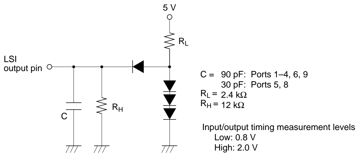
Figure 23.3 Output Load Circuit
