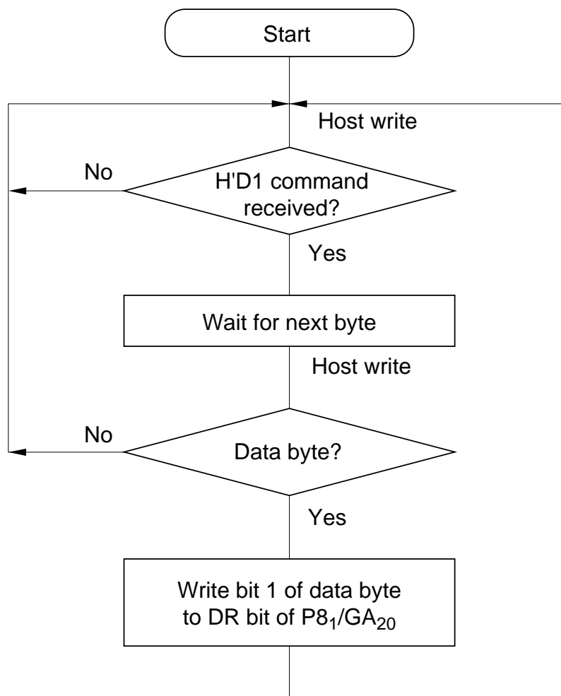
Figure 14.2 GA 20 Output
