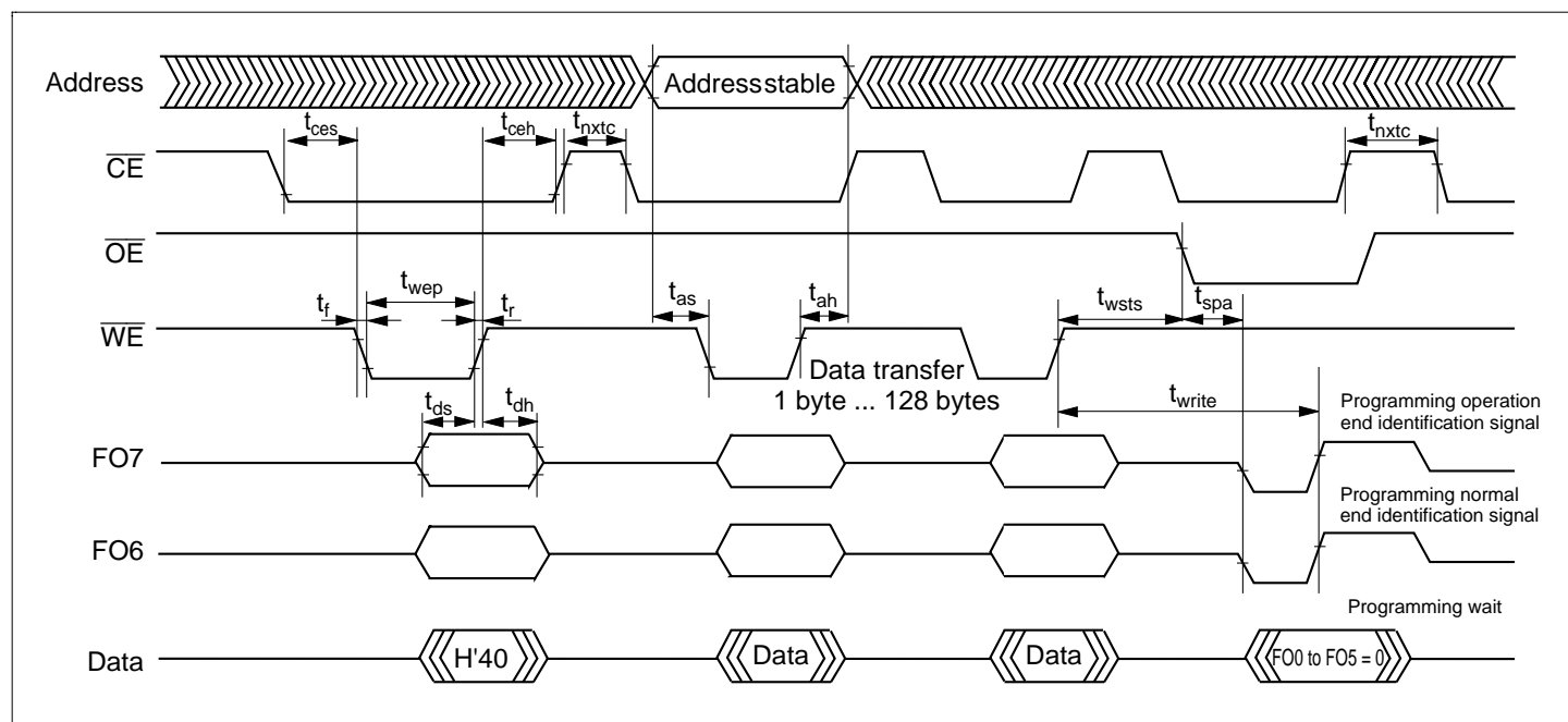
Figure 21.20 Auto-Program Mode Timing Waveforms
