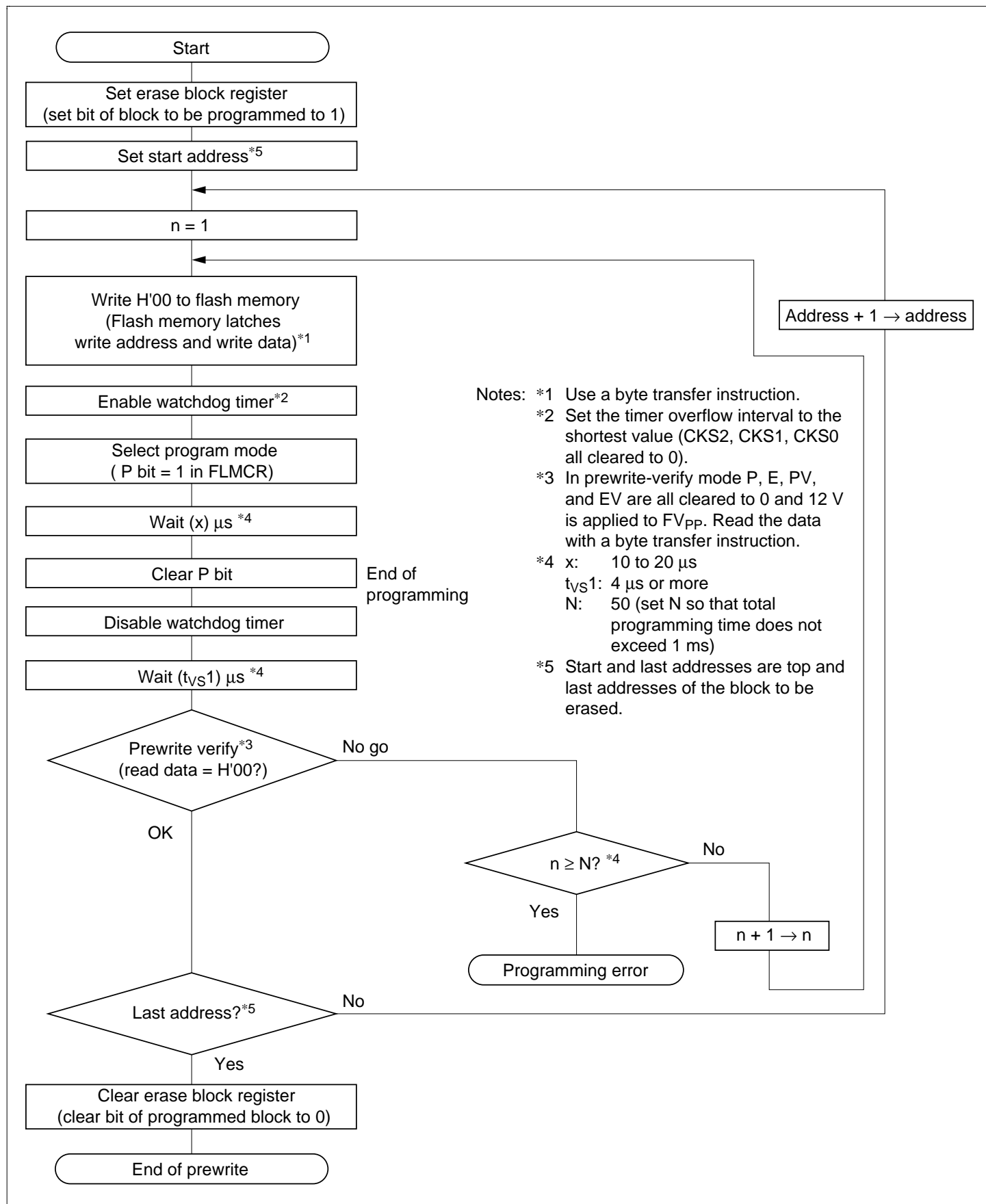
Figure 19.10 Prewrite Flowchart
