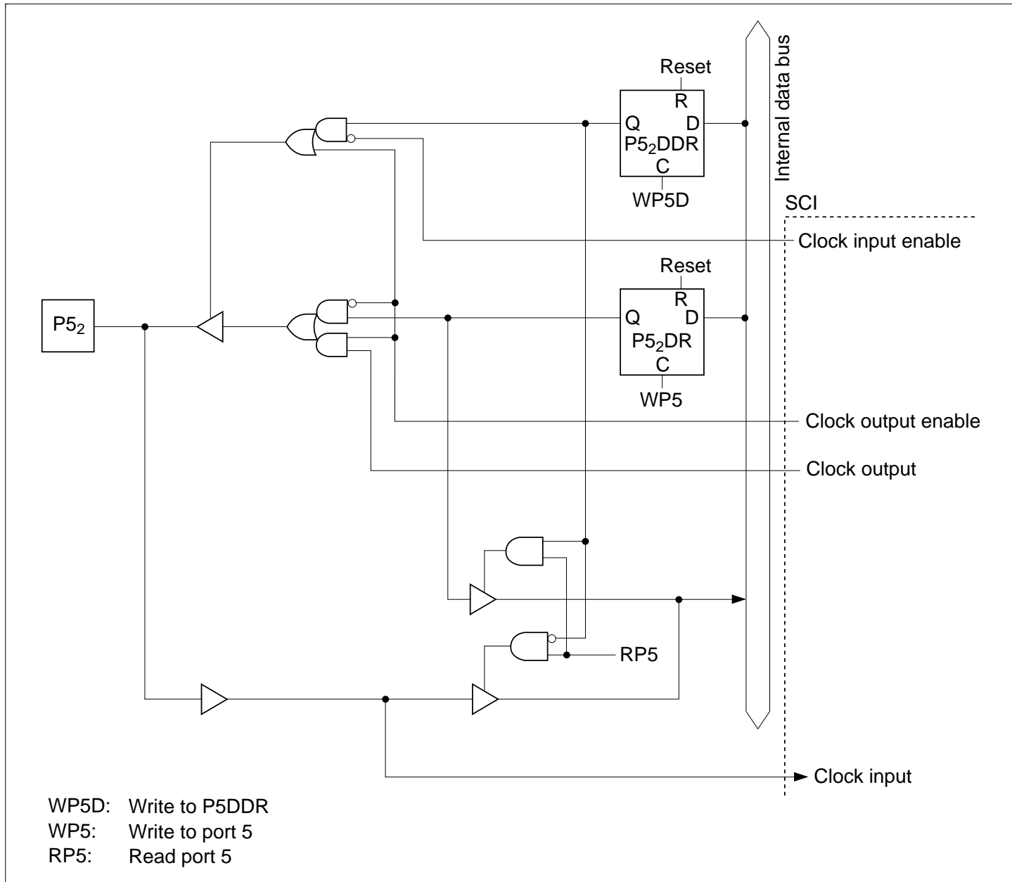
Figure C.5 (c) Port 5 Block Diagram (Pin P5 2 )
