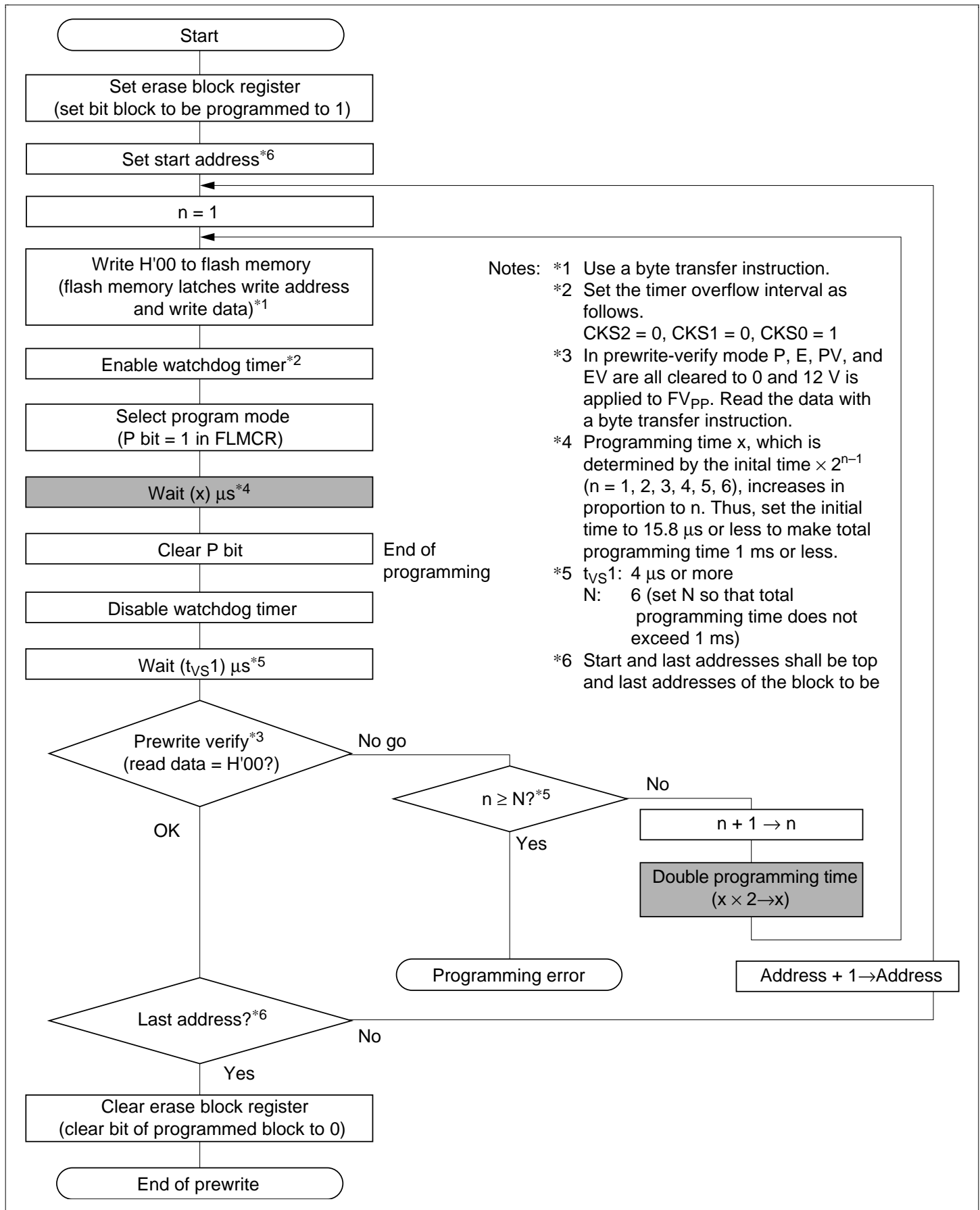
Figure 20.10 Prewrite Flowchart
