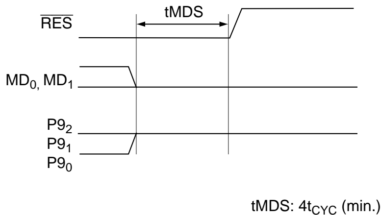
Figure 21.10 Programming Mode Timing
