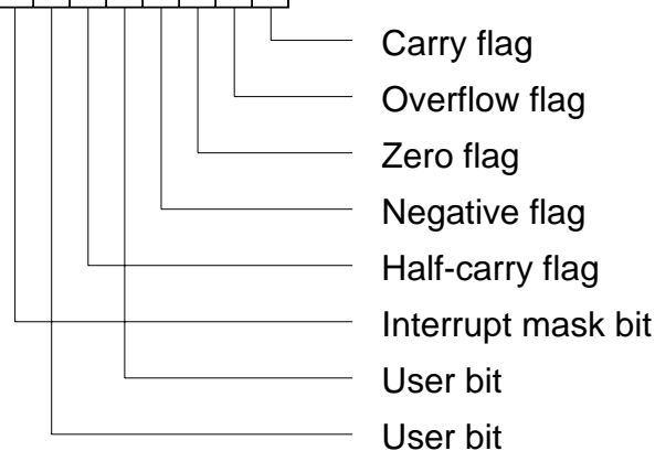
Figure 2.1 CPU Registers
