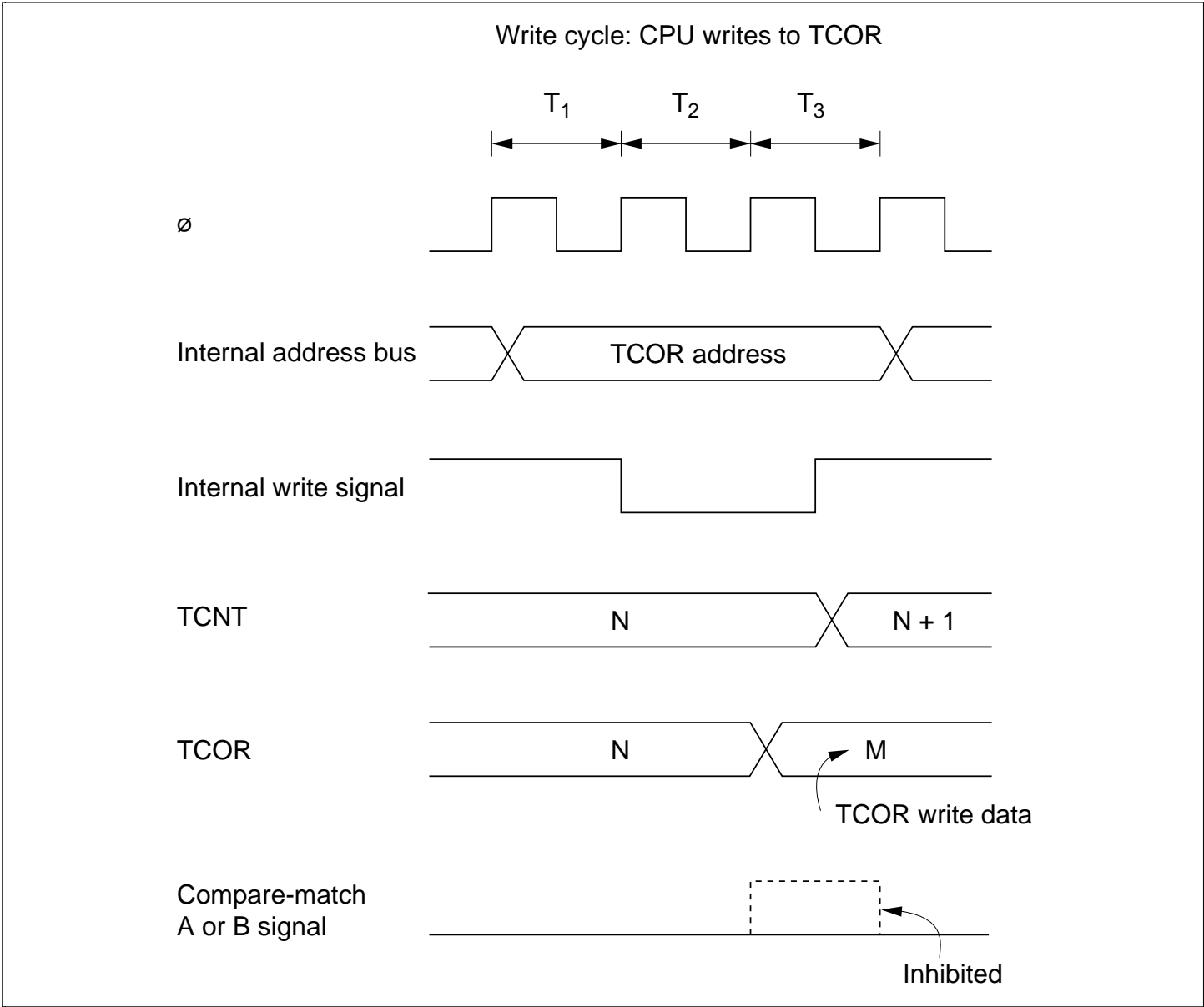
Figure 9.12 Contention between TCOR Write and Compare-Match
