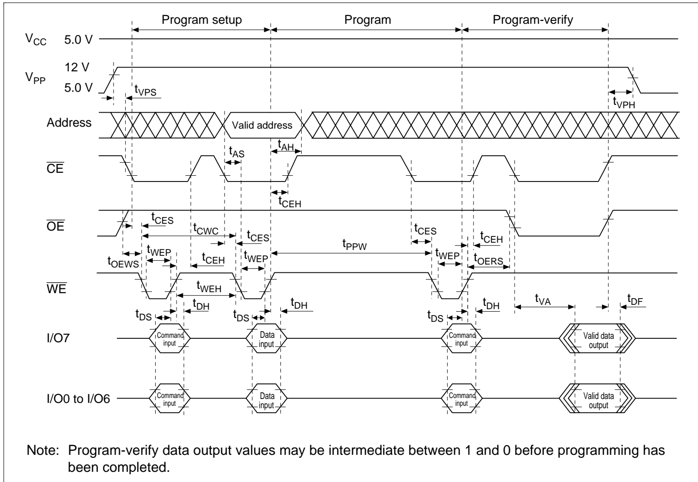
Figure 19.18 High-Speed, High-Reliability Programming Timing
