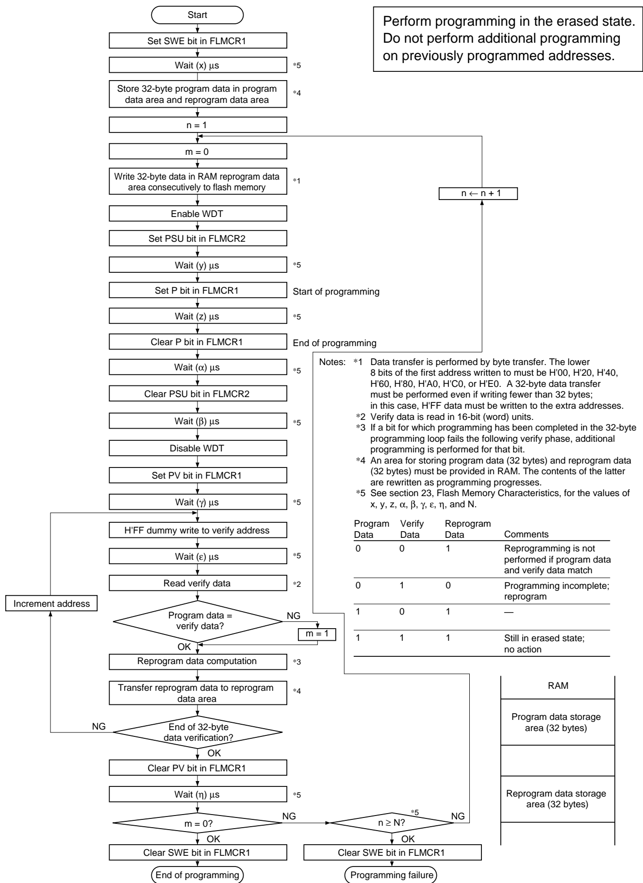
Figure 21.12 Program/Program-Verify Flowchart
