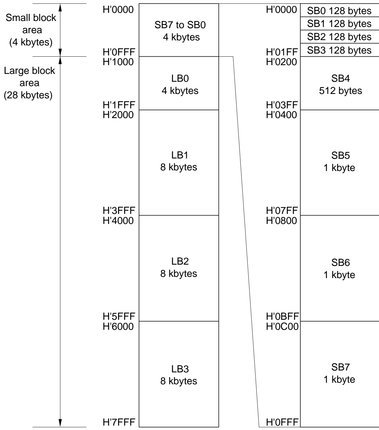
Figure 19.2 Erase Block Map
