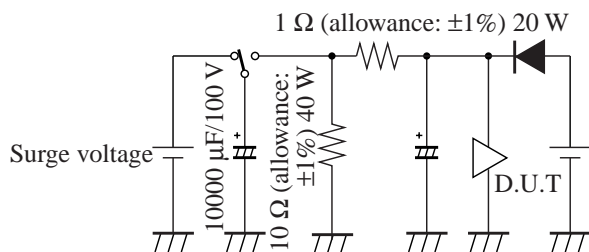
Figure 10. Power supply surge test circuit
