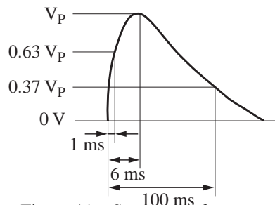
Figure 11. Surge waveform
