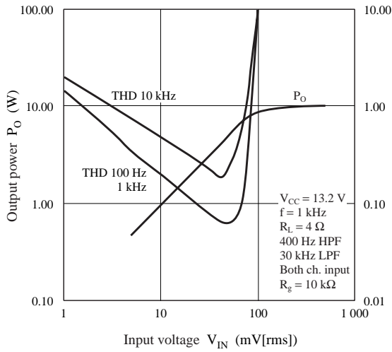
P_O , THD — V_{IN} ( R_L = 4 \Omega )
