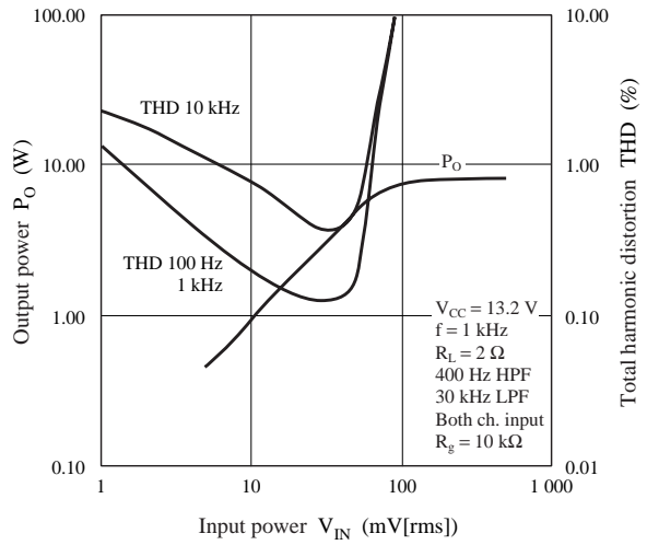
P_O , THD — V_{IN} ( R_L = 2 \Omega )
