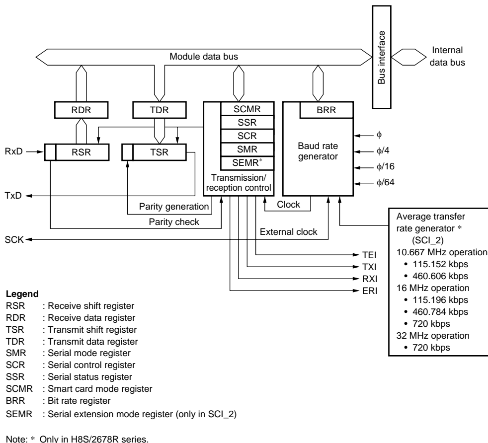
Figure 15.1 Block Diagram of SCI
