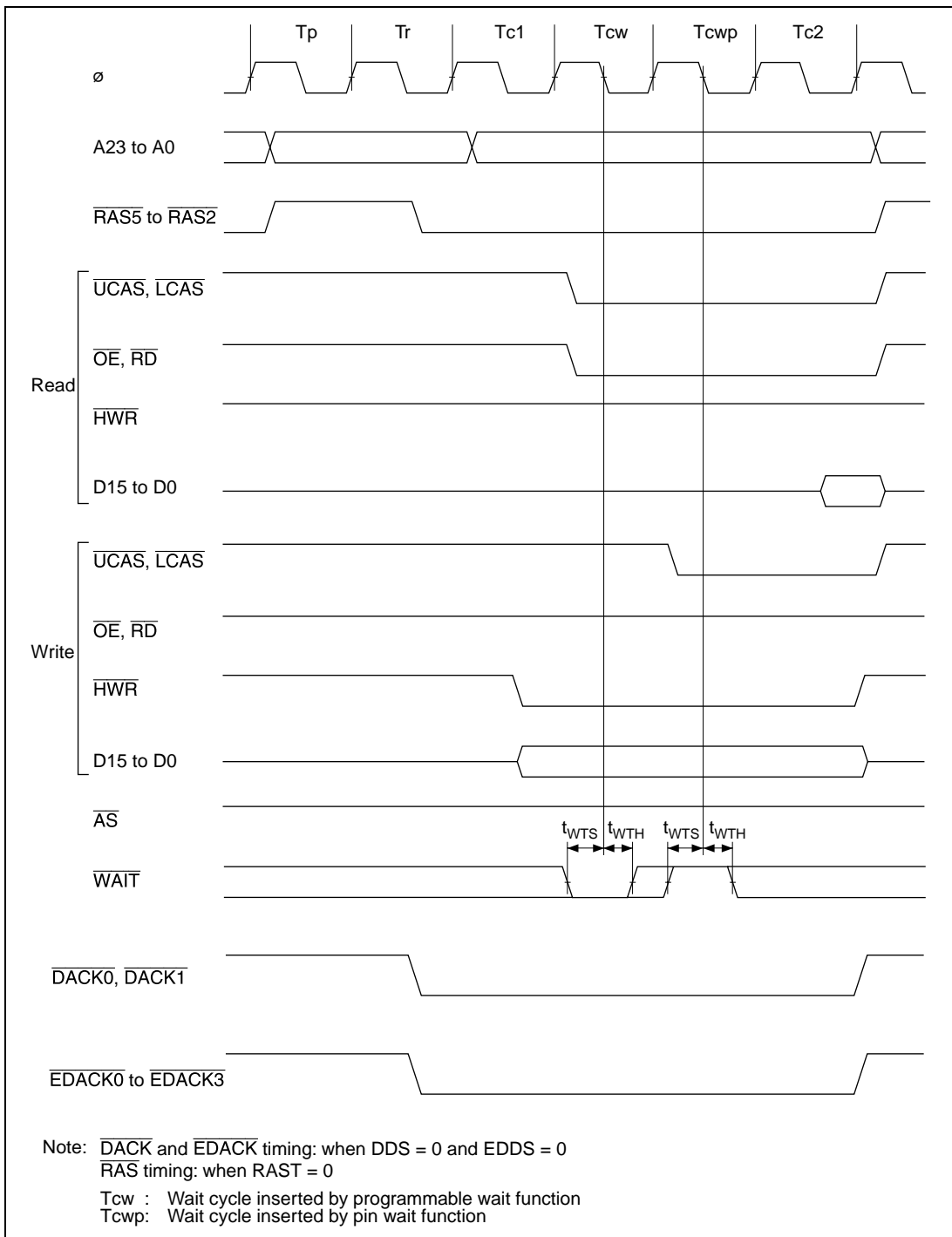
Figure 24.15 DRAM Access Timing: Two-State Access, One Wait
