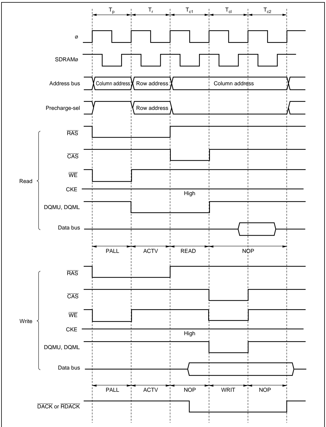
Figure 6.60 Example of \overline{\text{DACK}}/\text{EDACK} Output Timing when DDS = 1 or EDSS = 1
