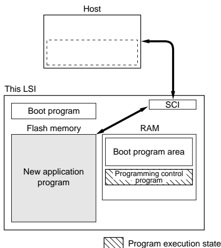
Figure 19.3 Boot Mode
