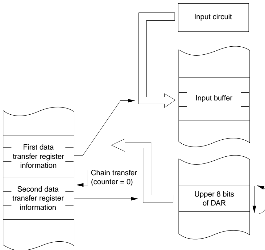
Figure 9.12 Chain Transfer when Counter = 0
