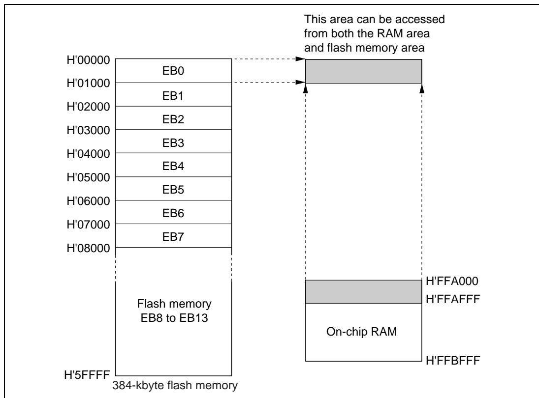
Figure 19.9 Example of RAM Overlap Operation
