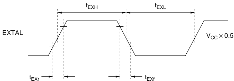
Figure 21.5 External Clock Input Timing
