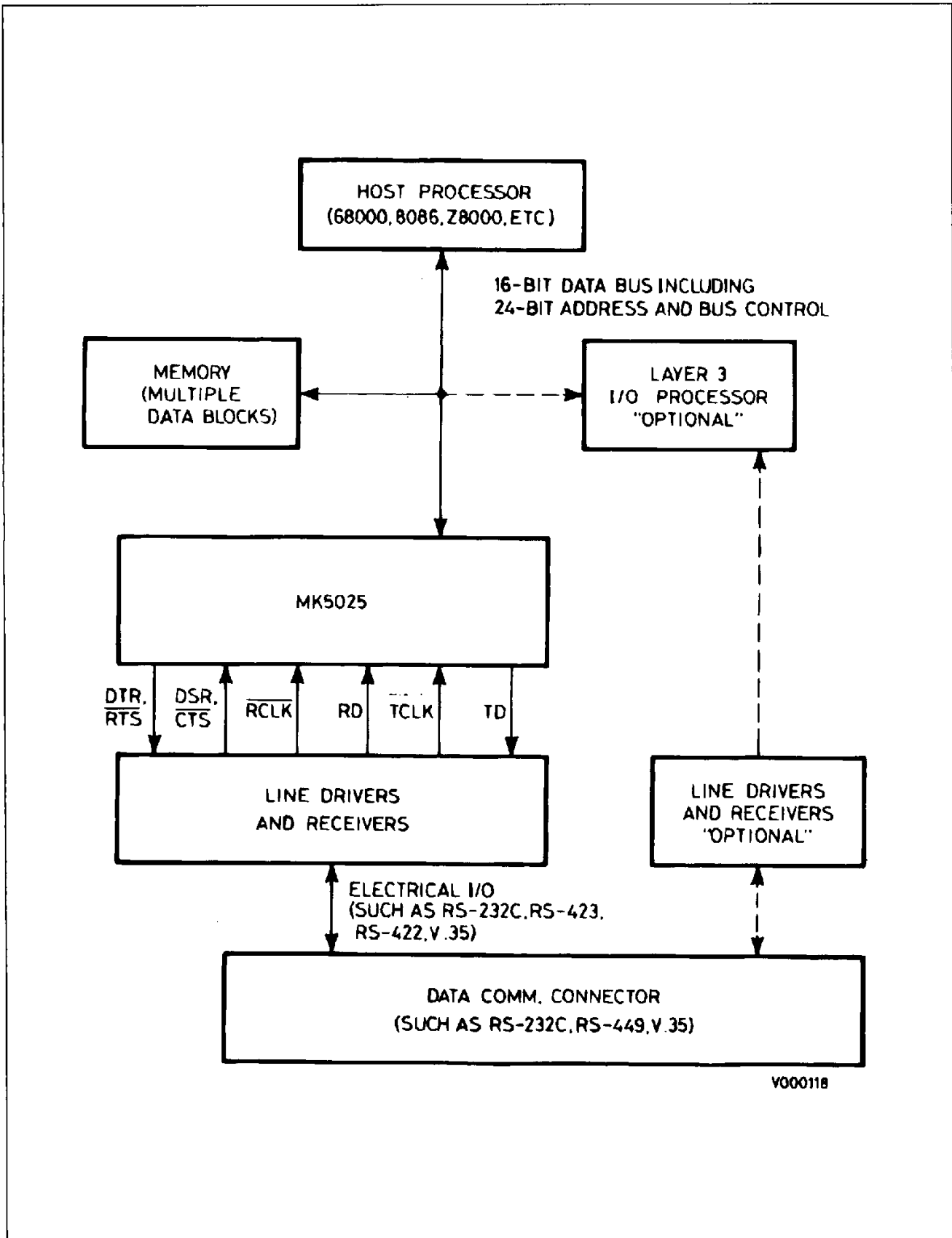
Figure 3 : Possible System Configuration for the MK5025.
