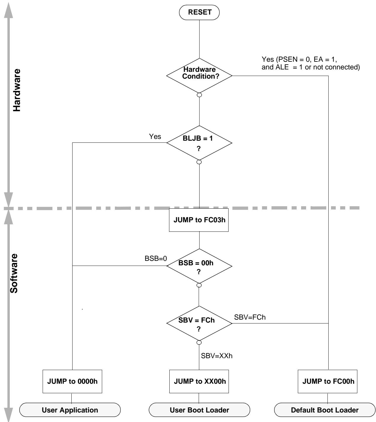
Figure 24. Bootloader Process
