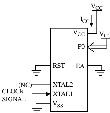
Figure 25. I CC Test Condition, Idle Mode
