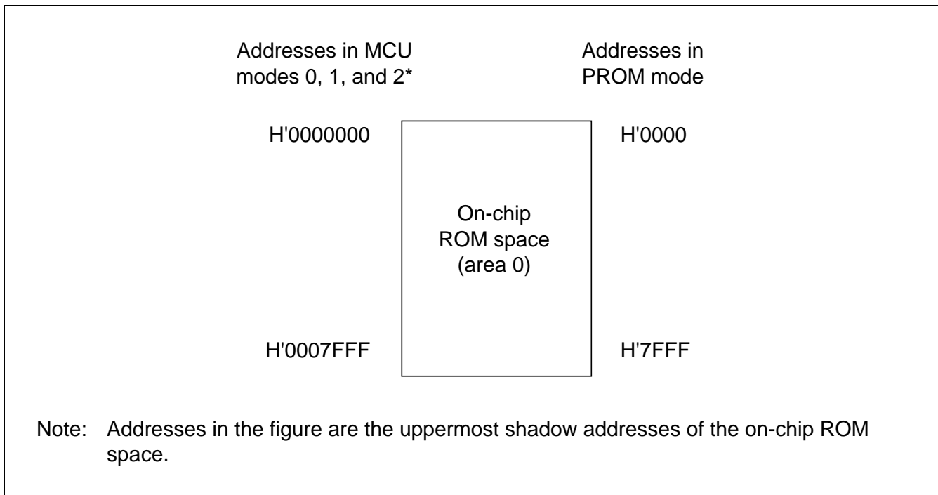
Figure 16.3 Memory Map of On-chip ROM
