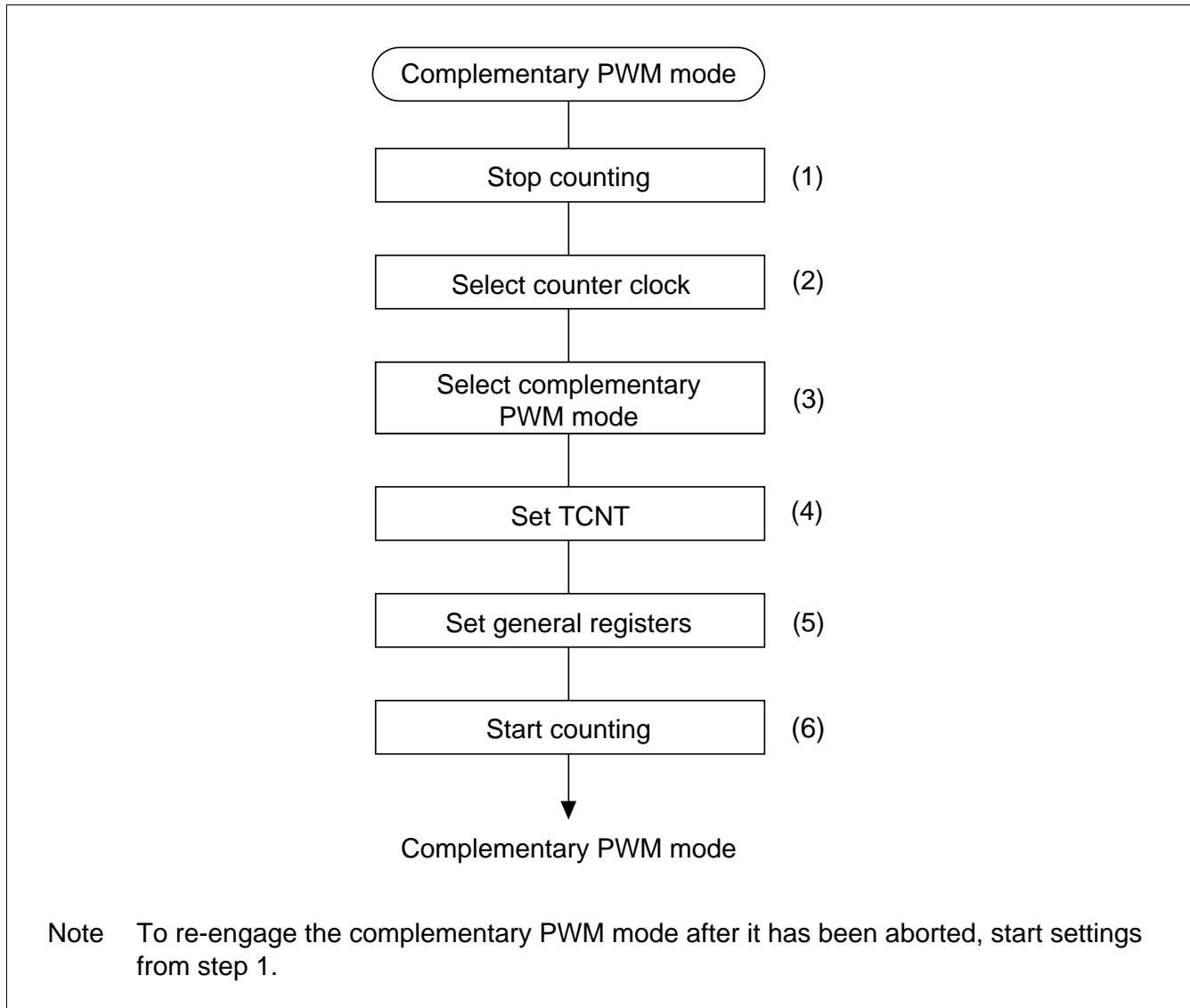
Figure 10.33 Procedure for Selecting the Complementary PWM Mode
