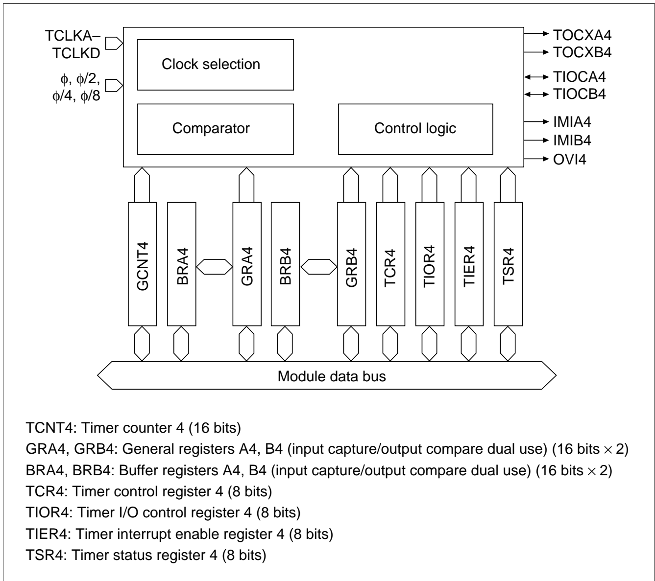
Figure 10.5 Channel 4 Block Diagram
