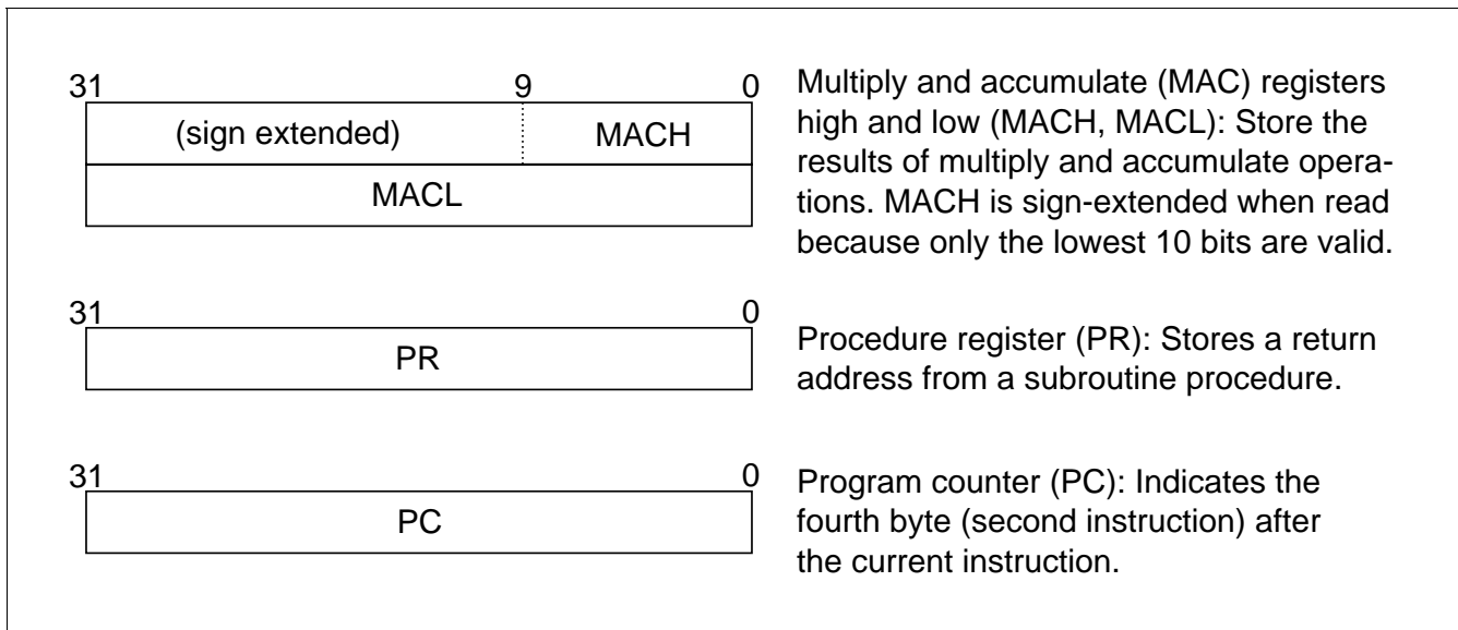
Figure 2.3 System Registers
