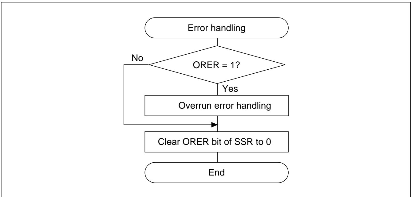
Figure 13.18 Sample Flowchart for Serial Receiving (cont)
