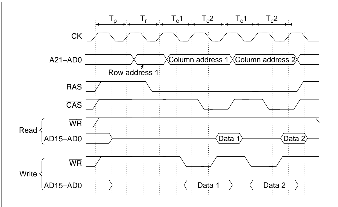
Figure 8.26 Long Pitch High-Speed Page Mode (Read/Write Cycle)
