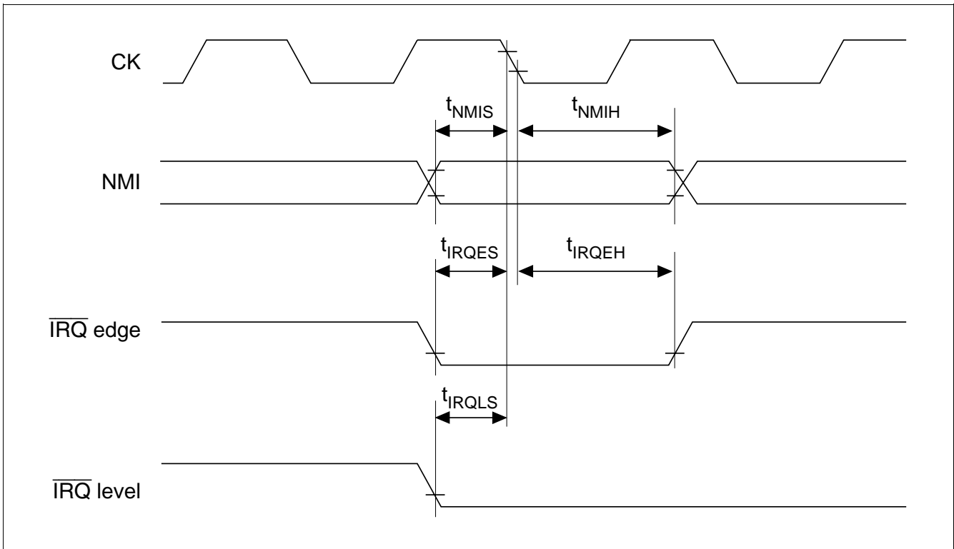
Figure 19.5 Interrupt Signal Input Timing
