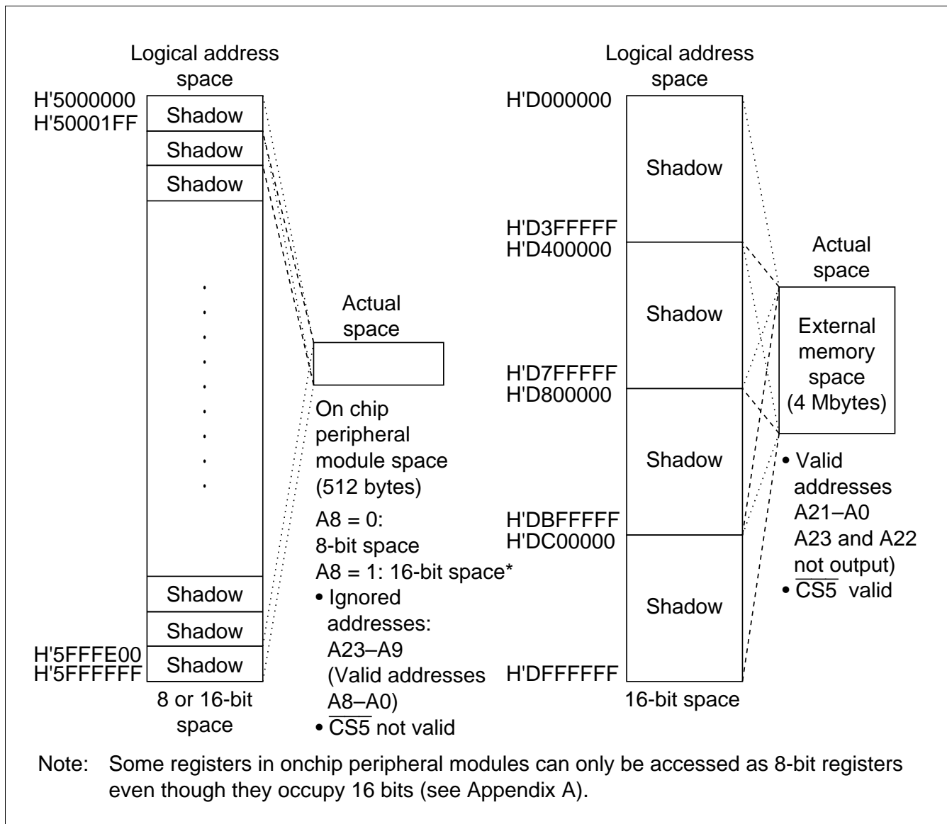
Figure 8.8 Memory Map of Area 5
