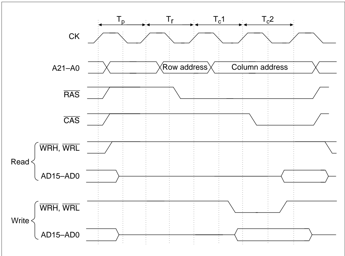
Figure 8.18 Long Pitch Access Timing
