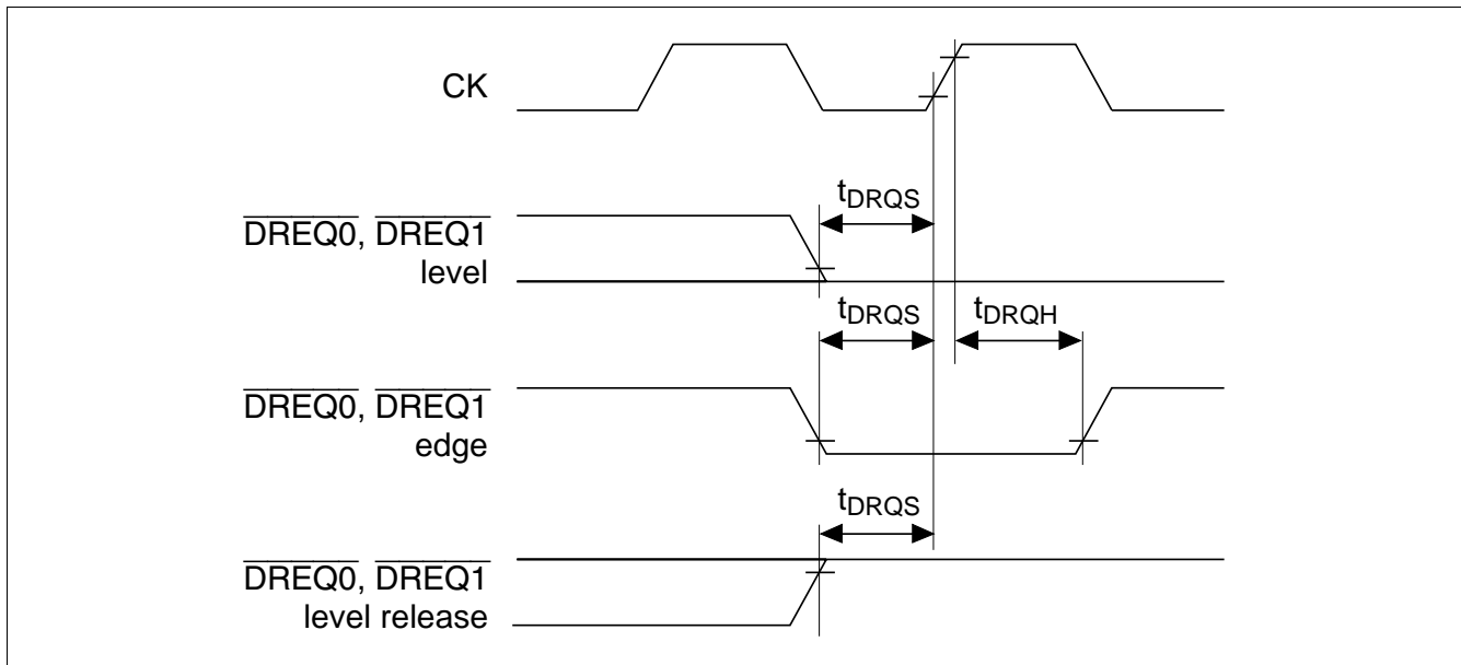
Figure 19.34 \overline{\text{DREQ0}}, \overline{\text{DREQ1}} Input Timing (1)
