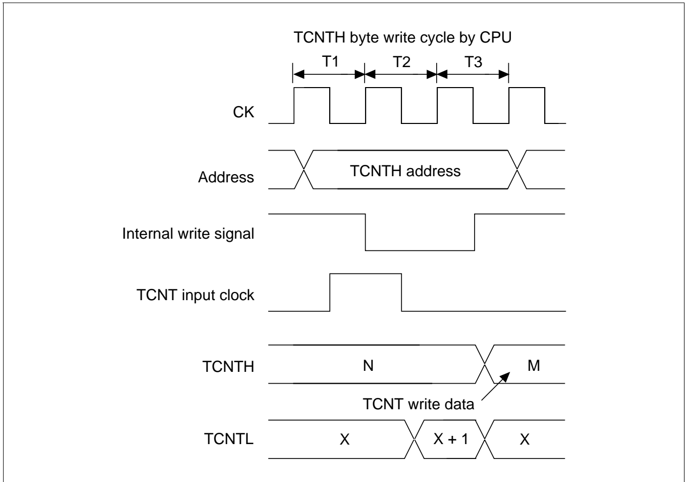
Figure 10.60 Contention between TCNT Byte Write and Increment
