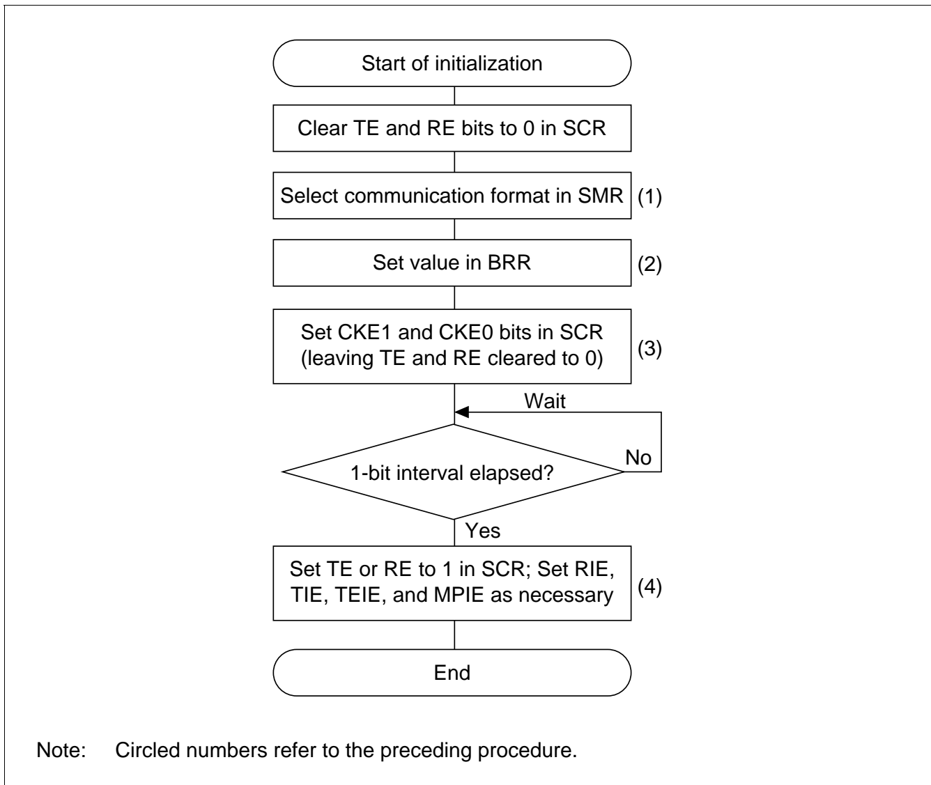
Figure 13.4 Sample Flowchart for SCI Initialization
