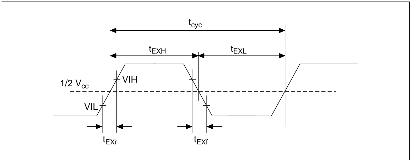
Figure 7.5 Input Clock Waveform
