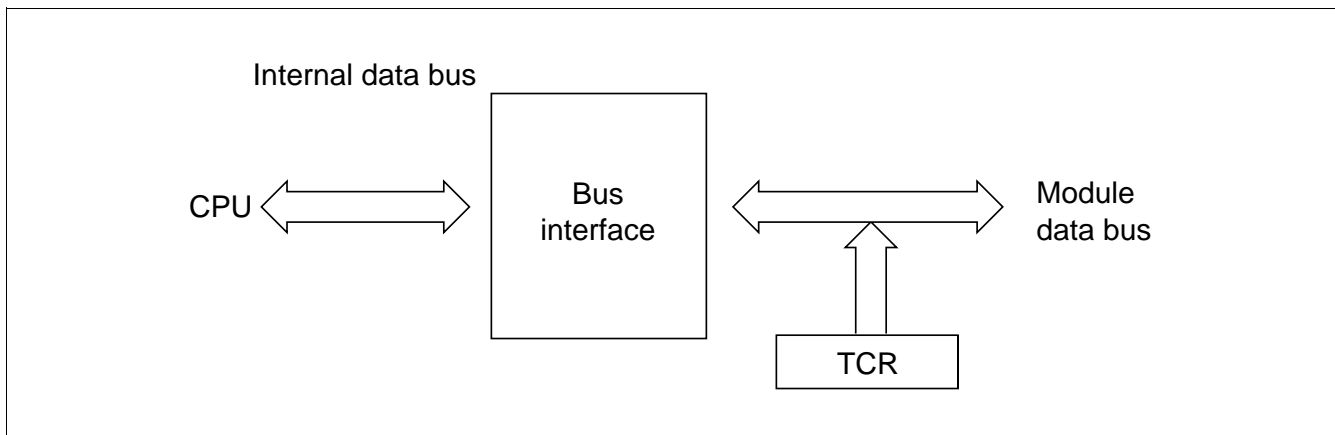
Figure 10.13 TCR Access (TCR-CPU )
