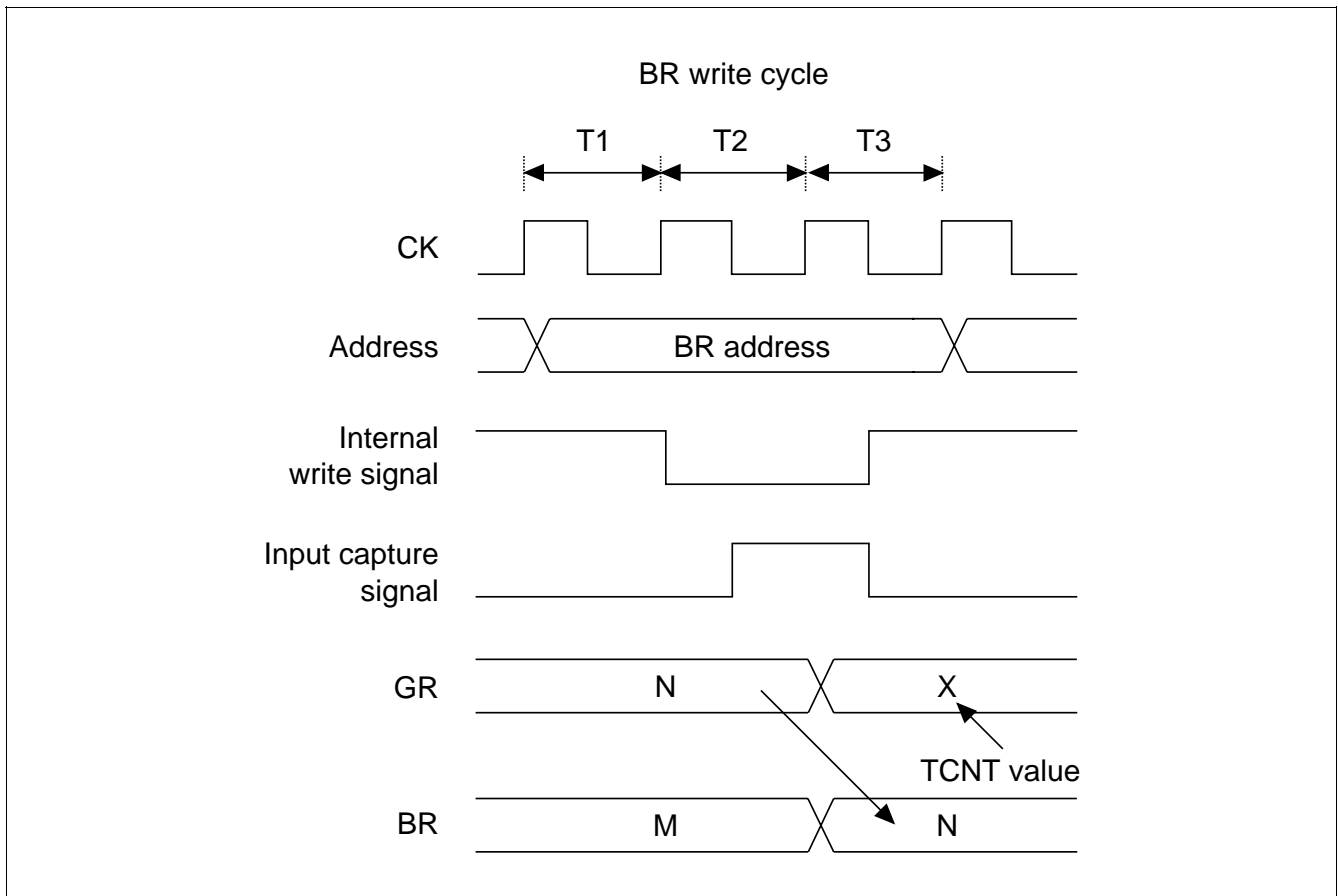
Figure 10.66 Contention Between BR Write and Input Capture
