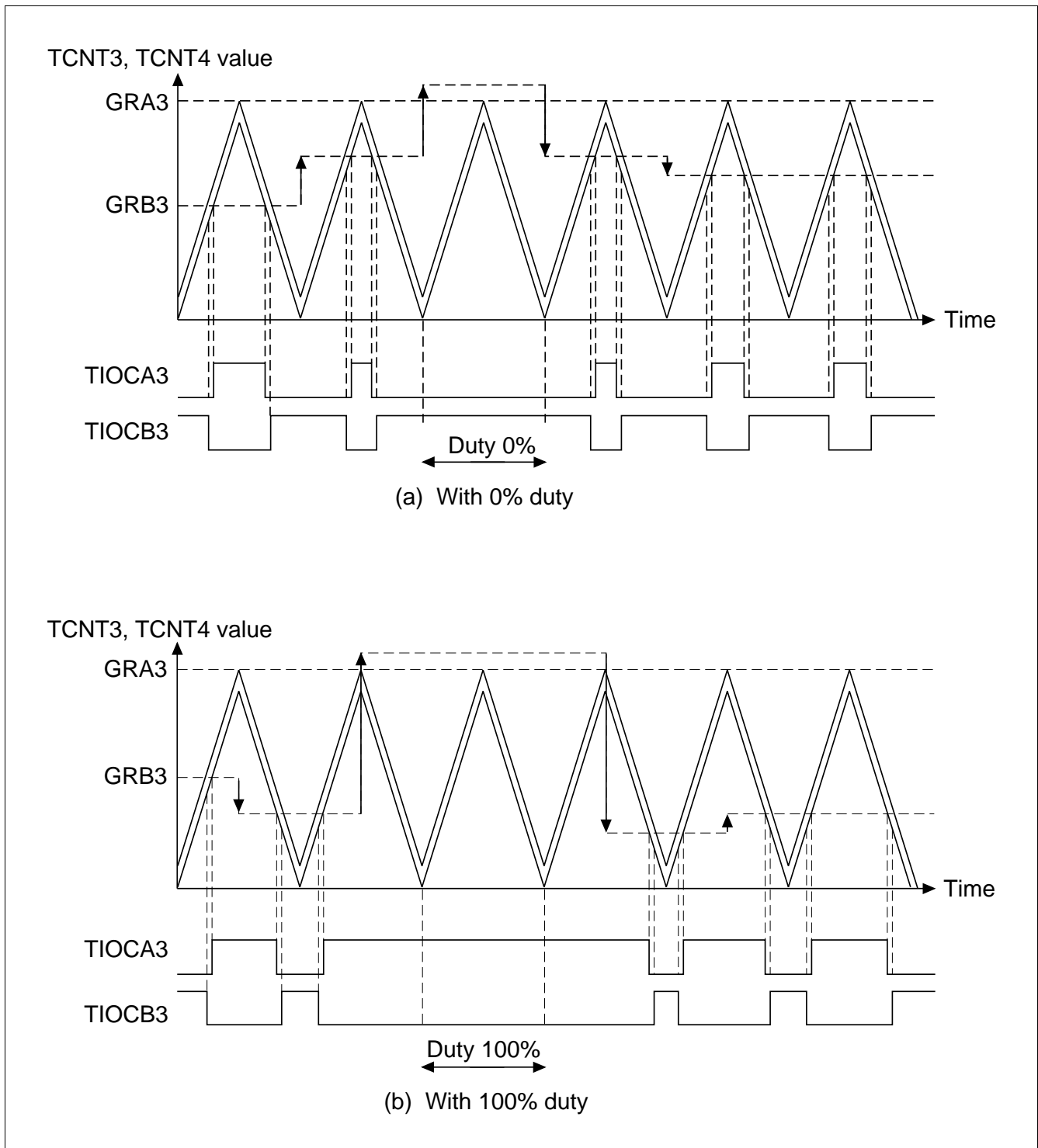
Figure 10.35 Complementary PWM Mode Operation Example 2
