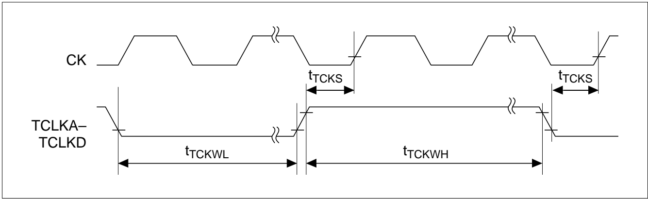
Figure 19.37 ITU Clock Input Timing
