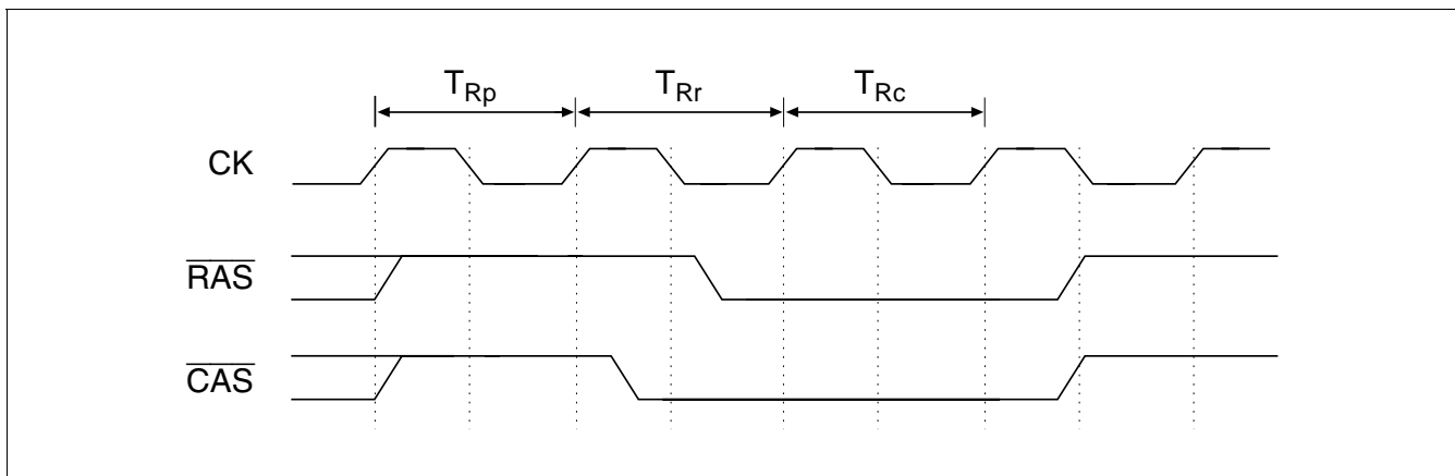
Figure 8.30 Output Timing for CAS-Before-RAS Refresh Signal
