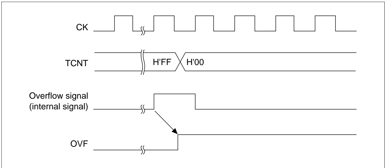
Figure 12.6 Timing of Setting the OVF
