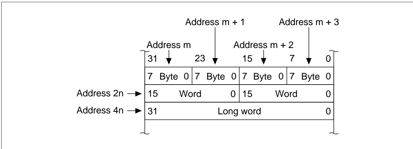
Figure 2.5 Data Format in Memory
