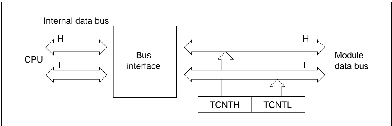
Figure 10.10 Accessing TCNT (TCNT–CPU (upper byte))
