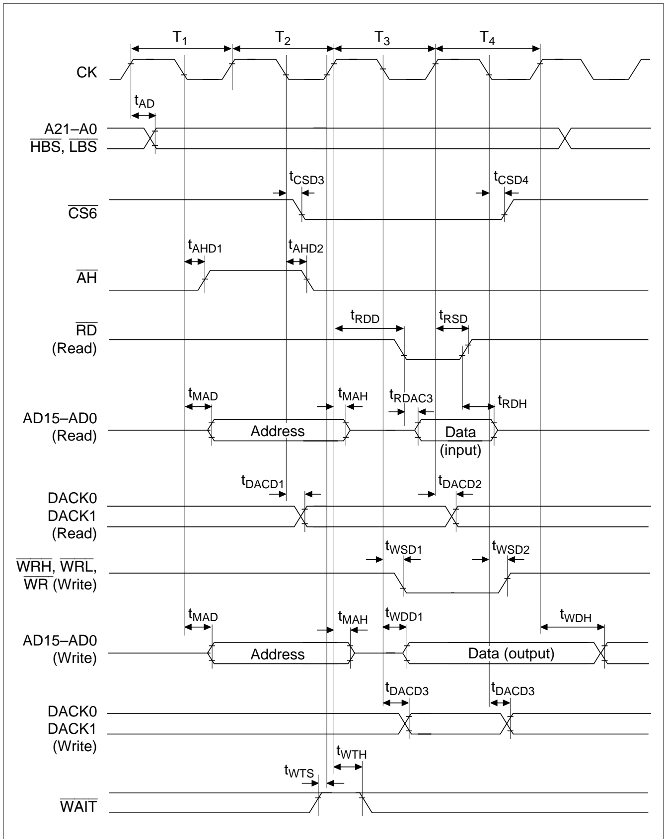
Figure 19.19 Address/Data Multiplex I/O Bus Cycle
