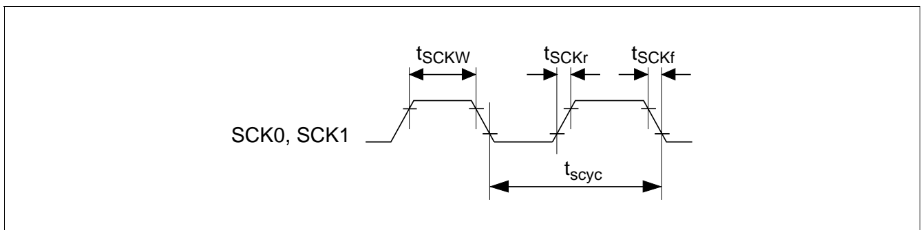
Figure 19.40 Input Clock Timing
