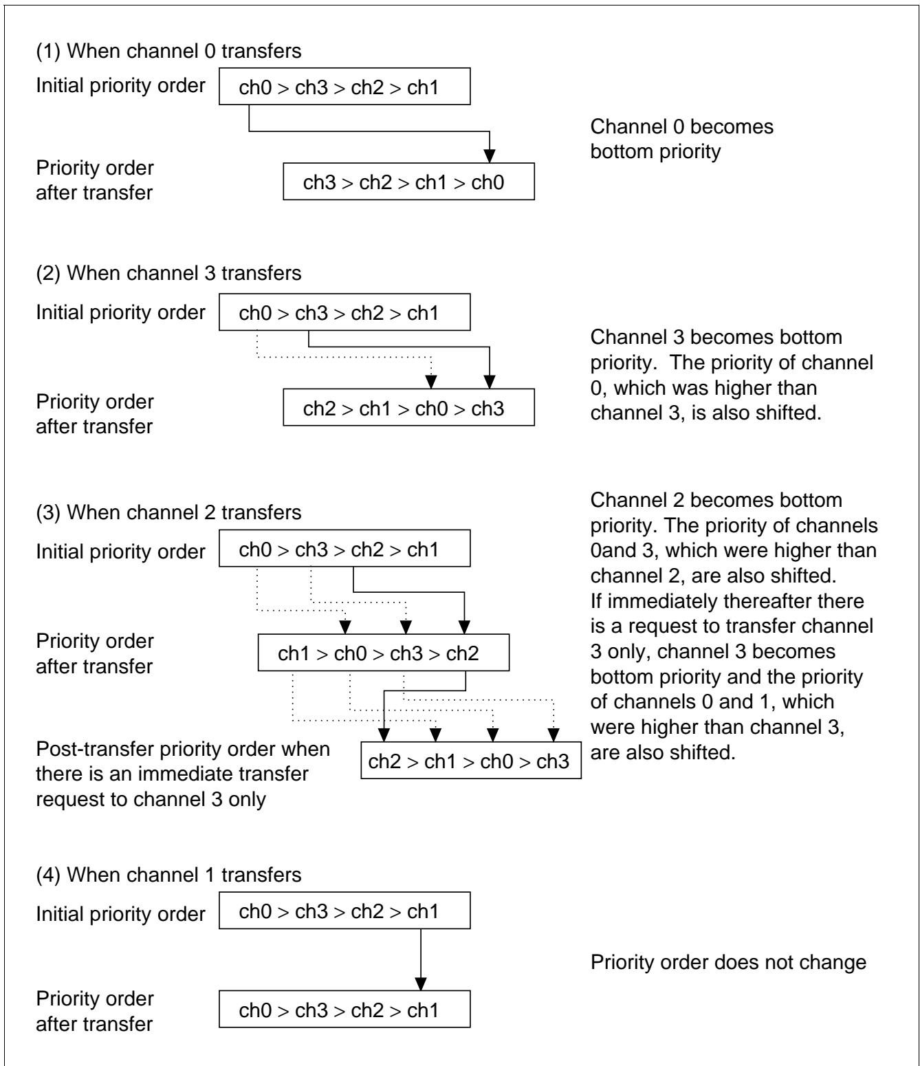
Figure 9.3 Round-Robin Mode
