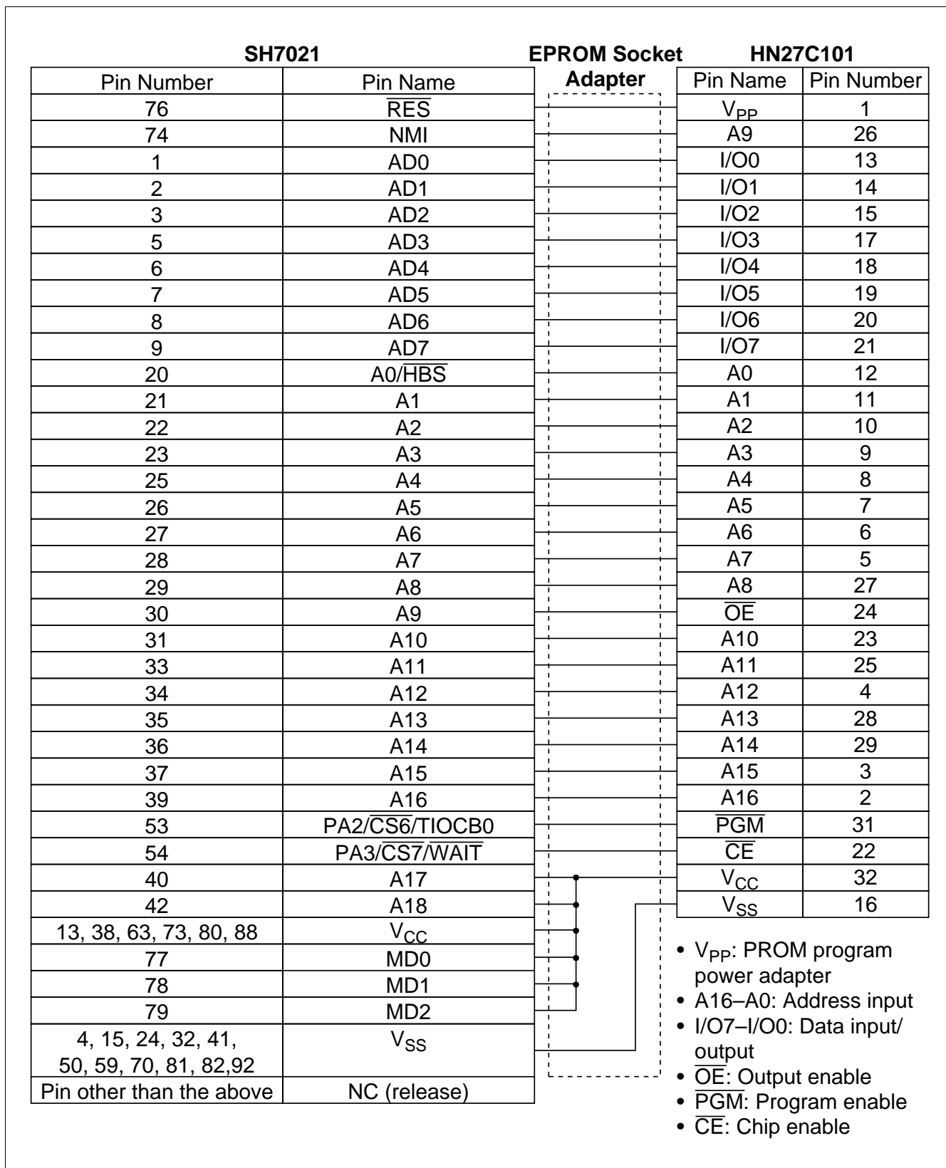
Figure 16.2 Correspondence Between SH7021 Pins and HN27C101 Pins
