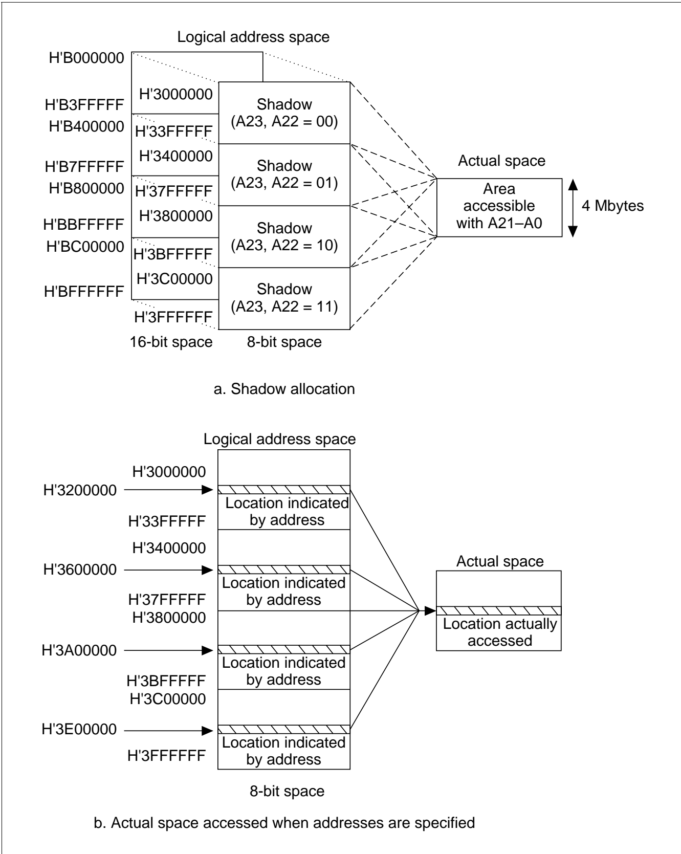
Figure 8.4 Shadows
