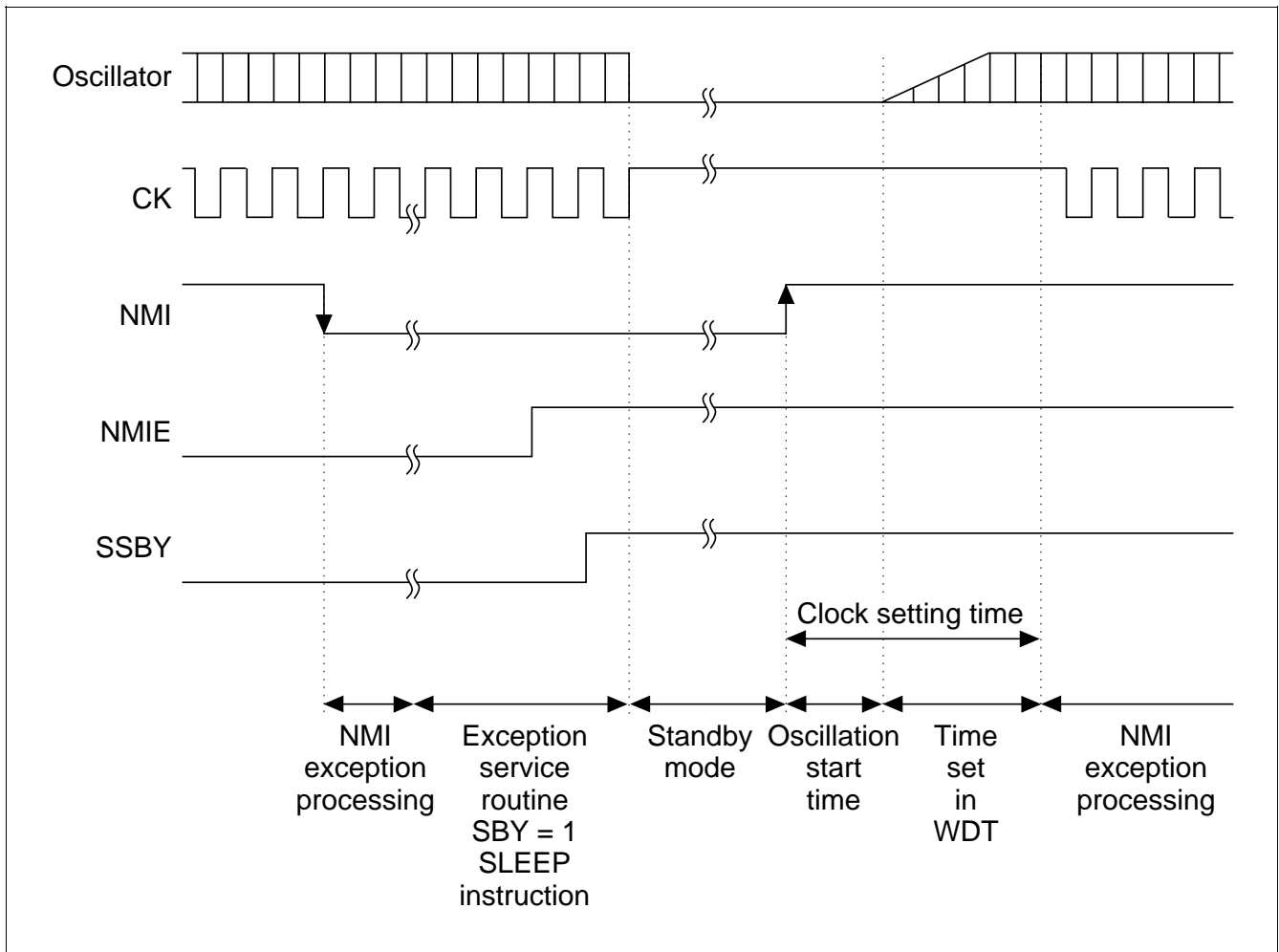
Figure 18.1 NMI Timing for the Standby Mode (Example)
