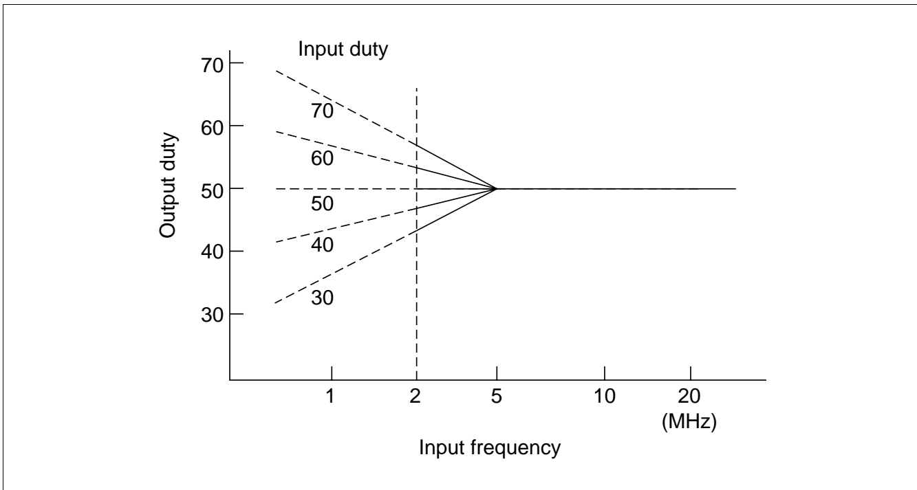
Figure 7.7 Duty Cycle Correction Circuit Standard Characteristics
