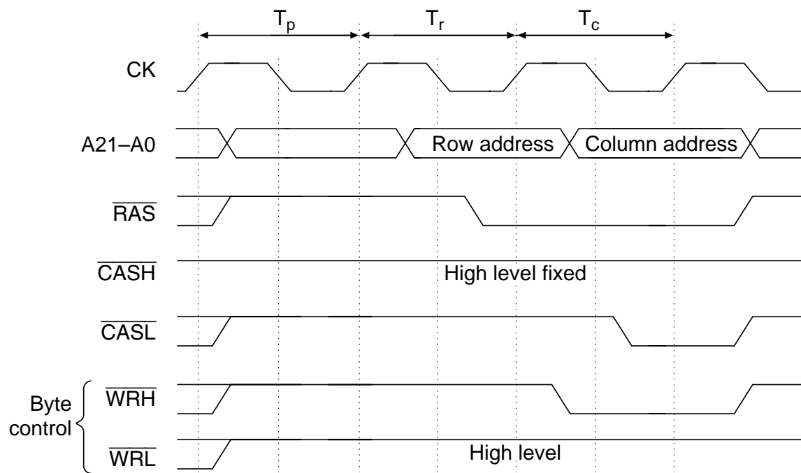
(a) Dual WE signals (CW2 = 1)
