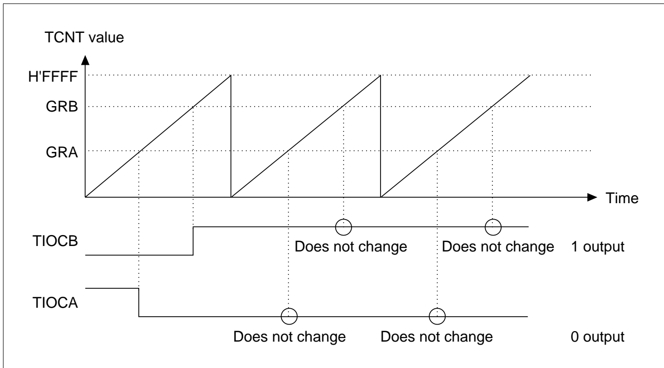
Figure 10.20 Example of 0 Output/1 Output
