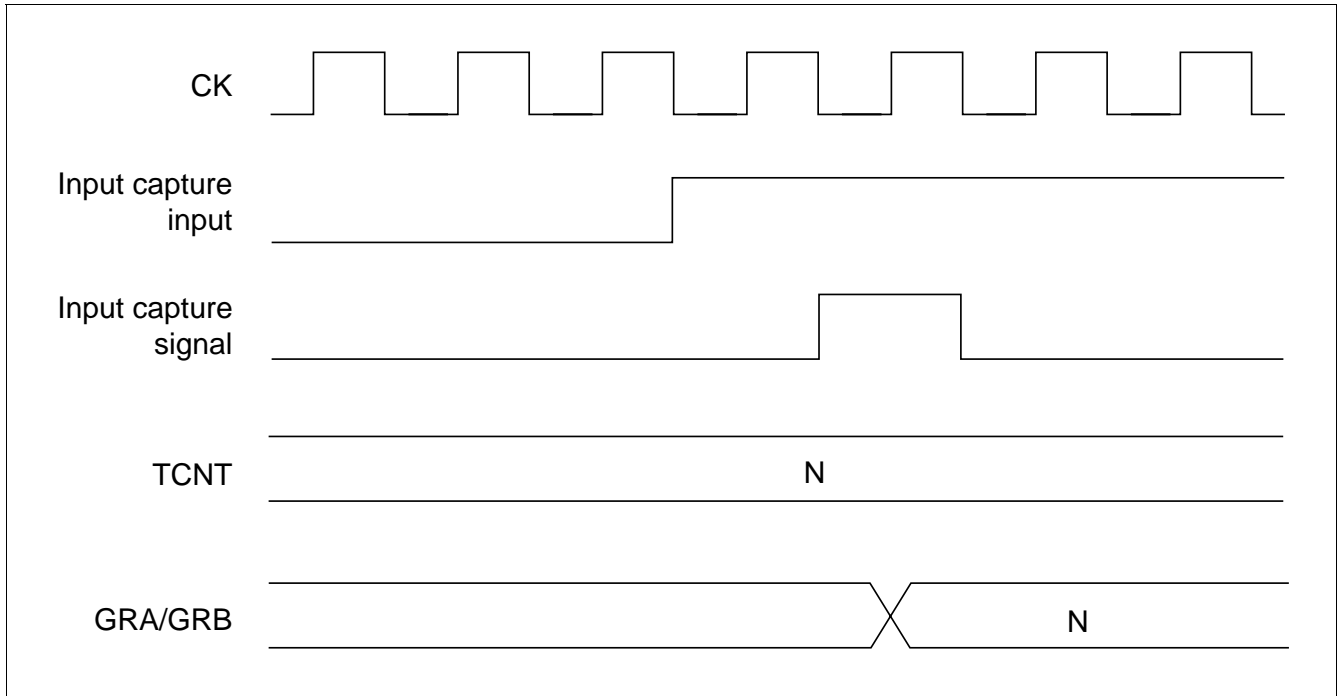
Figure 10.25 Input Capture Signal Timing
