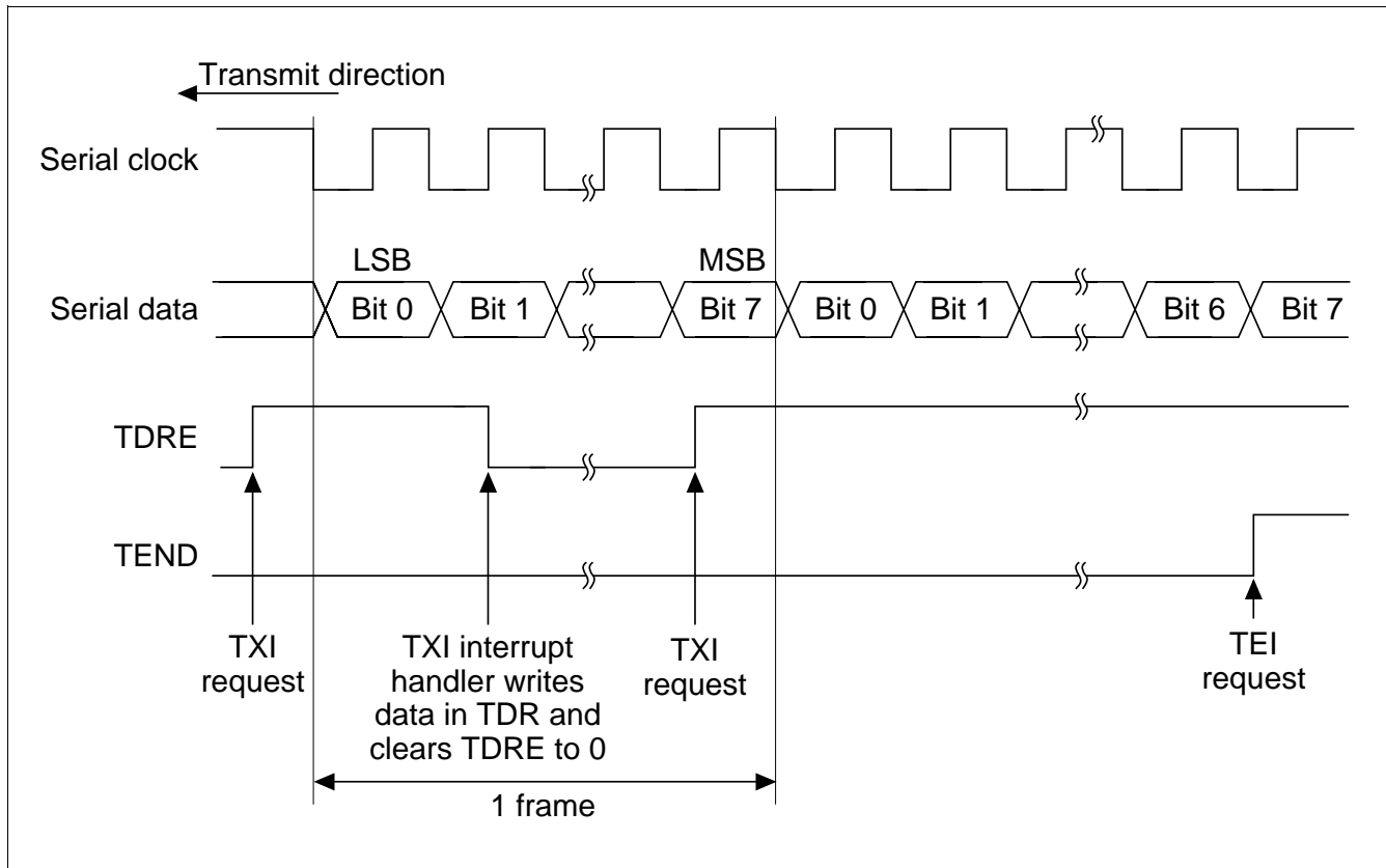
Figure 13.15 Example of SCI Transmit Operation
