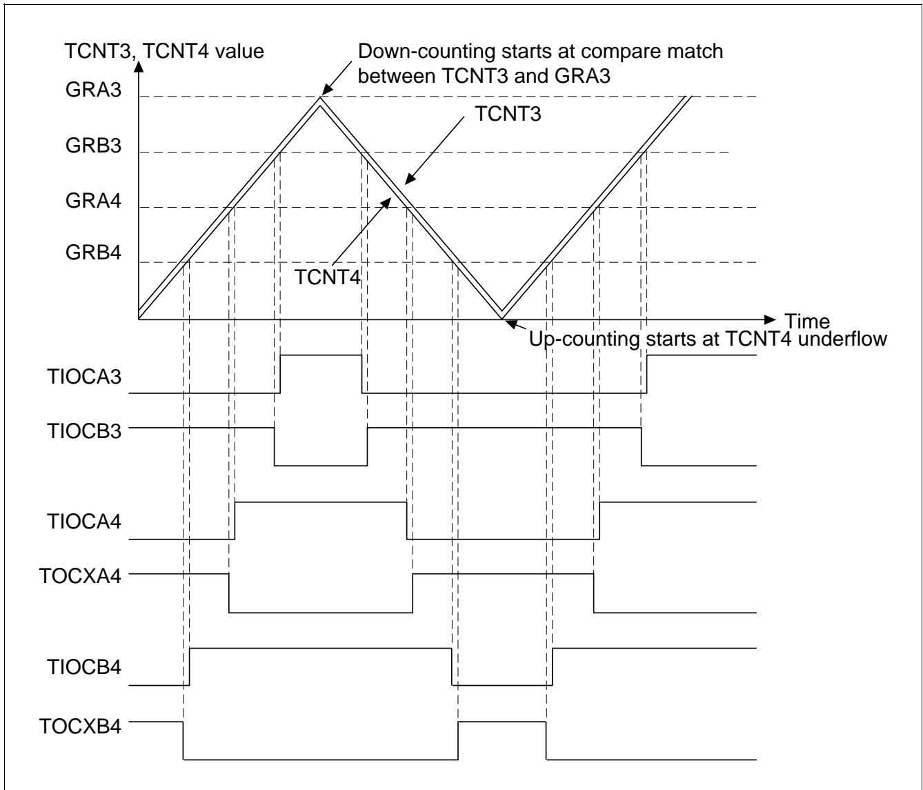
Figure 10.34 Complementary PWM Mode Operation Example 1
