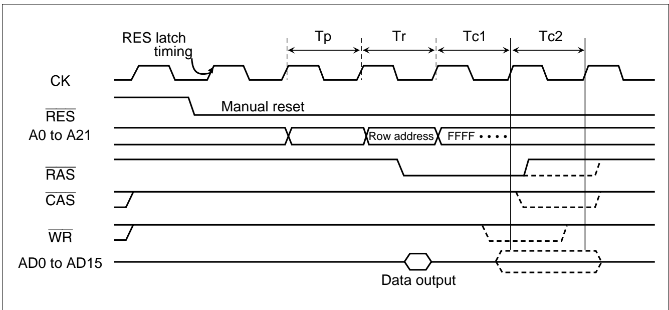
Figure 8.39 Long - pitch Mode Write (2)
