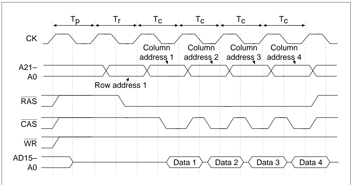
Figure 8.23 Short Pitch High-Speed Page Mode (Read Cycle)
