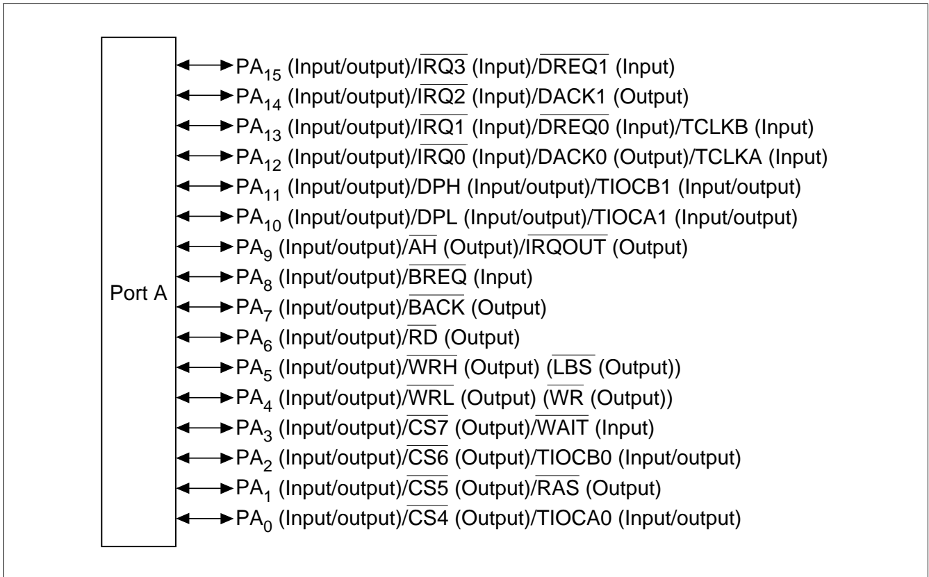
Figure 15.1 Port A Configuration
