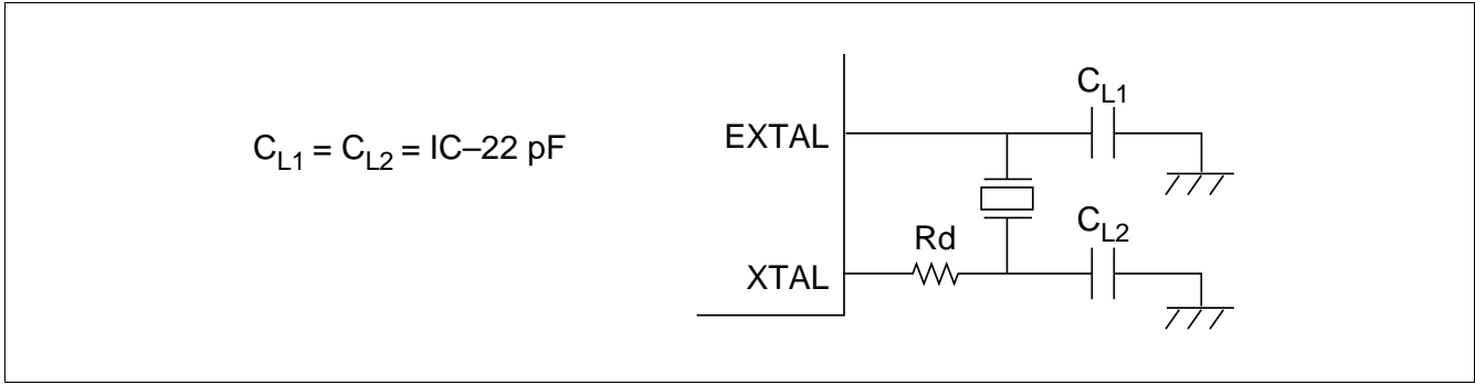
Figure 7.2 Connection of the Crystal Resonator (Example)
