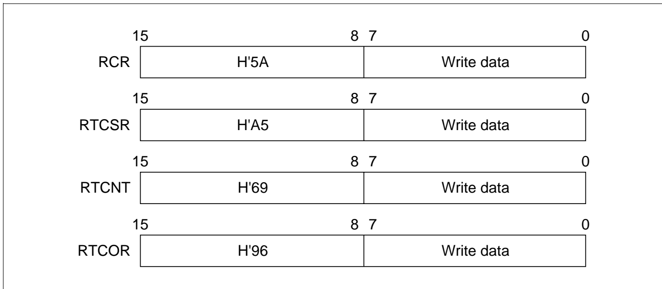
Figure 8.2 Writing to RCR, RTCSR, RTCNT, and RTCOR
