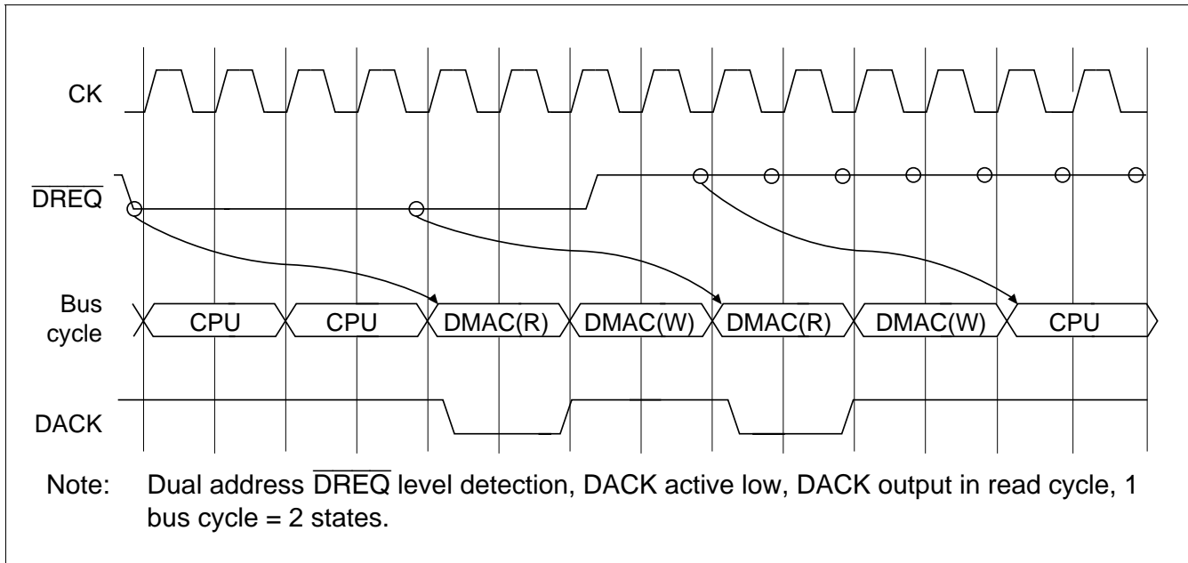
Figure 9.24 \overline{\text{DREQ}} Pin Sampling Timing in Burst Mode
