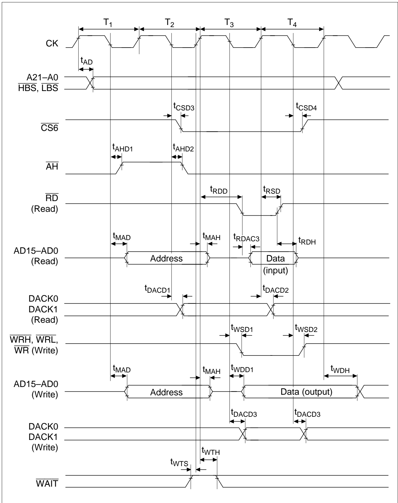
Figure 19.32 Address/Data Multiplex I/O Bus Cycle
