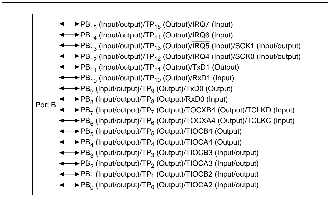
Figure 15.2 Port B Configuration
