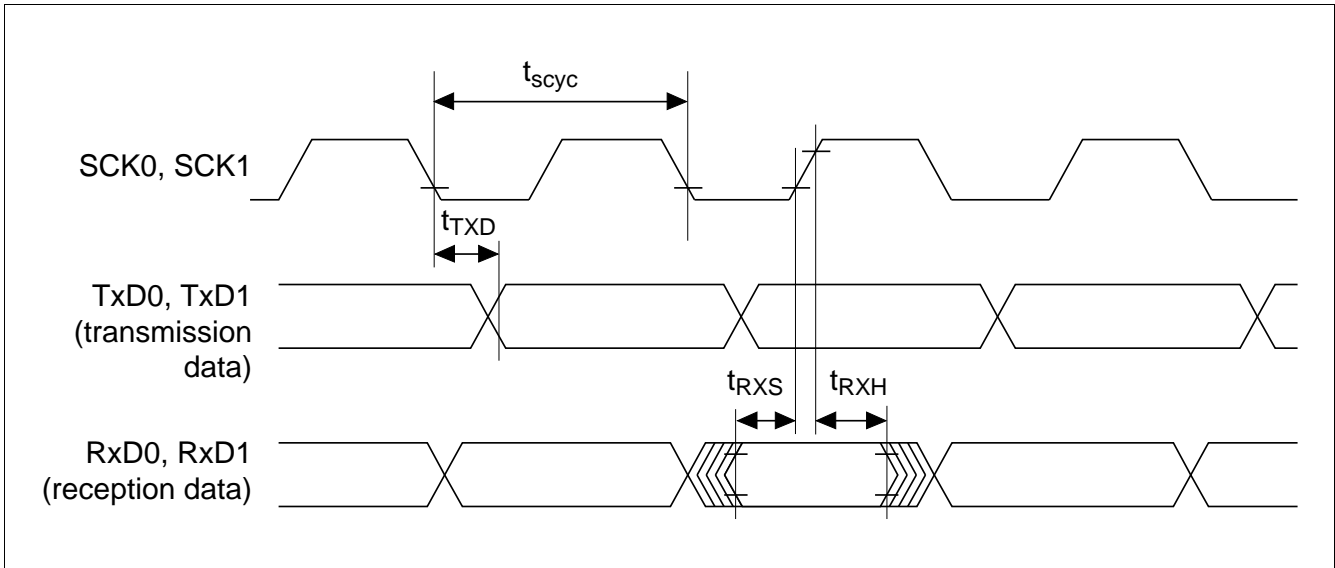
Figure 19.41 SCI I/O Timing (Clocked Synchronization Mode)
