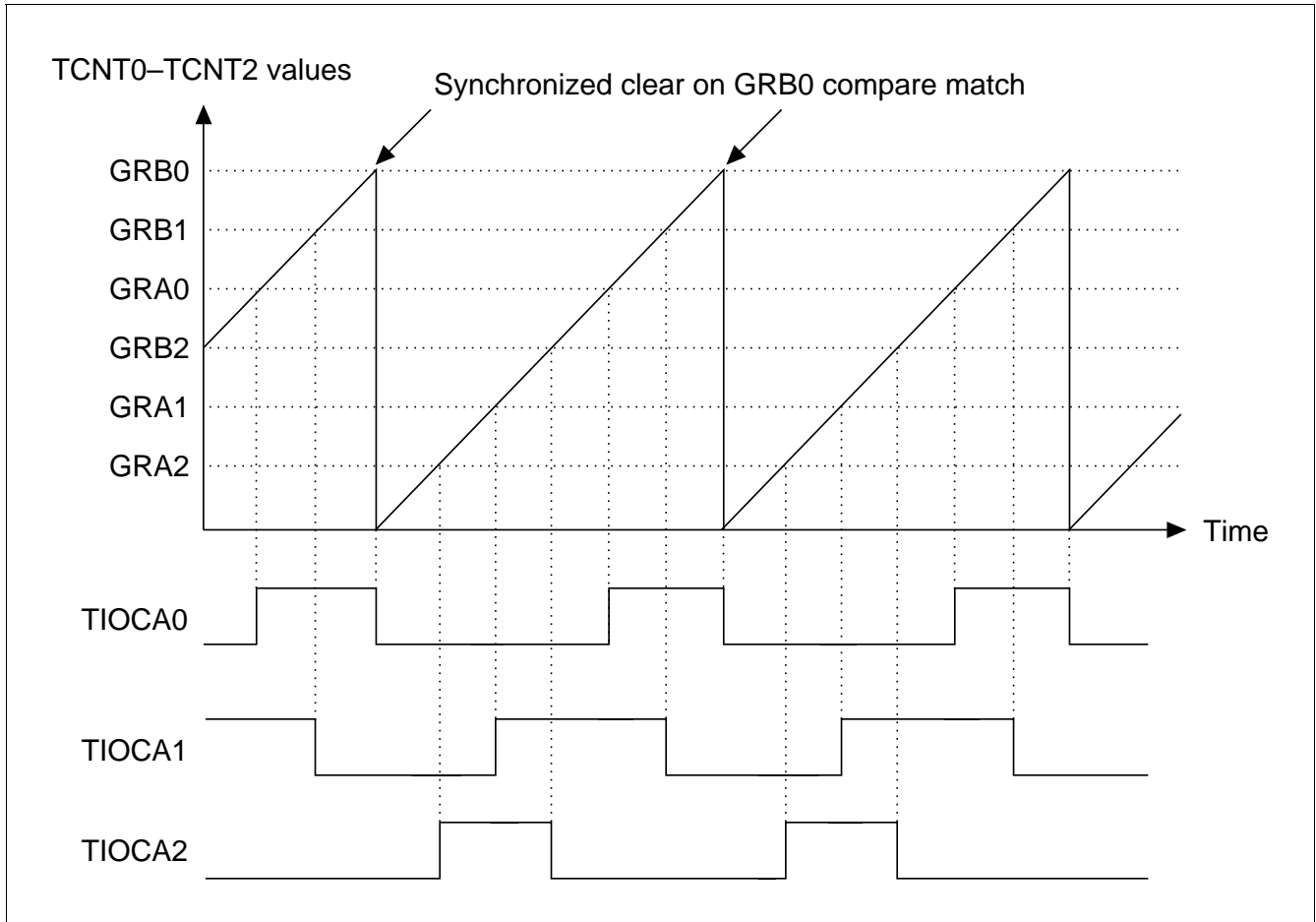
Figure 10.27 Synchronized Operation Example
