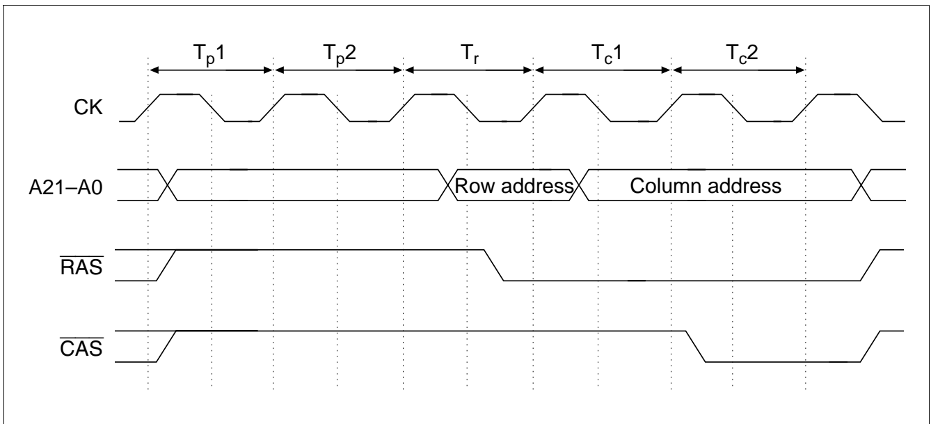
Figure 8.19 Precharge Timing (Long Pitch)
