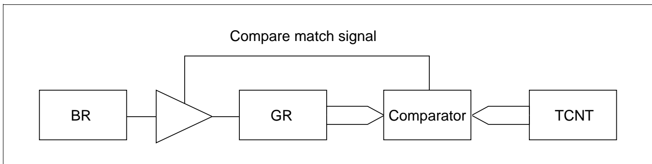
Figure 10.45 Compare Match Buffer Operation
