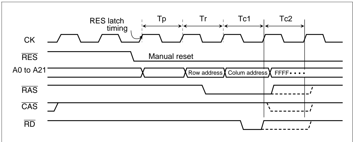
Figure 8.40 Long - pitch Mode Read (1)
