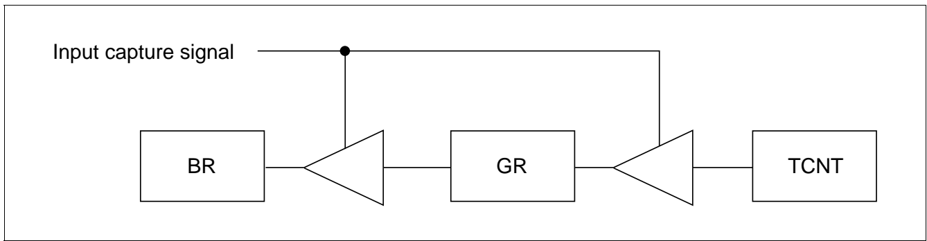
Figure 10.46 Input Capture Buffer Operation
