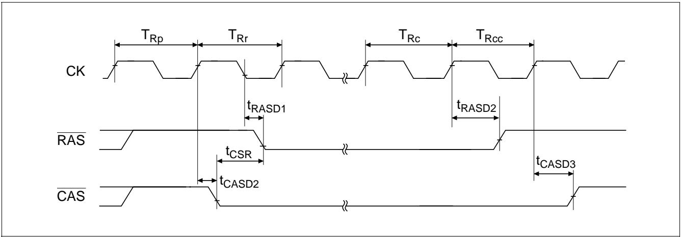
Figure 19.31 Self Refresh
