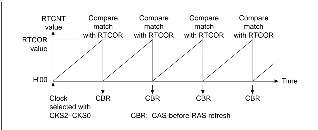
Figure 8.29 Refresh Timer Counter (RTCNT) Operation
