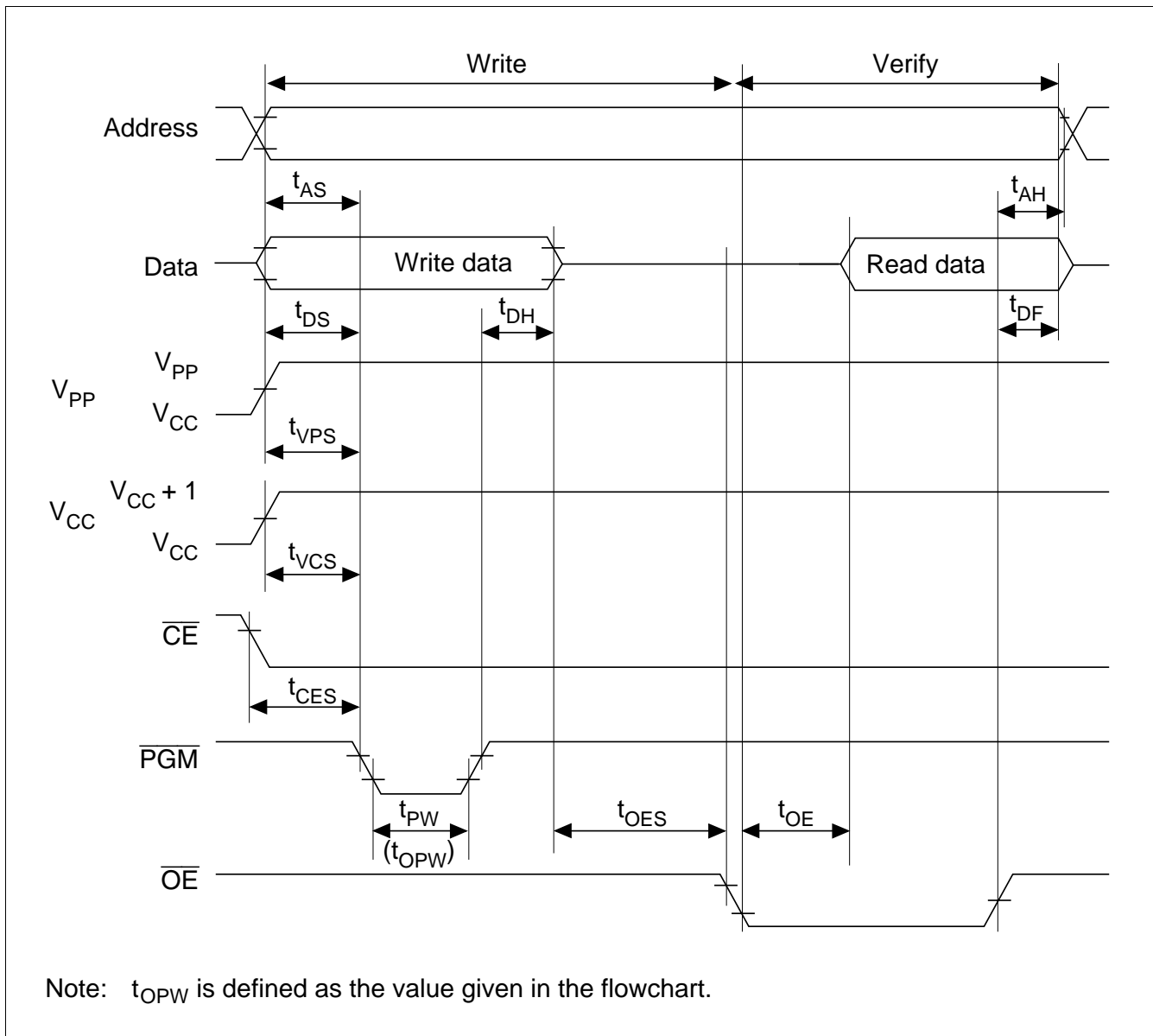
Figure 16.5 Write/Verify Timing
