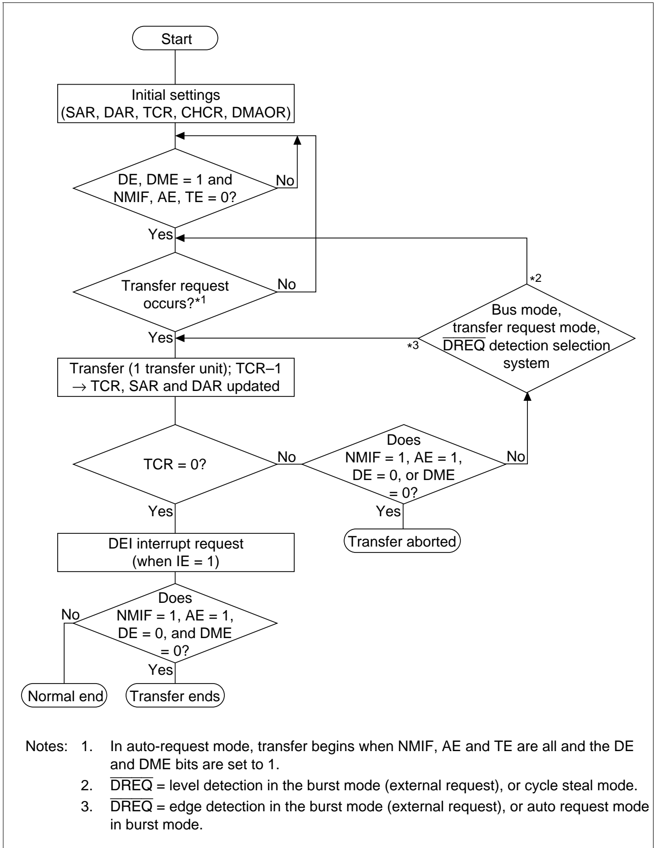
Figure 9.2 DMA Transfer Flowchart
