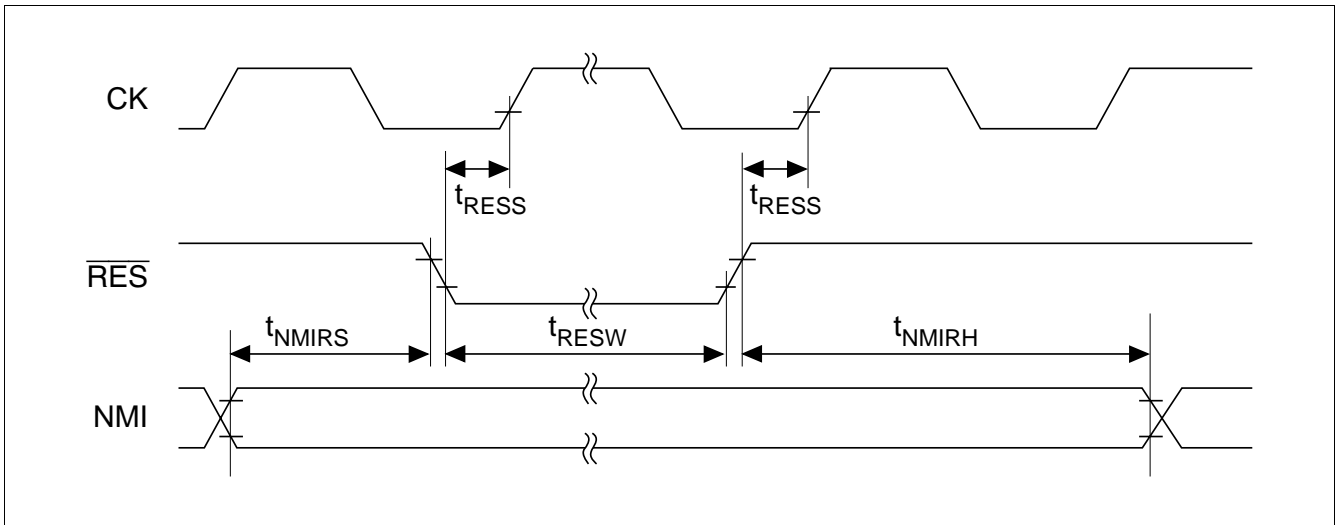
Figure 19.4 Reset Input Timing
