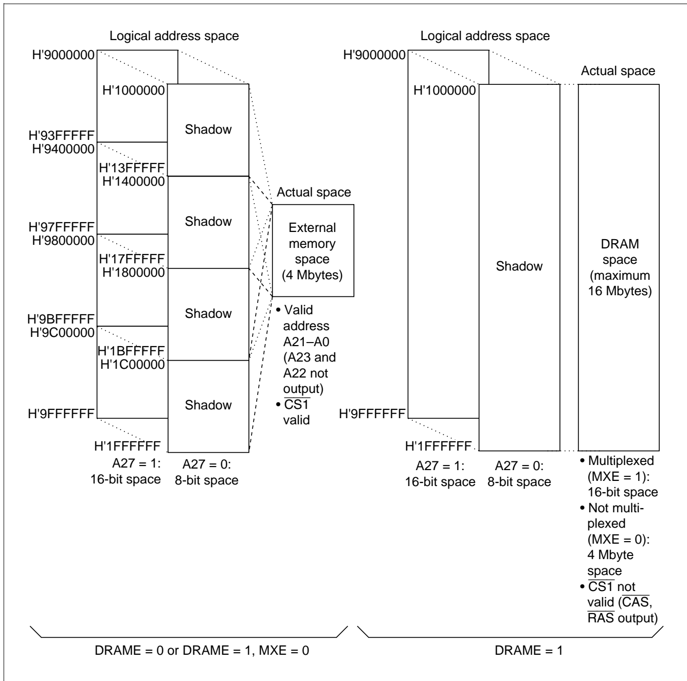
Figure 8.6 Memory Map of Area 1
