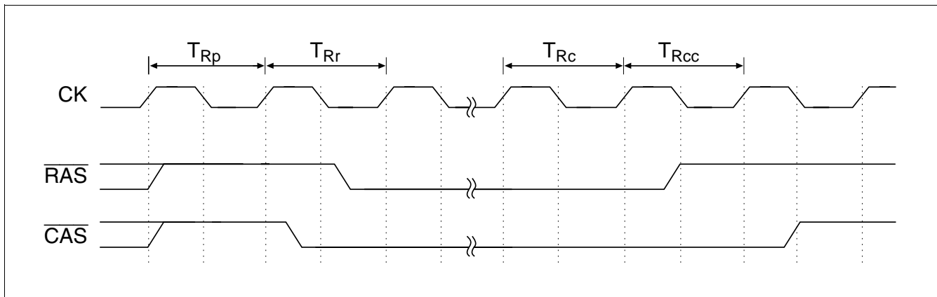
Figure 8.31 Output Timing of Self-Refresh Signal
