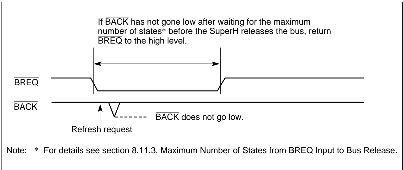
Figure 8.37 \overline{\text{BACK}} Operation in Response to Refresh Request (2)
