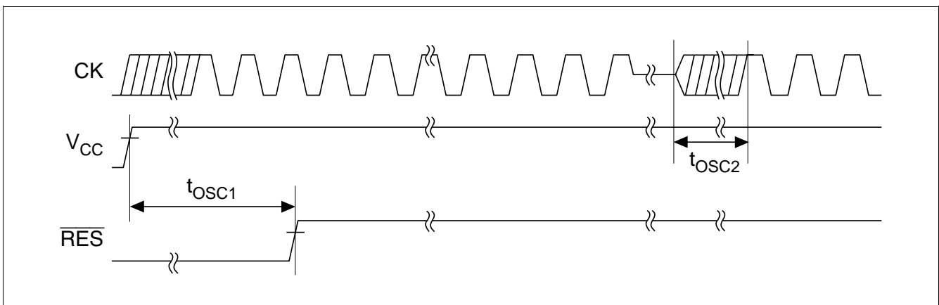
Figure 19.3 Oscillation Settling Time
