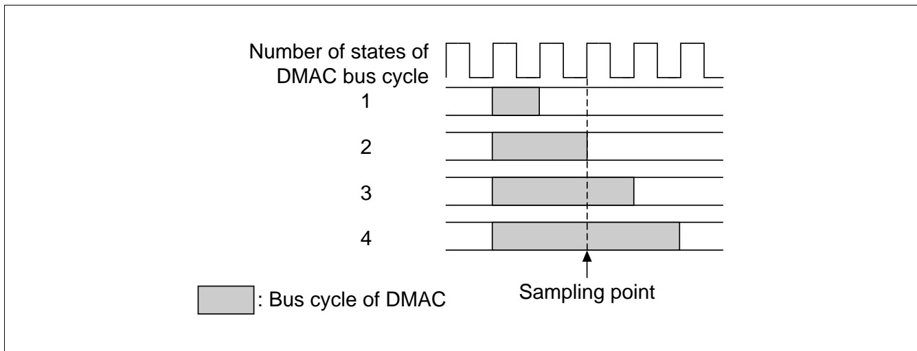
Figure 9.16 Sampling Points of DREQ
