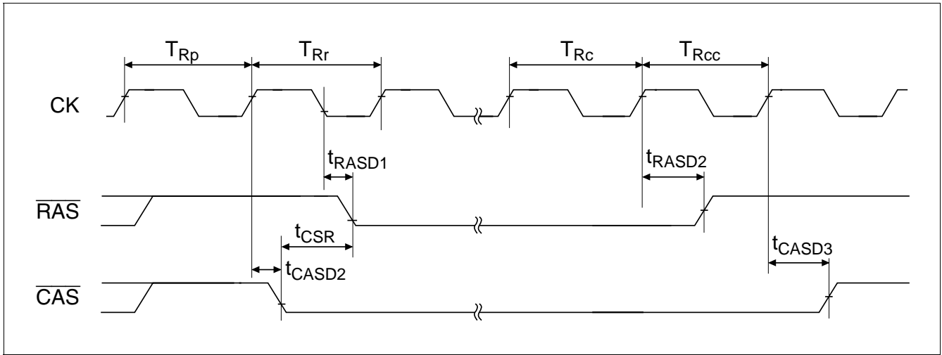
Figure 19.18 Self Refresh
