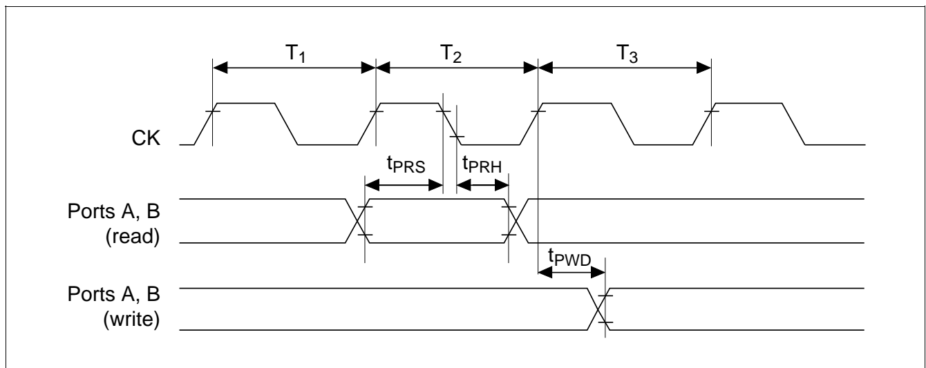
Figure 19.38 Programmable Timing Pattern Controller Output Timing
