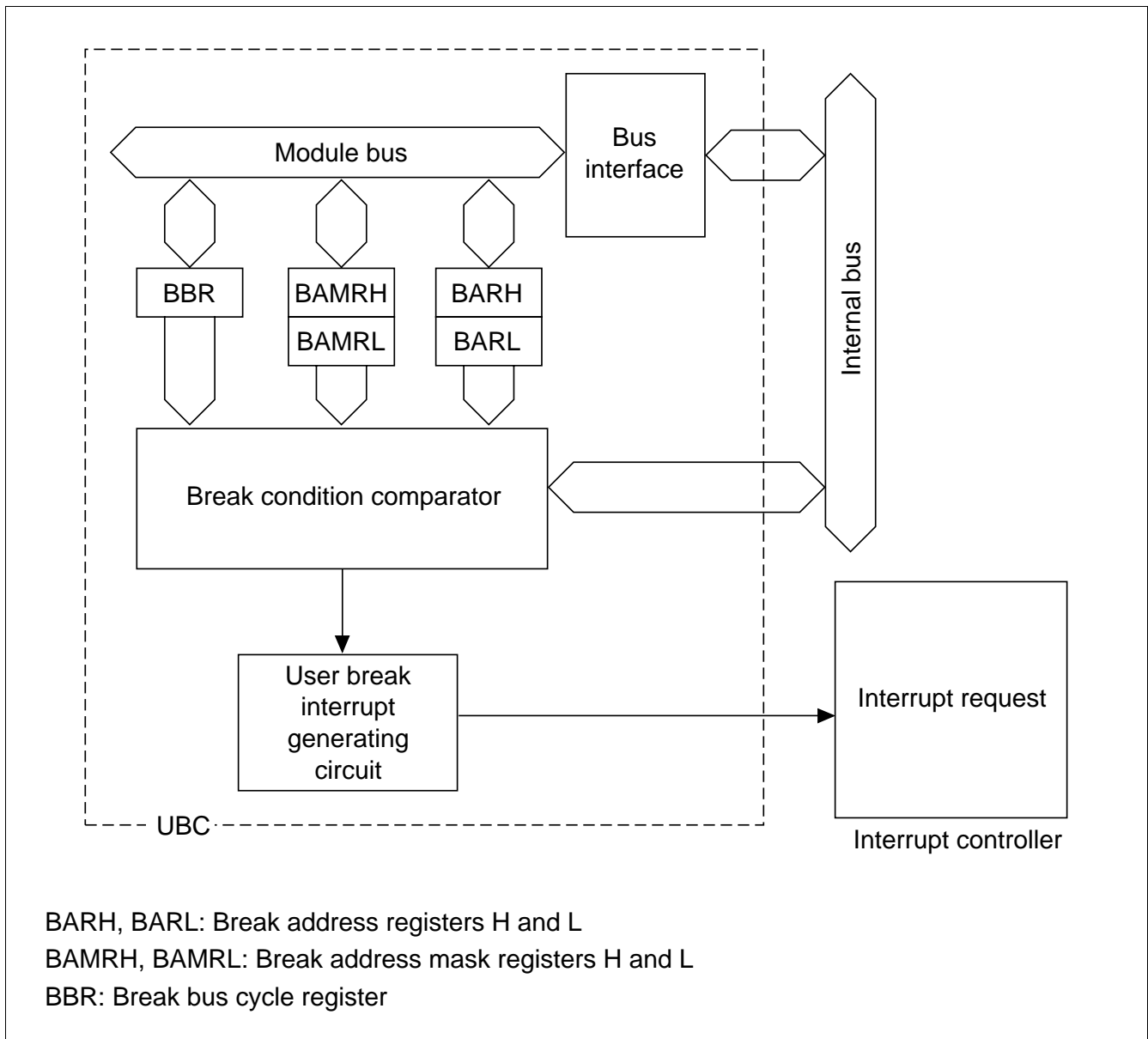
Figure 6.1 Block Diagram of the User Break Controller
