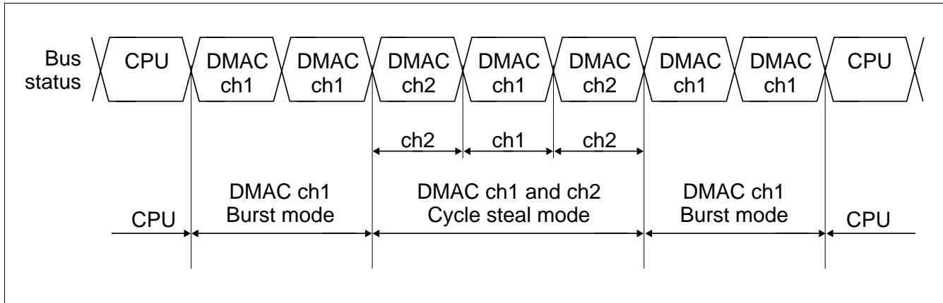
Figure 9.12 Bus Handling when Multiple Channels Are Operating
