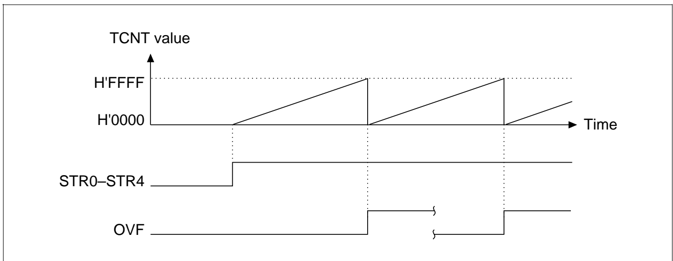
Figure 10.15 Free-Running Counter Operation
