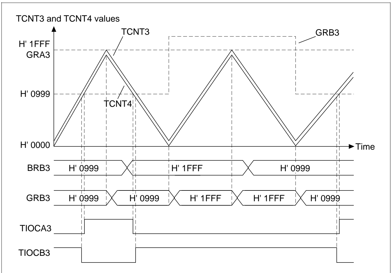
Figure 10.52 Buffer Operation 4 (Complementary PWM Mode)
