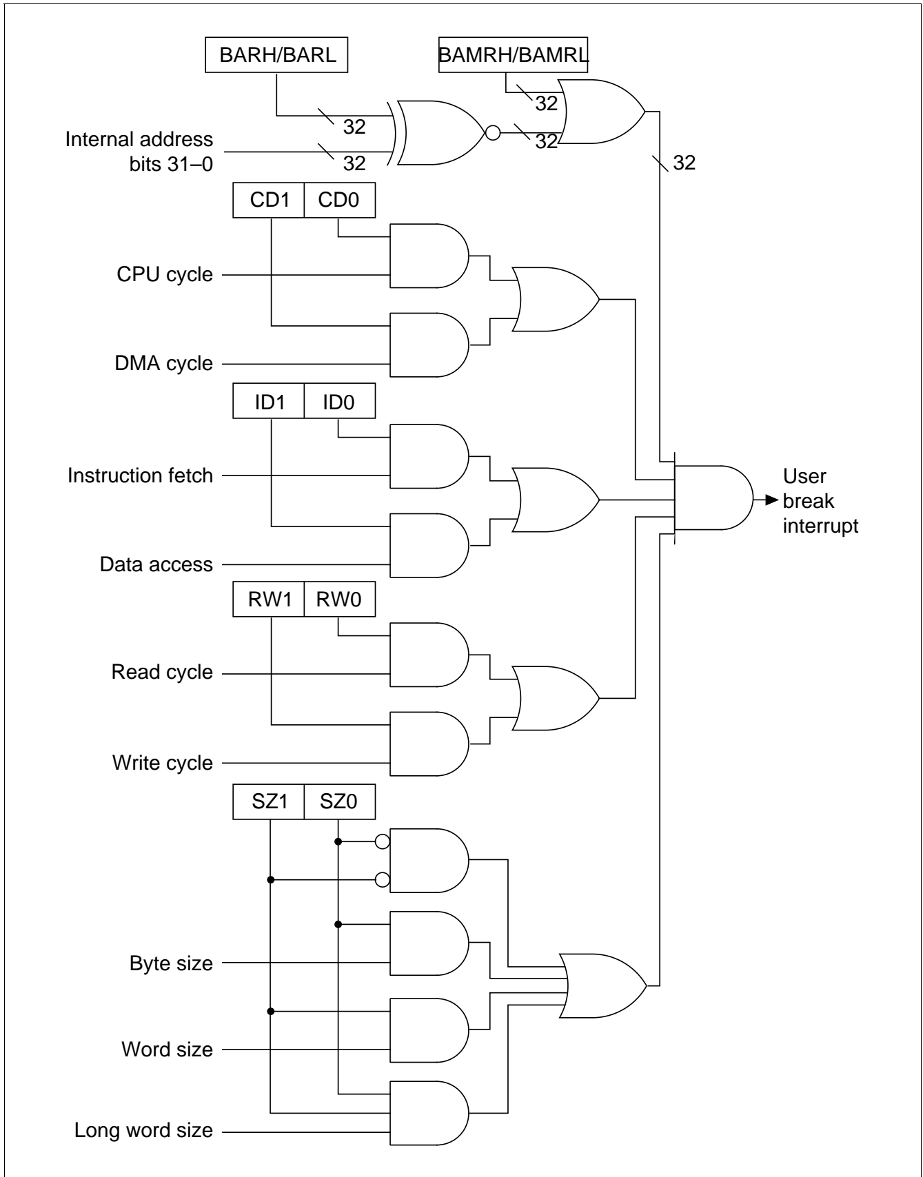
Figure 6.2 Break Condition Logic
