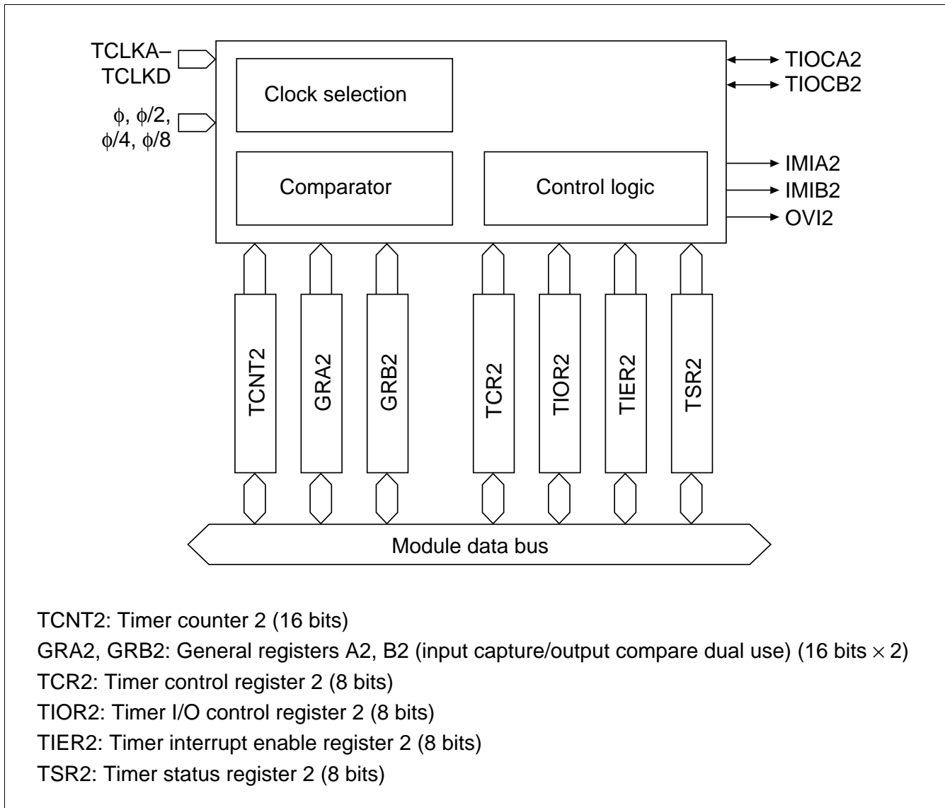
Figure 10.3 Channel 2 Block Diagram
