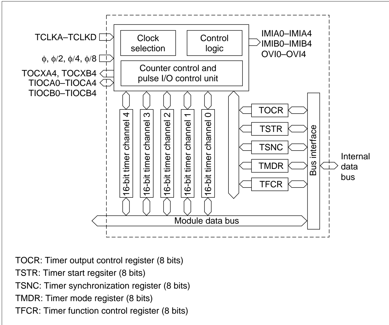
Figure 10.1 ITU Block Diagram
