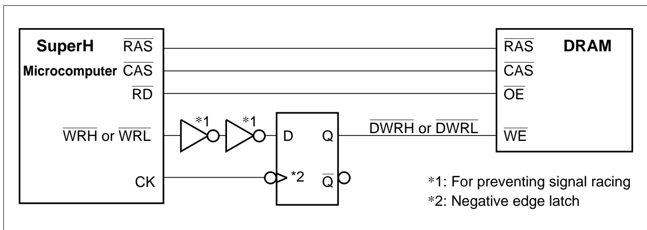
Figure 8.42 Delayed-Write Control Circuit
