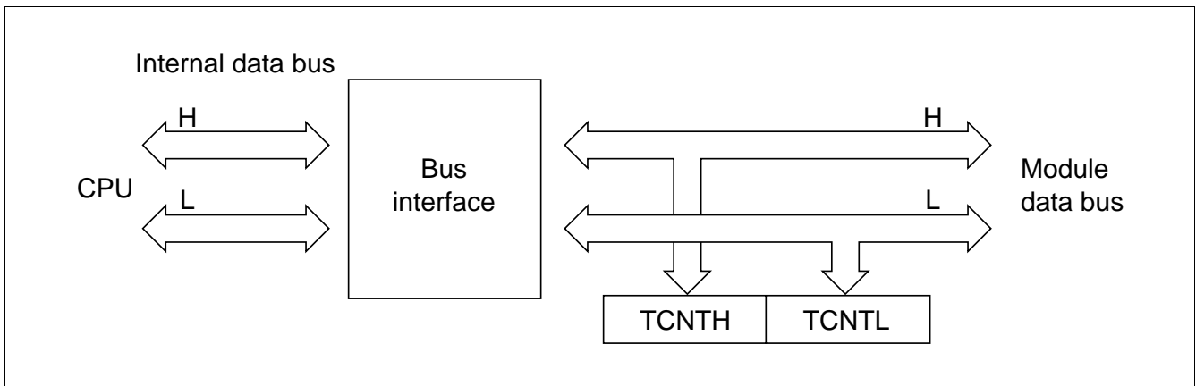
Figure 10.9 Accessing TCNT (CPU–TCNT (lower byte))
