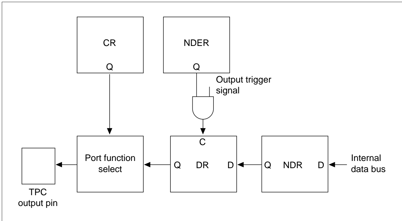
Figure 11.2 TPC Output Operation
