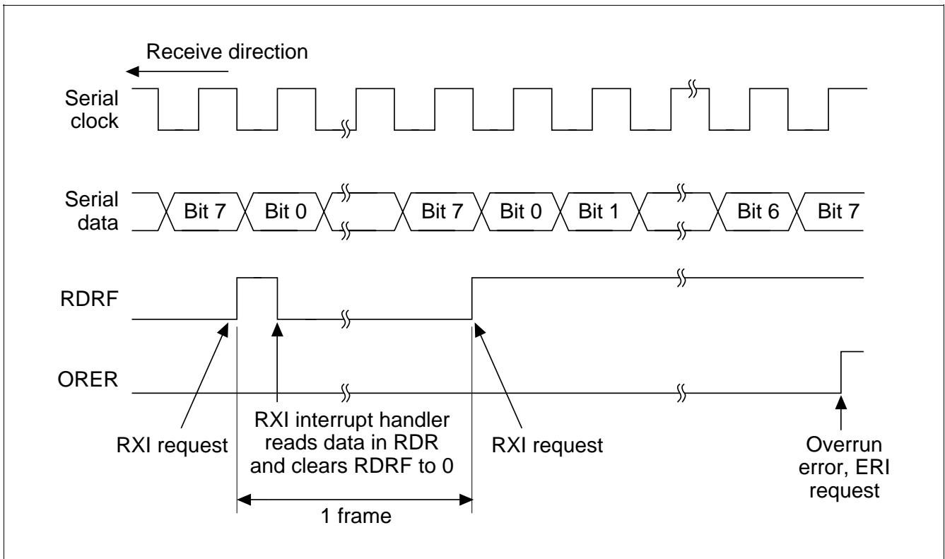
Figure 13.19 Example of SCI Receive Operation
