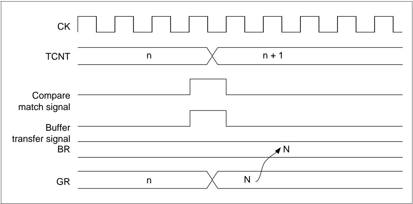
Figure 10.49 Compare Match Timing Example for Buffer Operation
