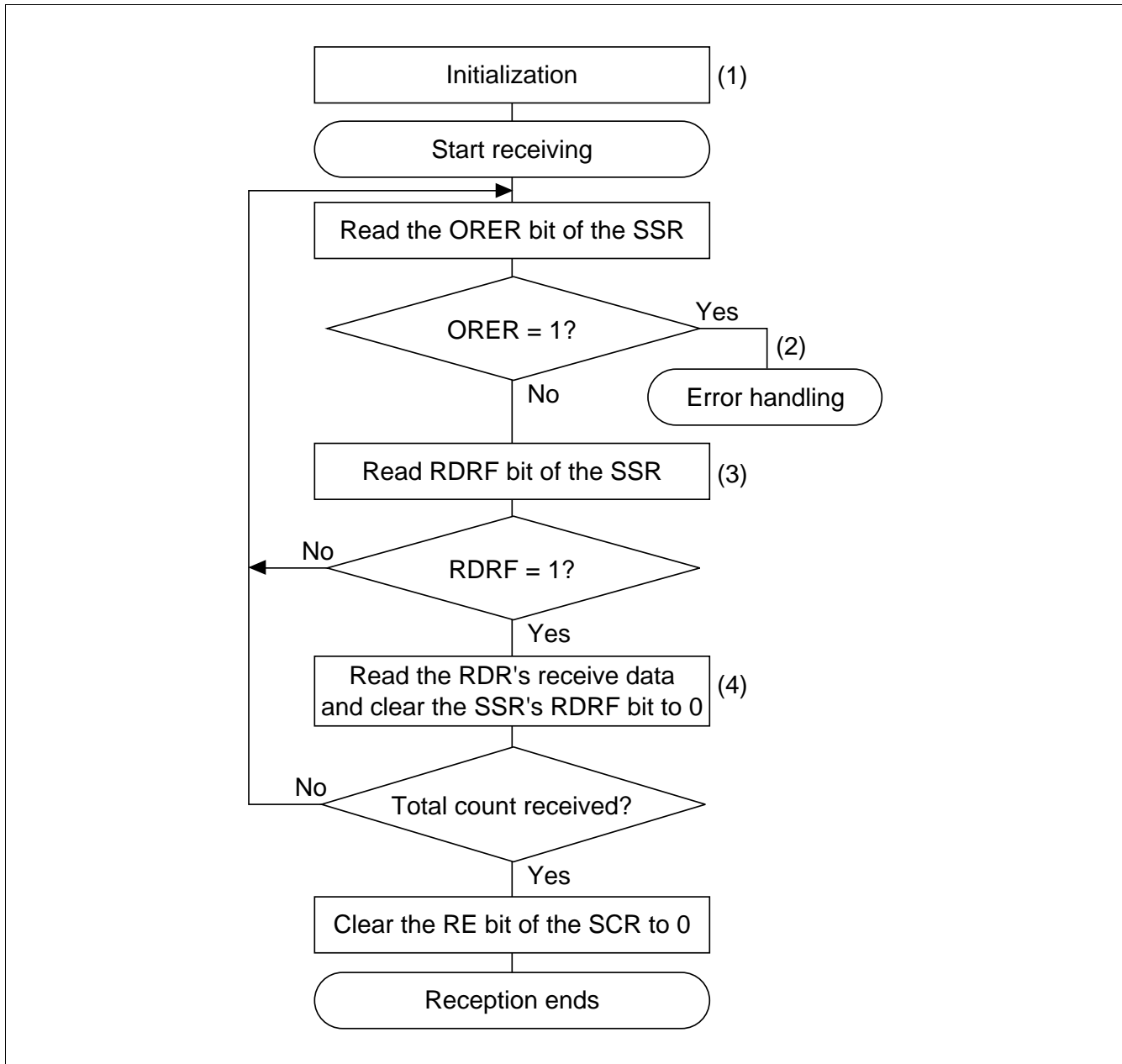
Figure 13.18 Sample Flowchart for Serial Receiving
