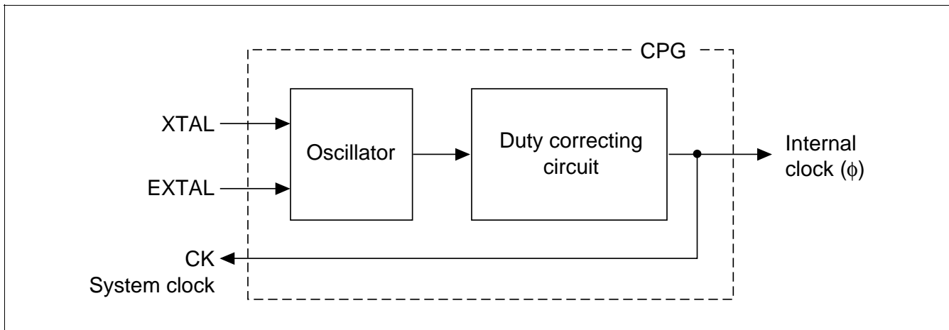
Figure 7.1 Block Diagram of the Clock Pulse Generator
