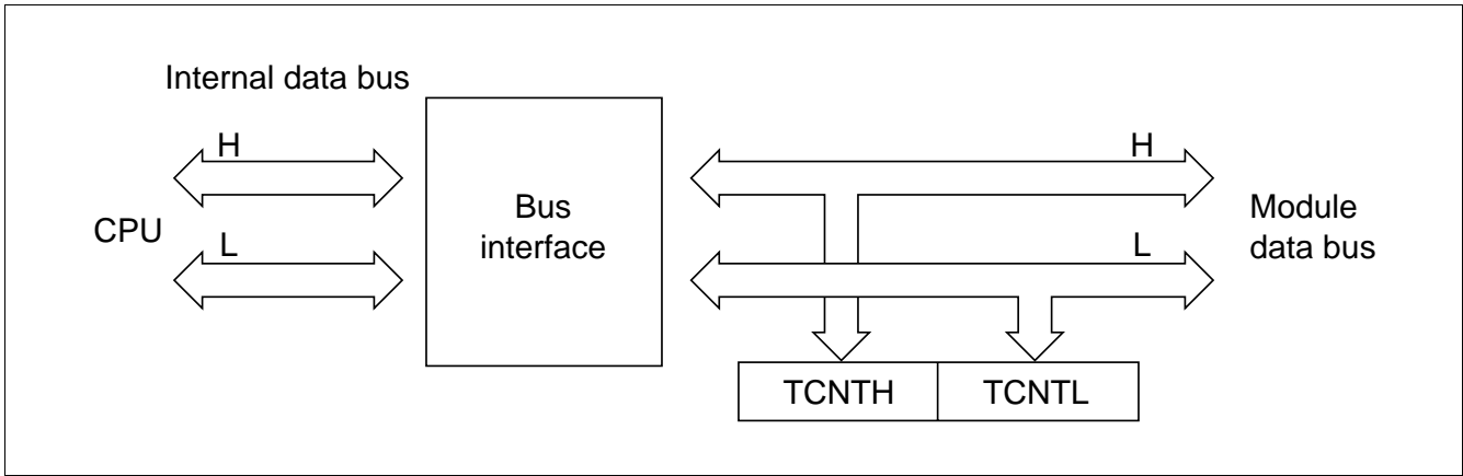
Figure 10.6 Accessing TCNT (CPU-TCNT (word))
