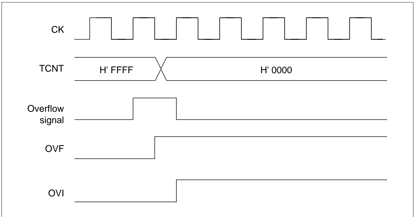
Figure 10.56 Timing of Setting OVF
