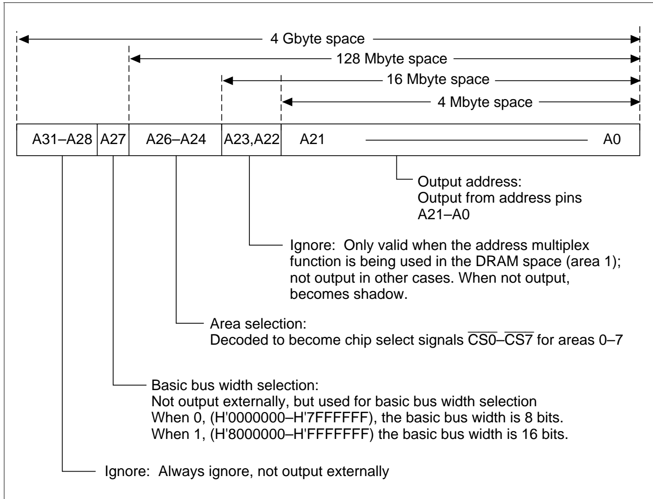
Figure 8.3 Address Format
