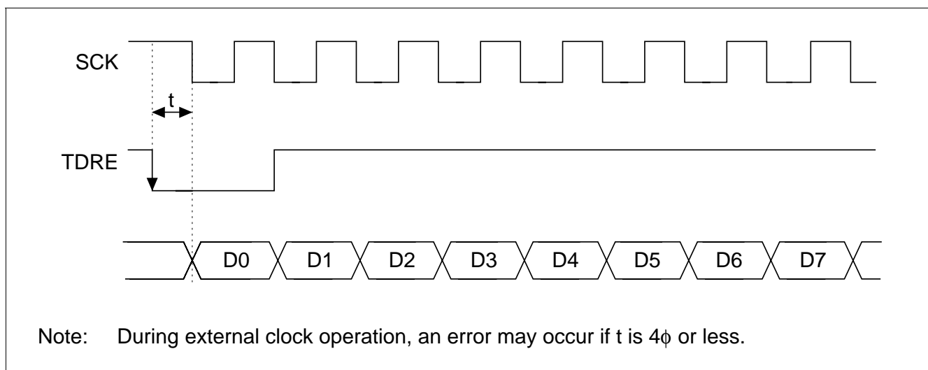
Figure 13.22 Clocked Synchronous Transmitting Example with DMAC
