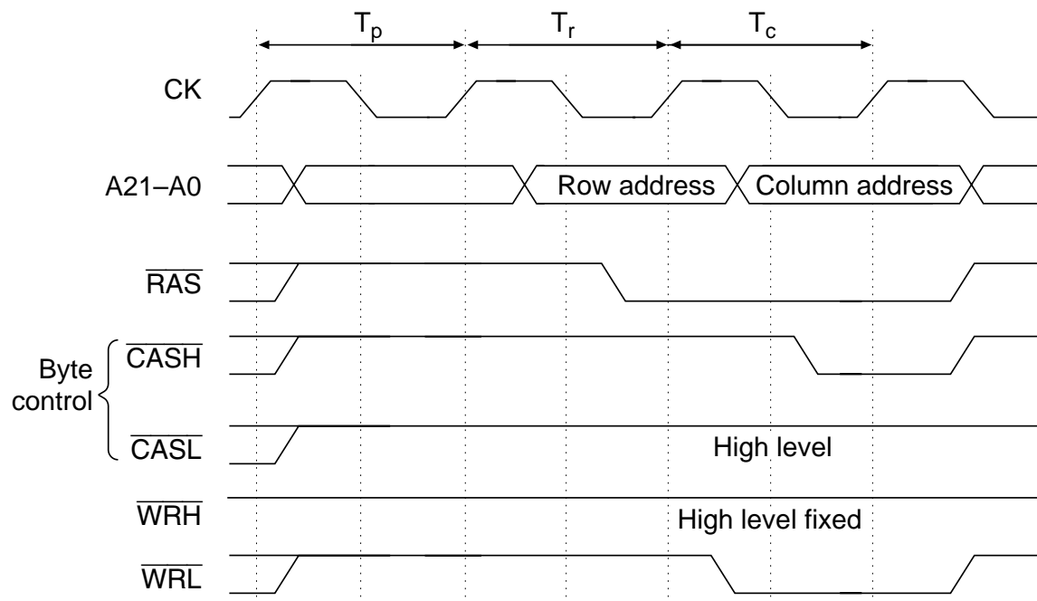
(a) Dual CAS signals (CW2 = 0)
