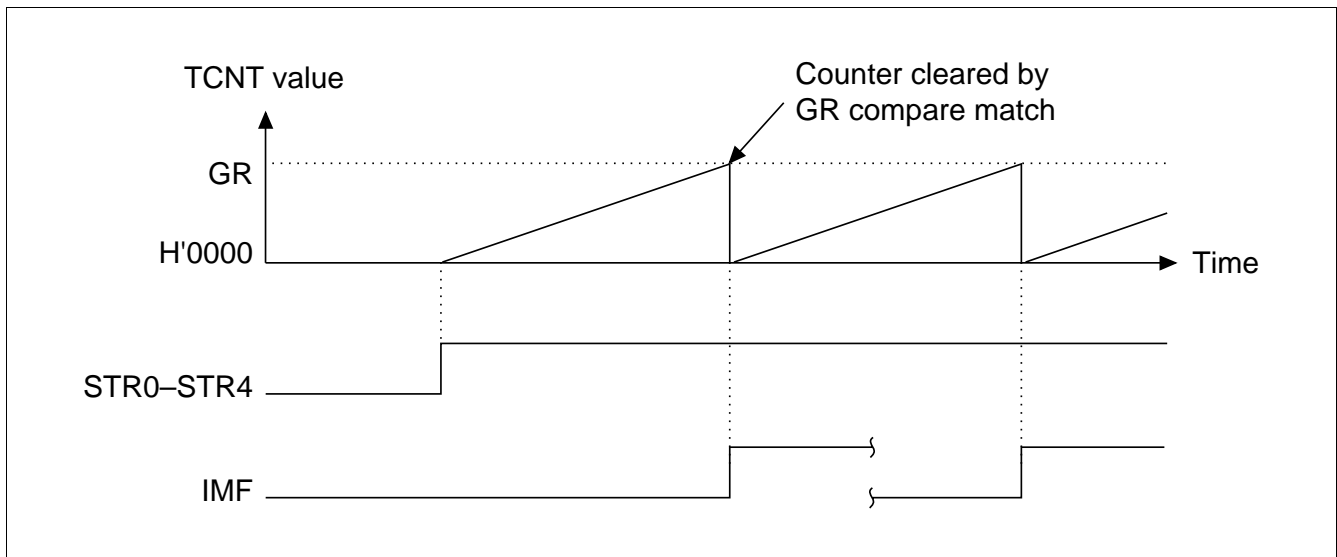
Figure 10.16 Periodic Counter Operation
