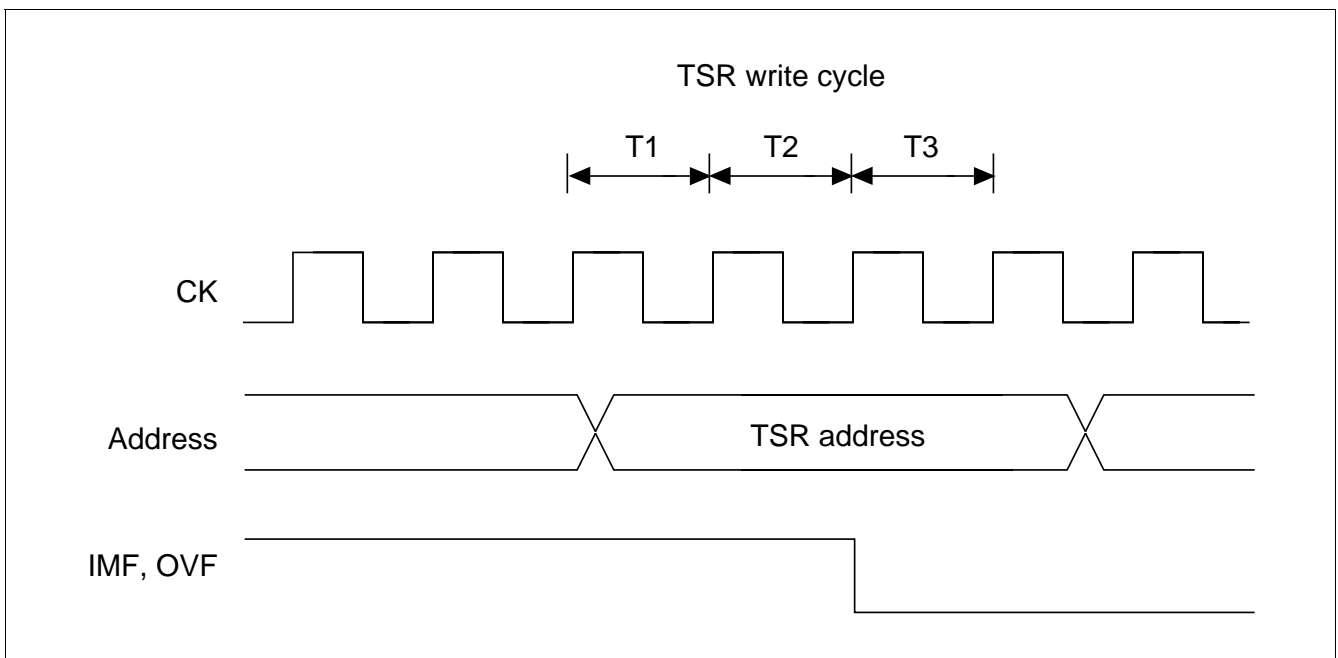
Figure 10.57 Timing of Status Flag Clearing
