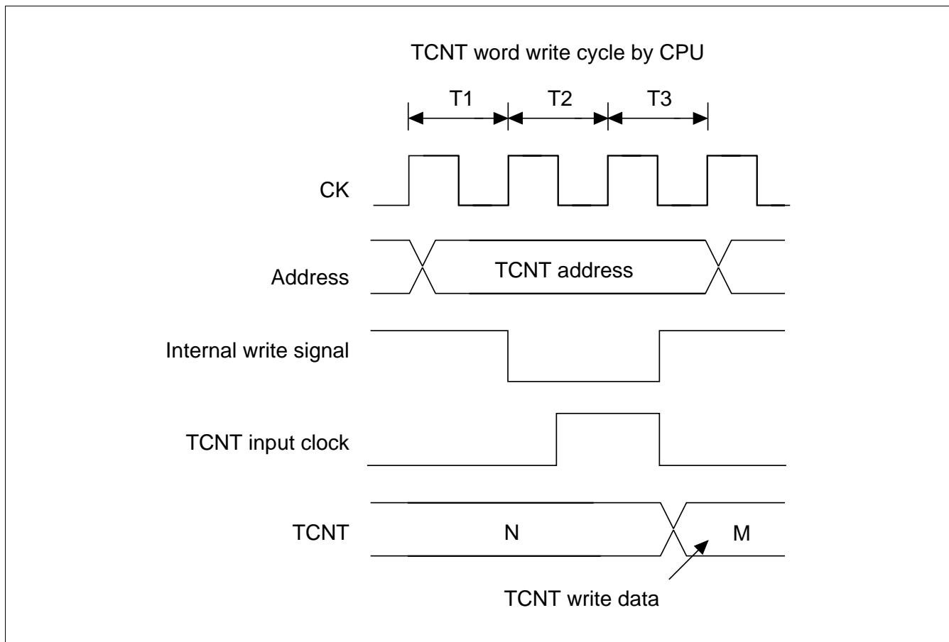
Figure 10.59 Contention between TCNT Word Write and Increment
