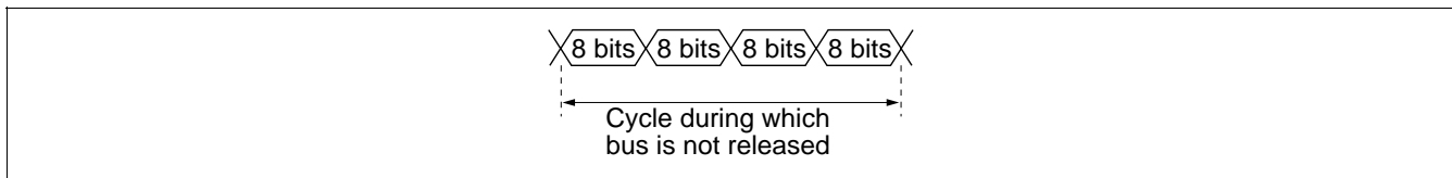
Figure 8.44 One Bus Cycle
