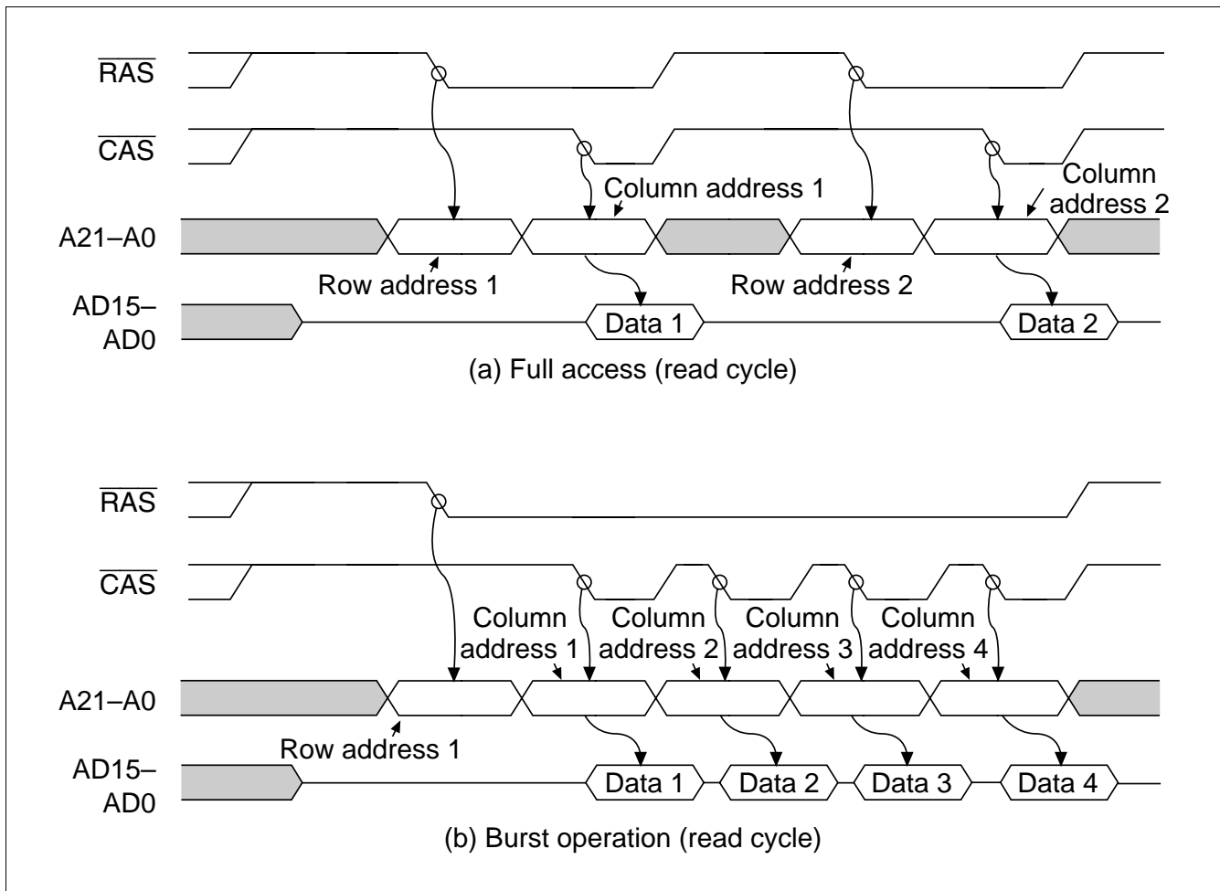
Figure 8.22 Full Access and Burst Operation
