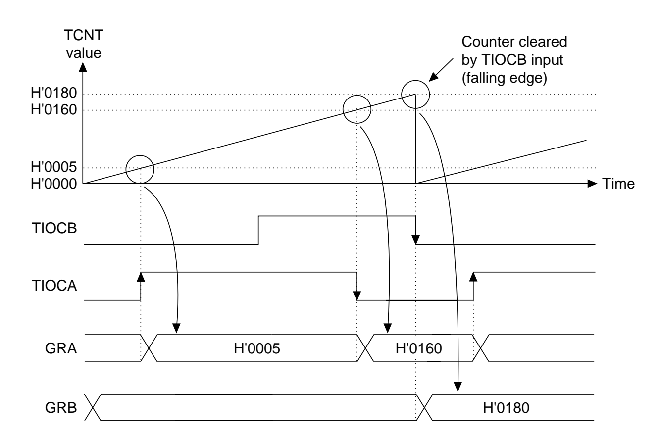
Figure 10.24 Input Capture Operation
