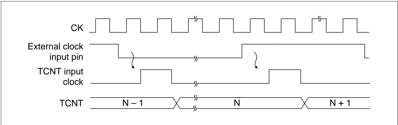
Figure 10.18 Count Timing for External Clock Sources
