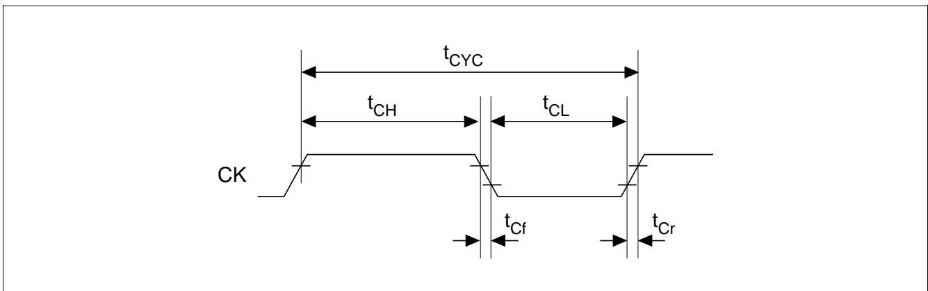
Figure 19.2 System Clock Timing
