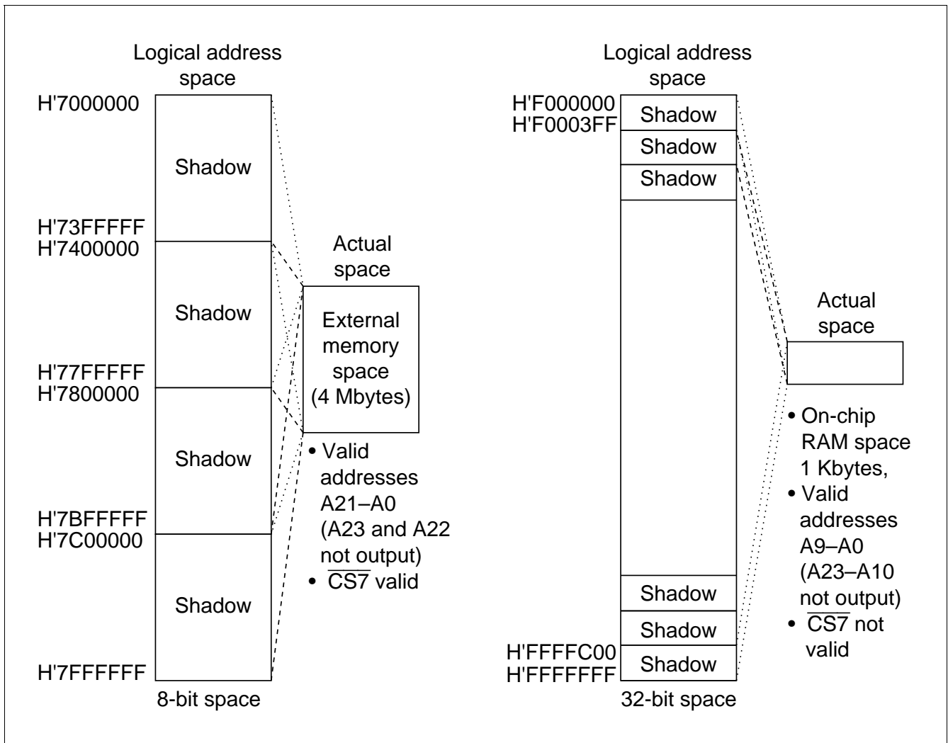
Figure 8 10 Memory Map of Area 7
