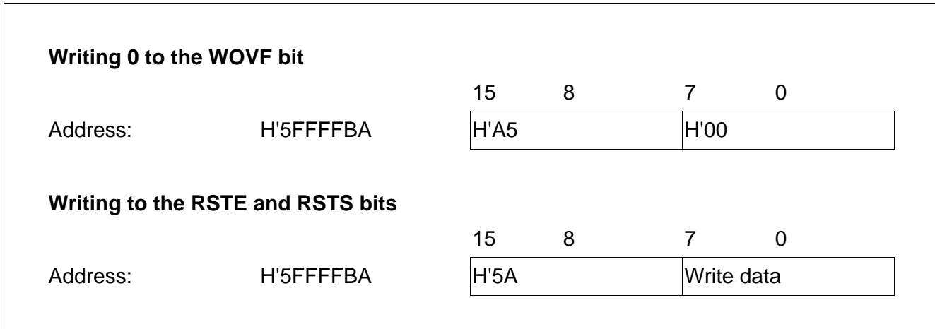
Figure 12.3 Writing to the RSTCSR
