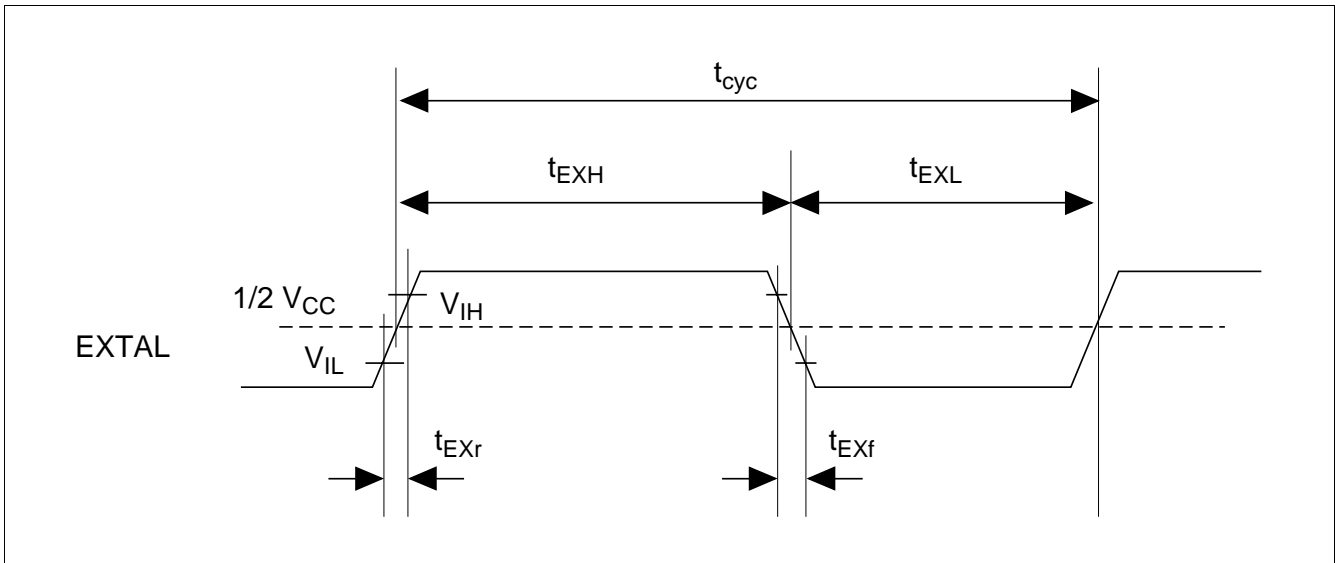
Figure 19.1 EXTAL Input Timing
