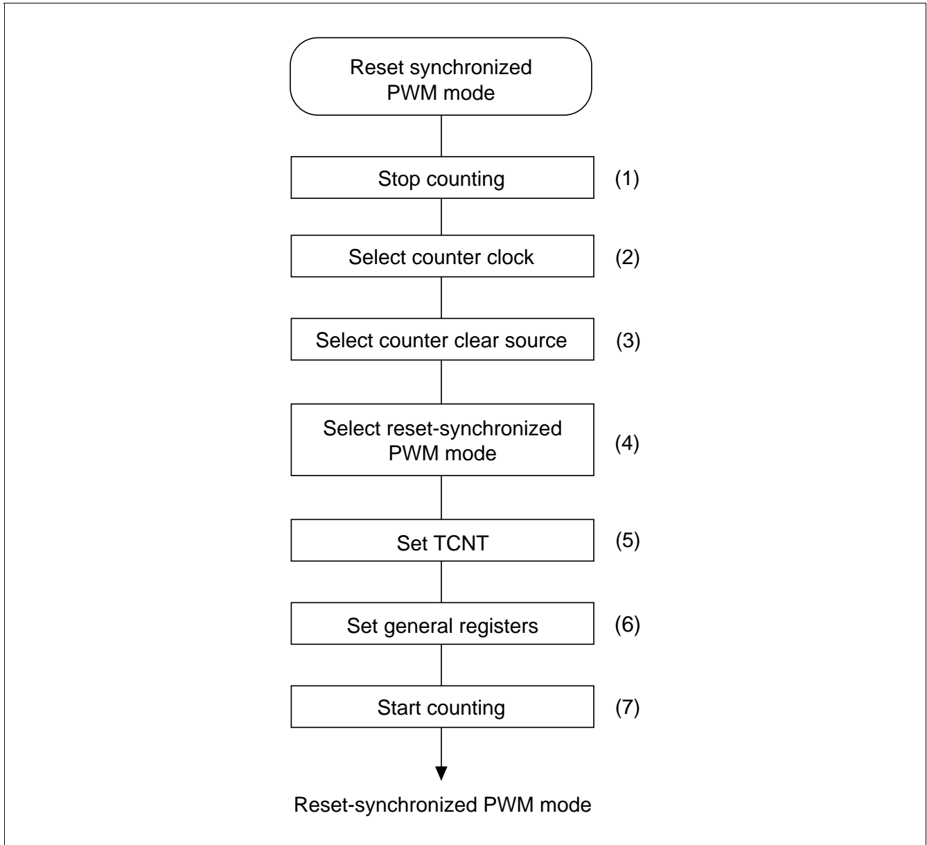
Figure 10.31 Procedure for Selecting the Reset-Synchronized PWM Mode
