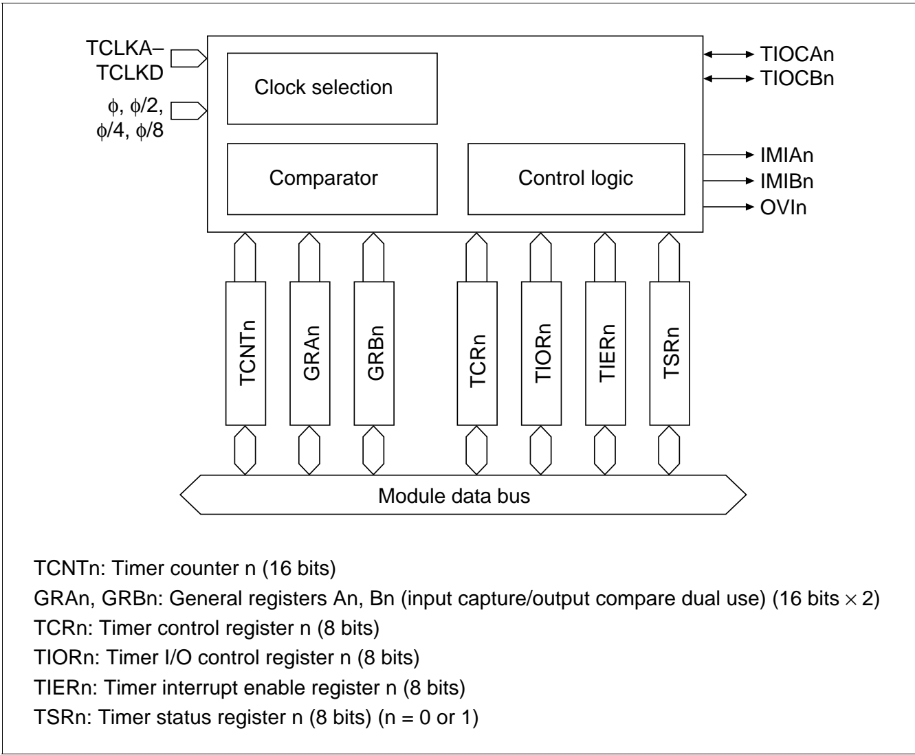
Figure 10.2 Channels 0 and 1 Block Diagram (One Channel Shown)
