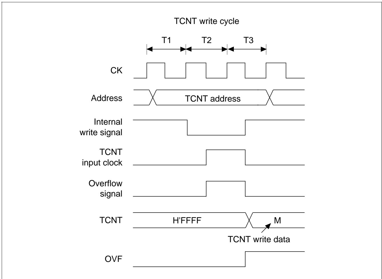
Figure 10.62 Contention between TCNT Write and Overflow
