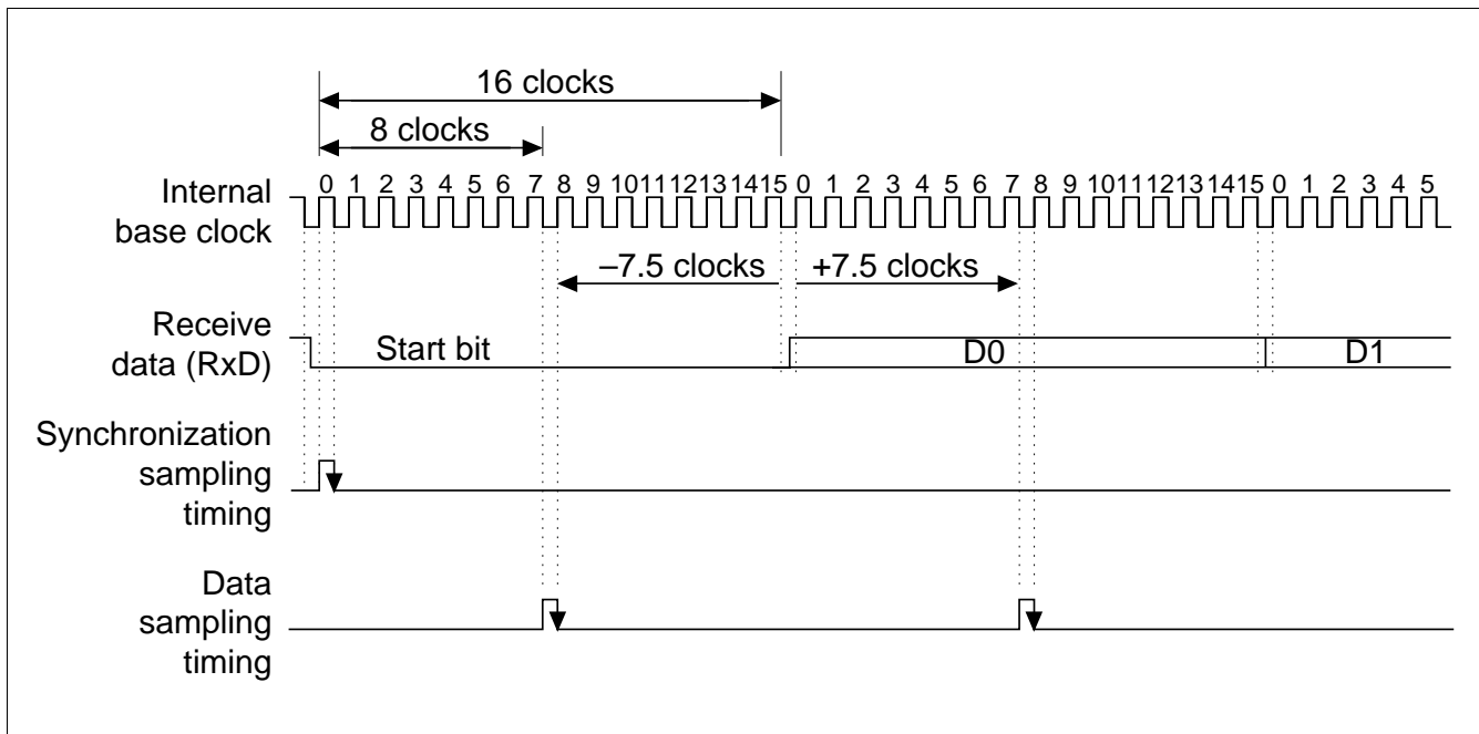
Figure 13.21 Receive Data Sampling Timing in Asynchronous Mode
