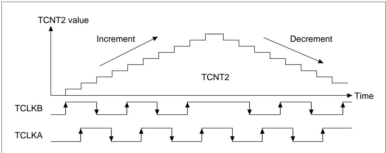
Figure 10.43 Phase Counting Mode Operation
