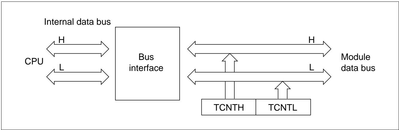
Figure 10.7 Accessing TCNT (TCNT-CPU (word))
