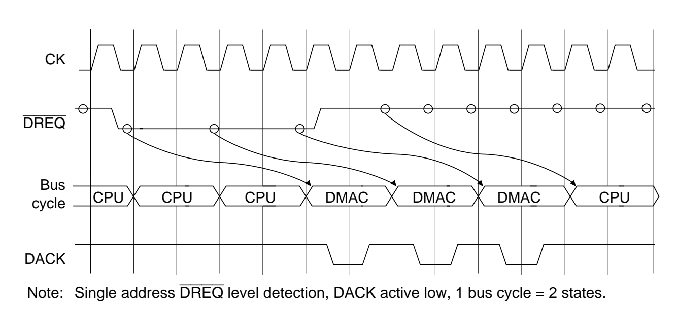
Figure 9.23 \overline{\text{DREQ}} Pin Sampling Timing in Burst Mode
