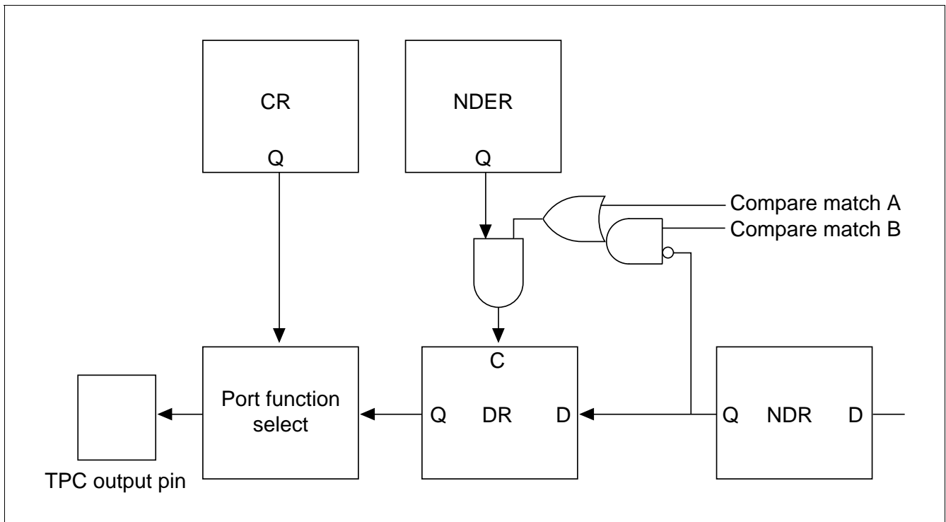
Figure 11.9 TPC Output Non-Overlap Operation
