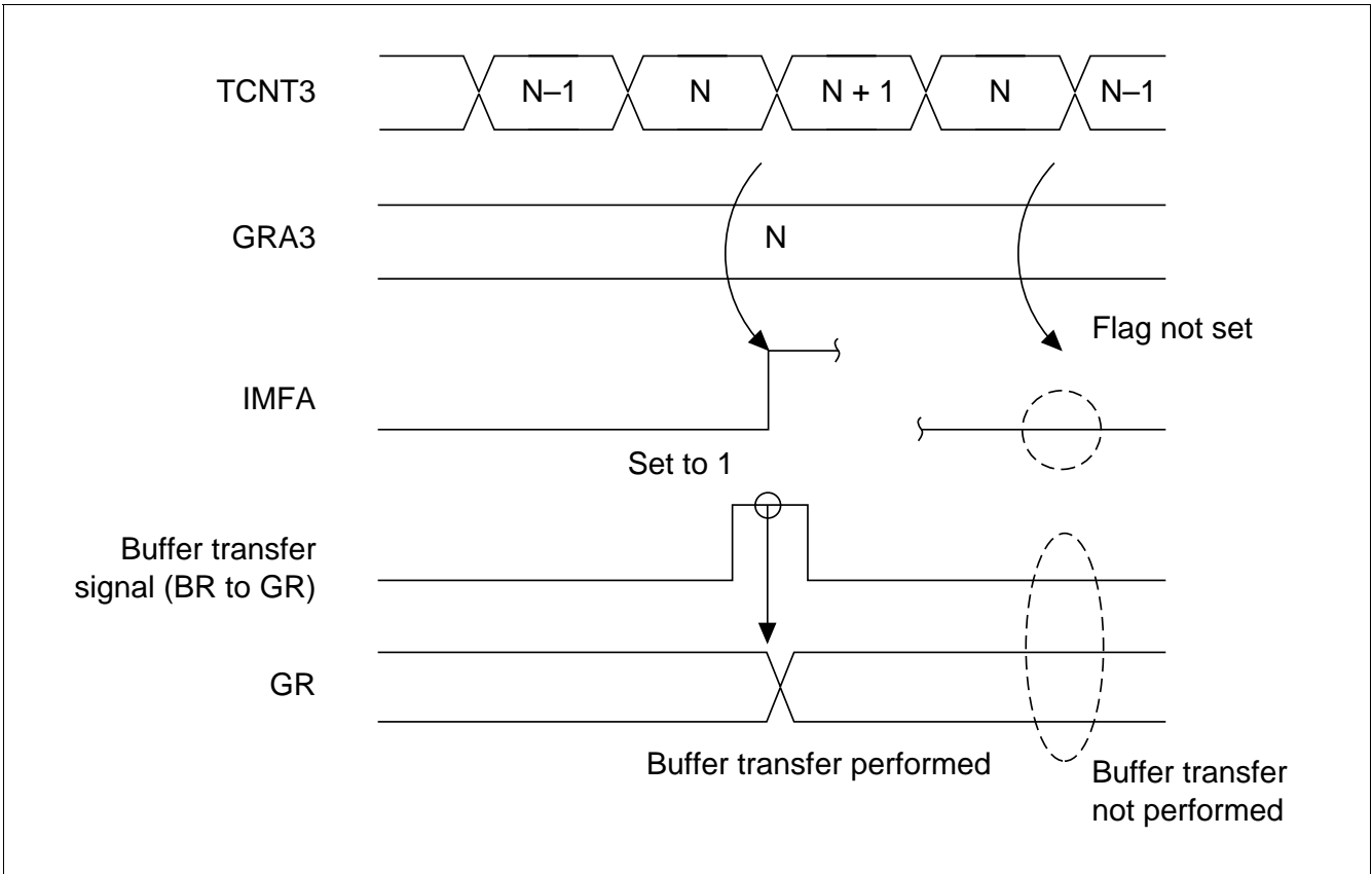
Figure 10.36 Overshoot Timing
