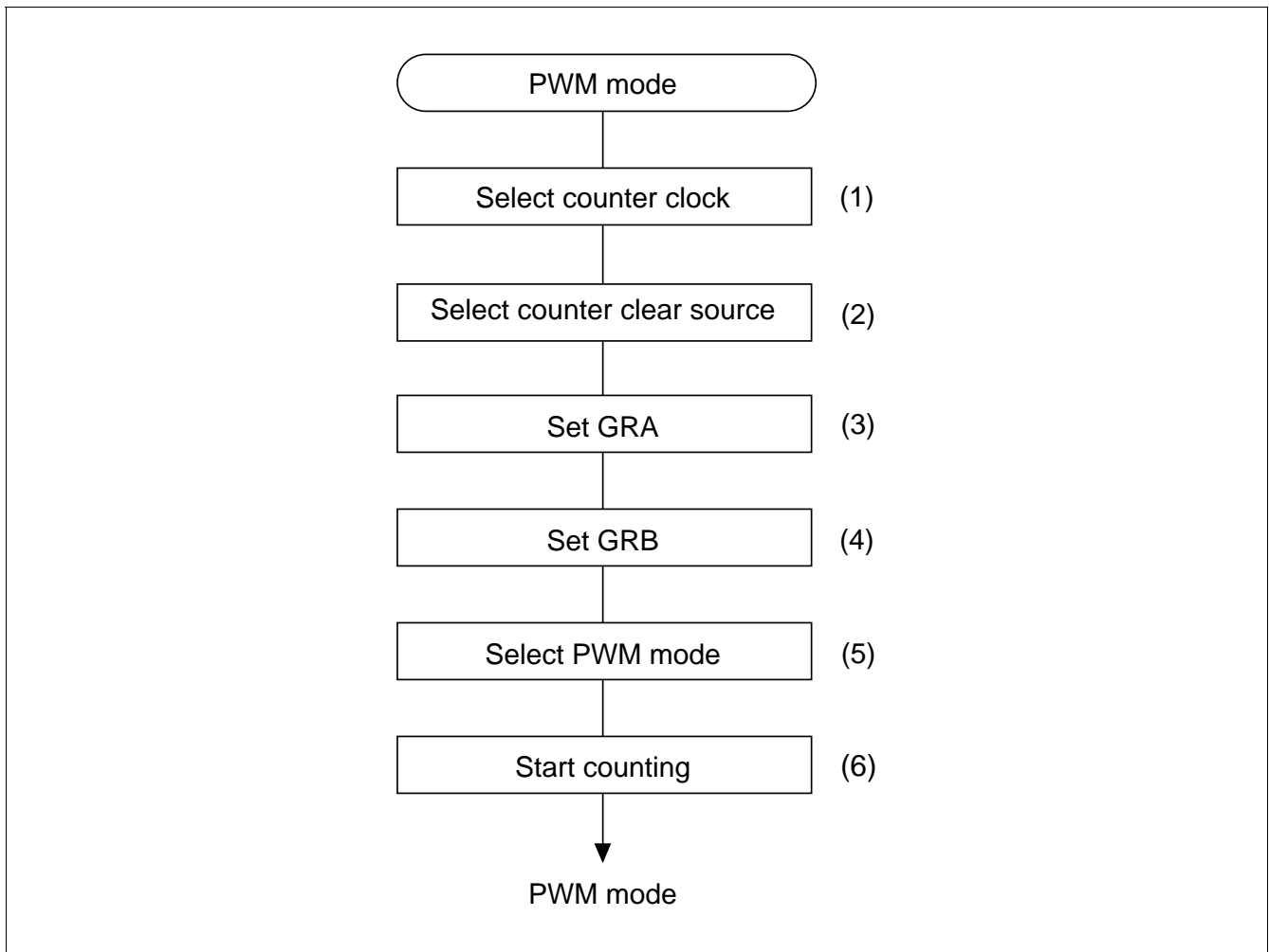
Figure 10.28 Procedure for Selecting the PWM Mode
