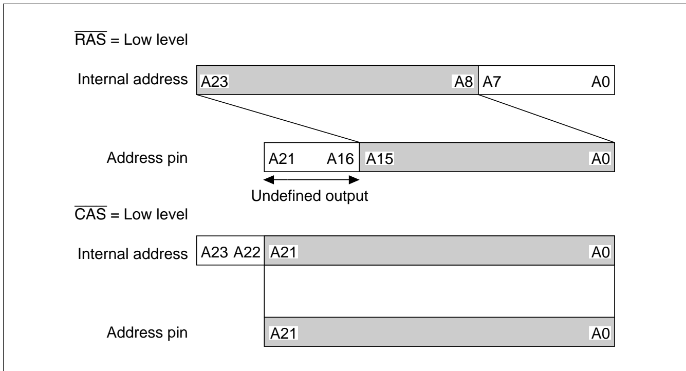
Figure 8.16 Address Multiplexing States (8-bit shift)
