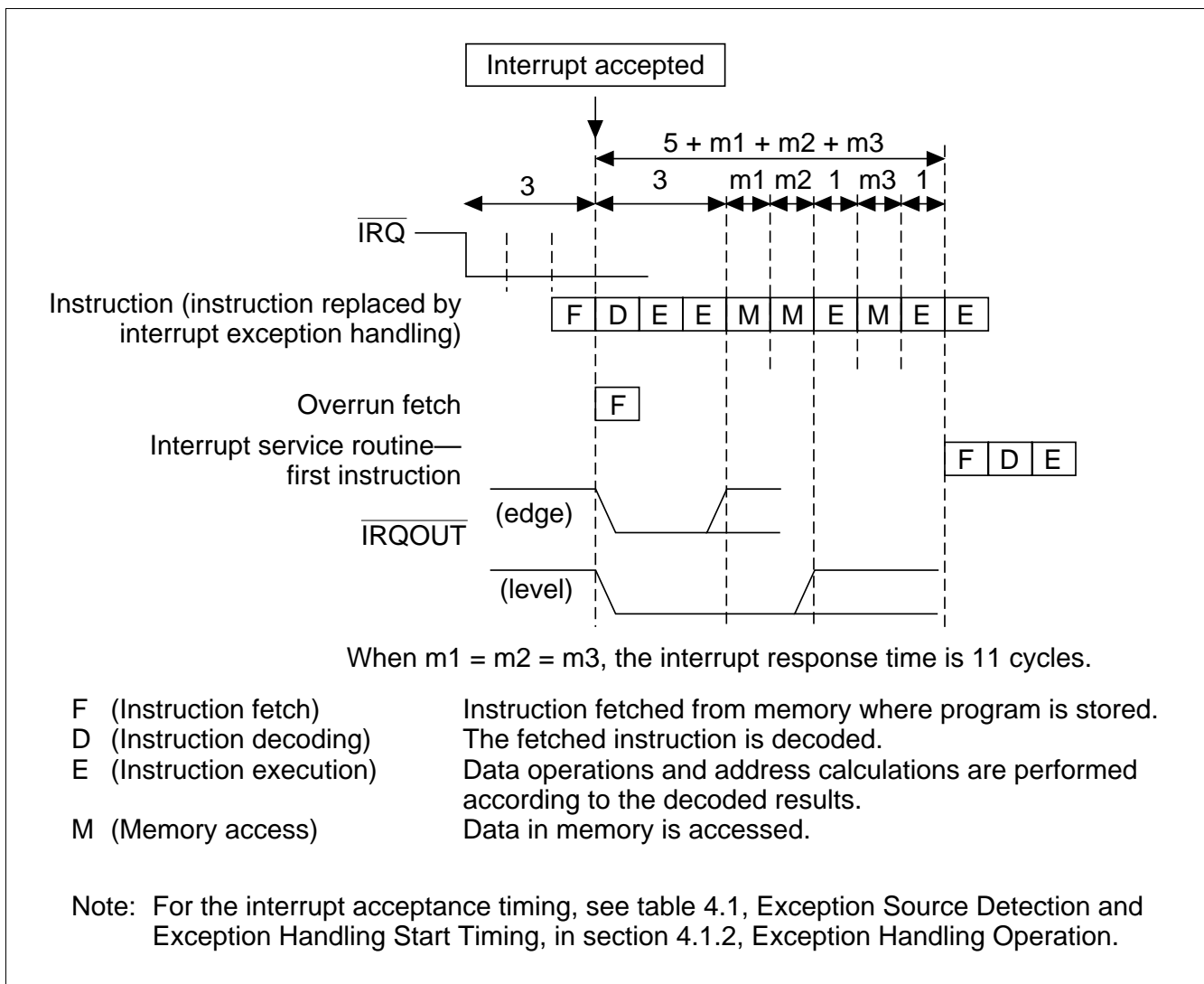
Figure 5.4 Example of Pipelining in IRQ Interrupt Acceptance
