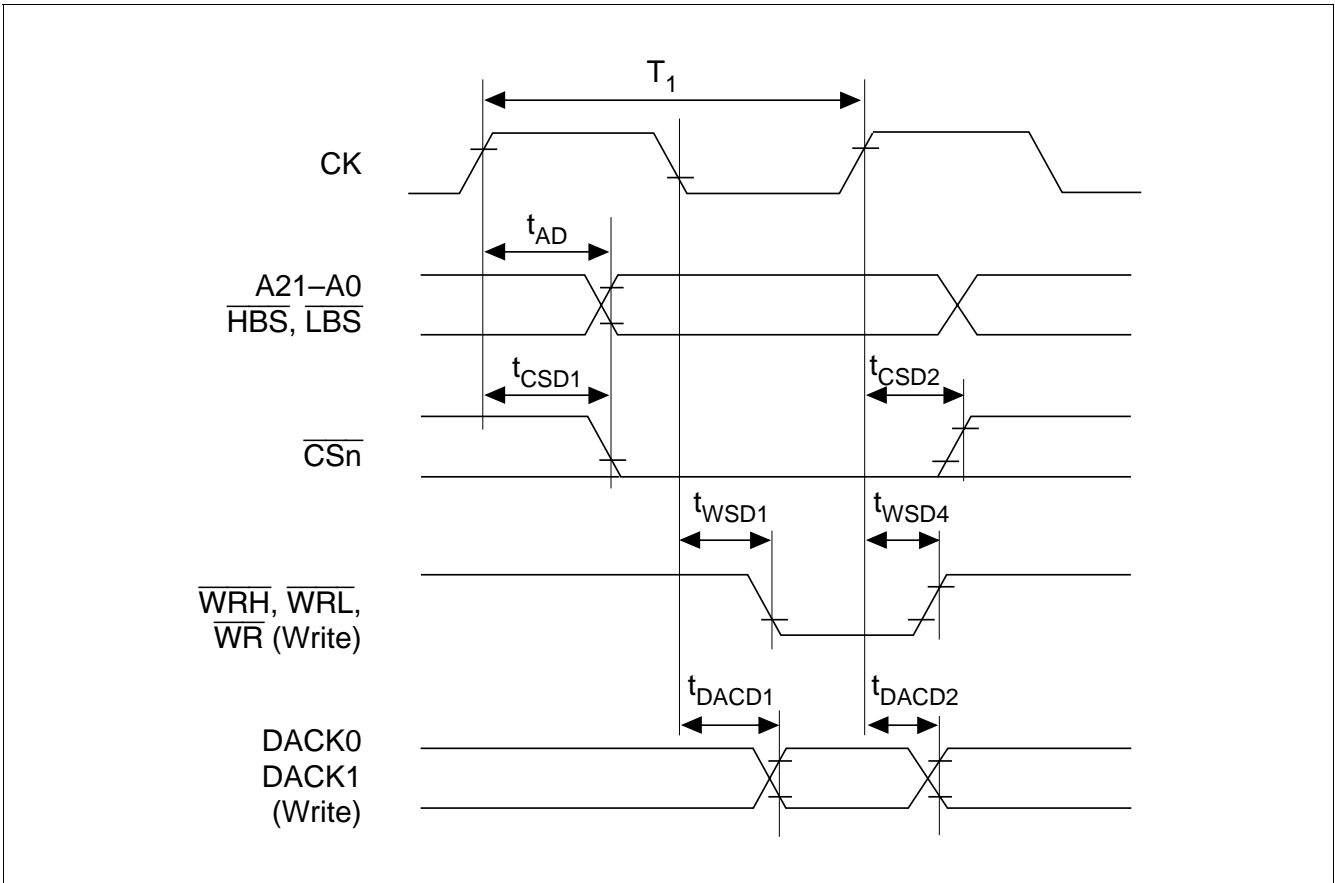
Figure 19.20 DMA Single Transfer/1 State Access Write
