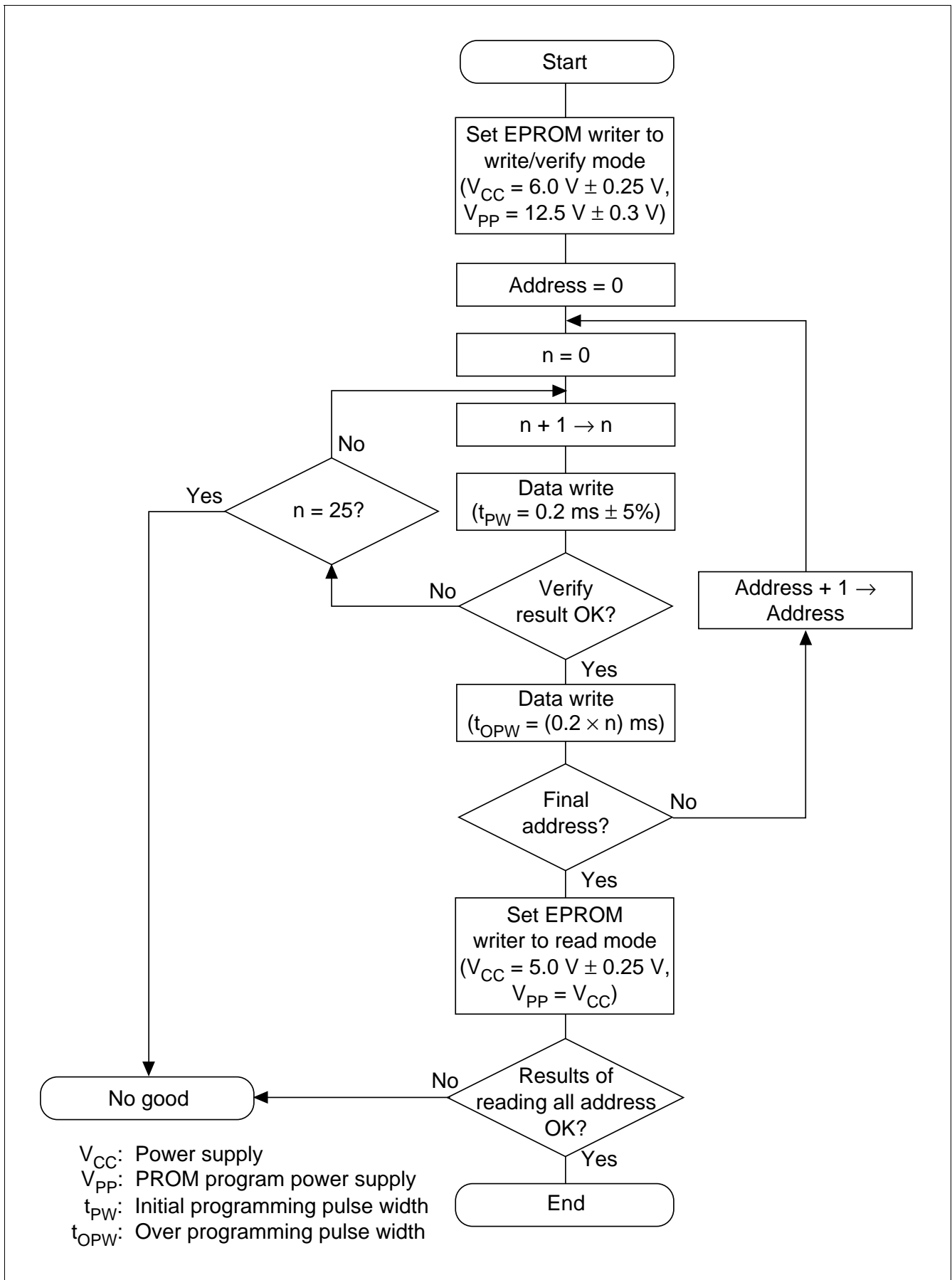
Figure 16.4 Basic Flowchart of High-Speed High-Reliability Programming
