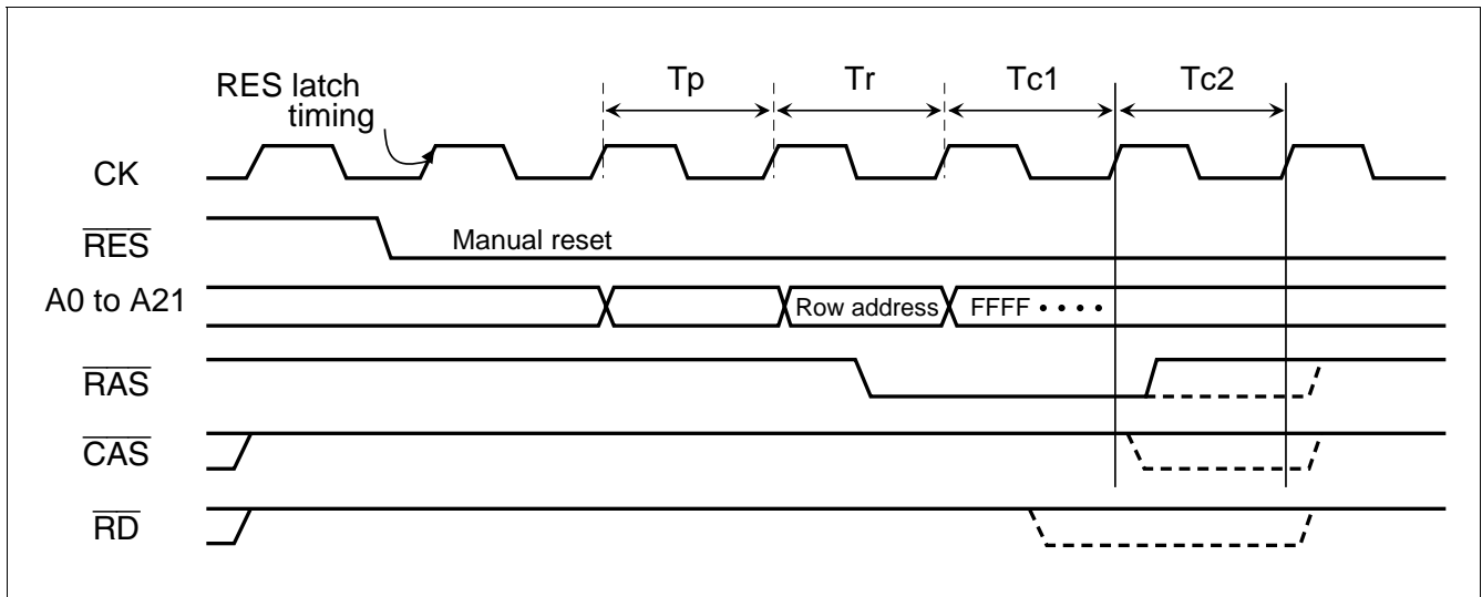
Figure 8.41 Long - pitch Mode Read (2)
