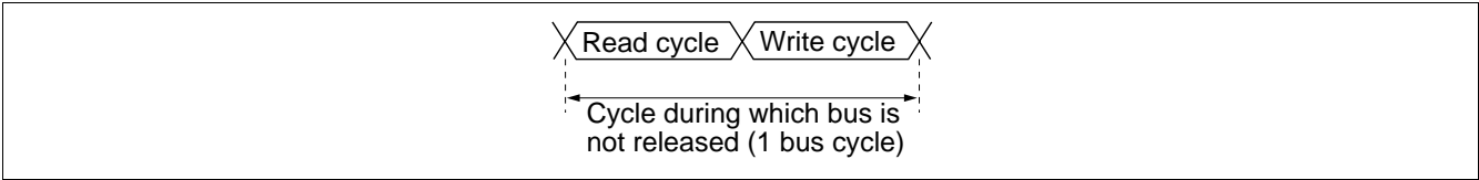
Figure 8.45 TAS Instruction Read Cycle and Write Cycle
