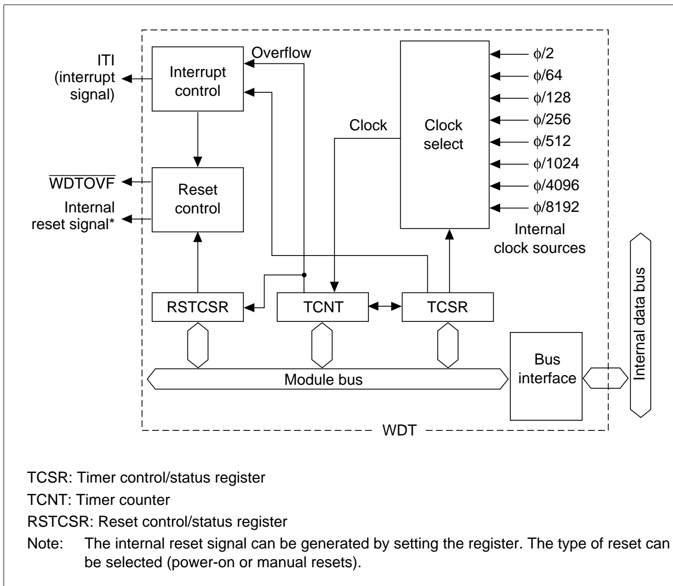
Figure 12.1 WDT Block Diagram
