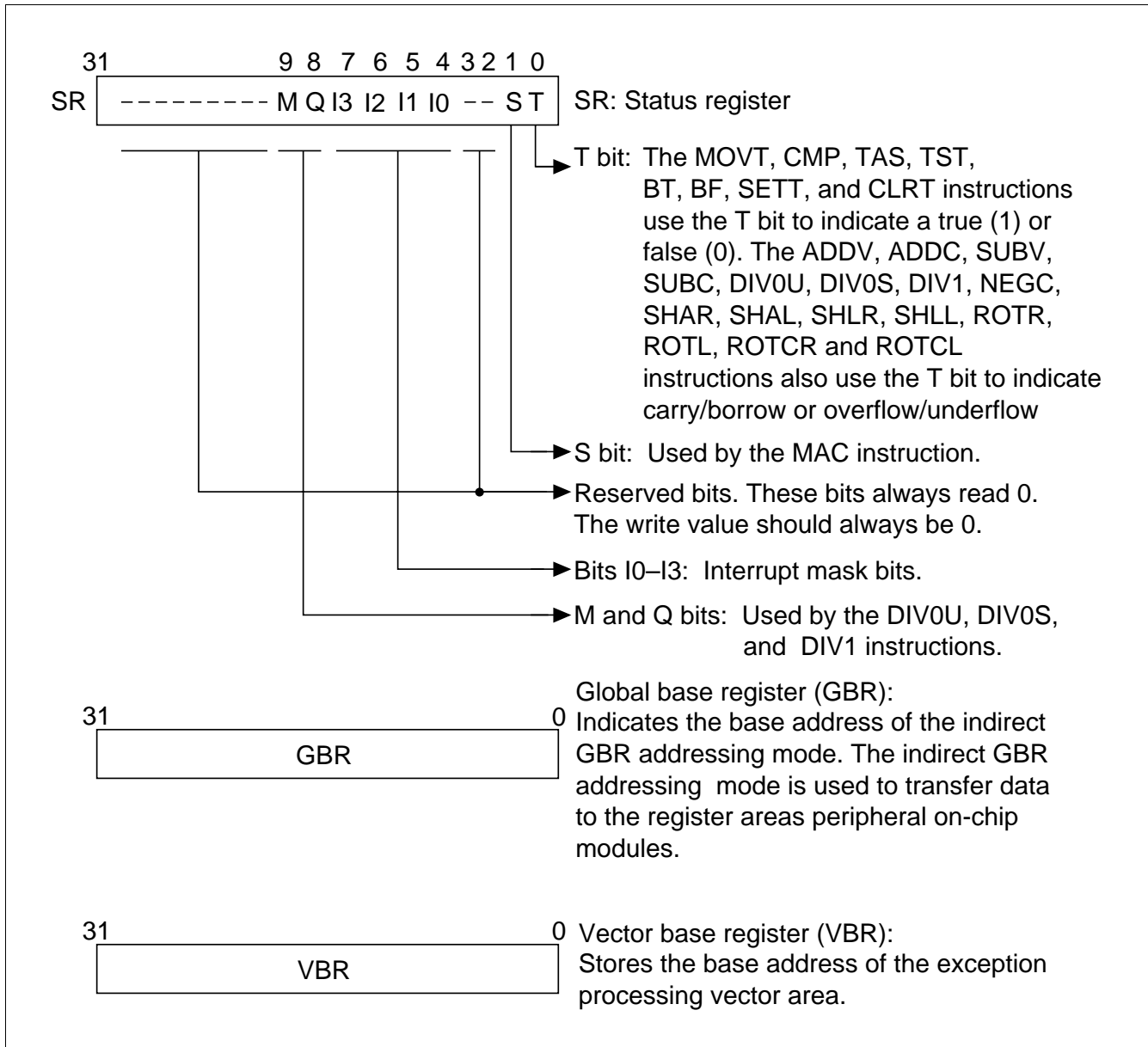
Figure 2.2 Control Registers
