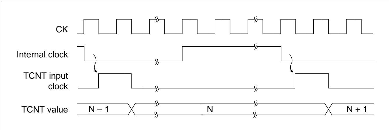
Figure 10.17 Count Timing for Internal Clock Sources
