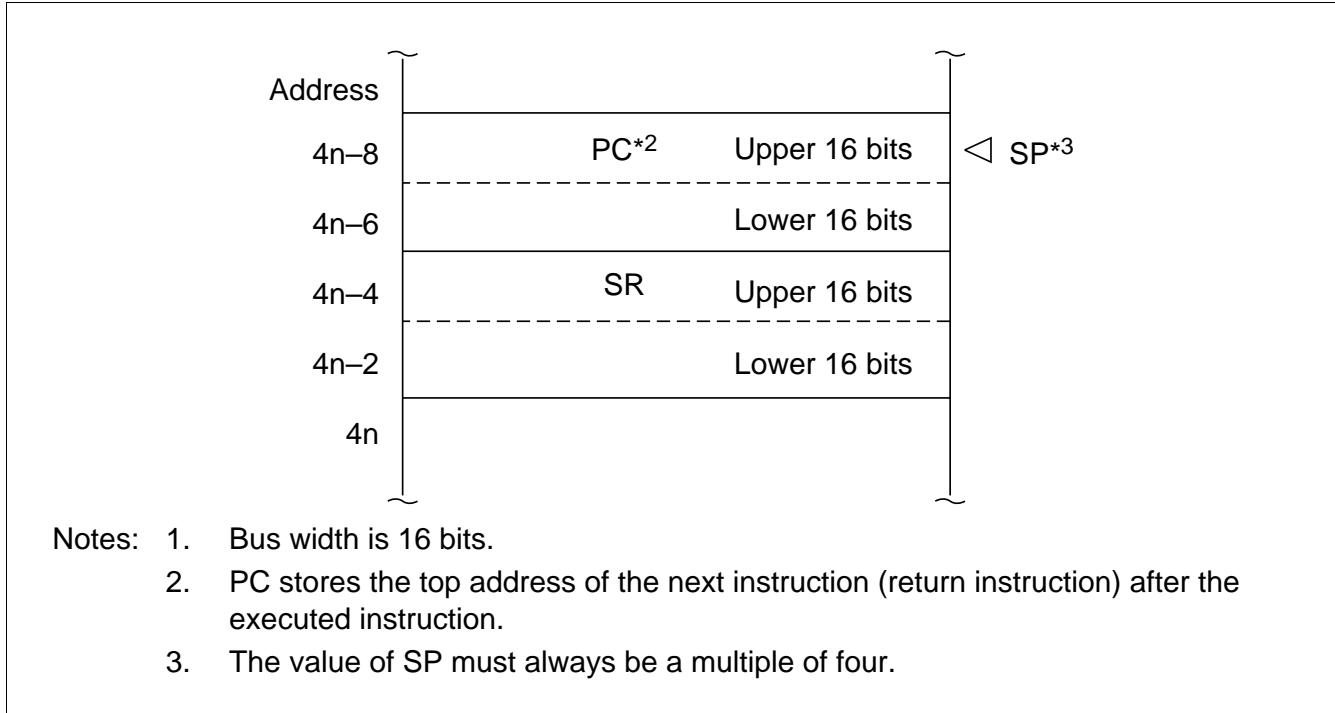
Figure 5.3 Stack after Interrupt Exception Processing
