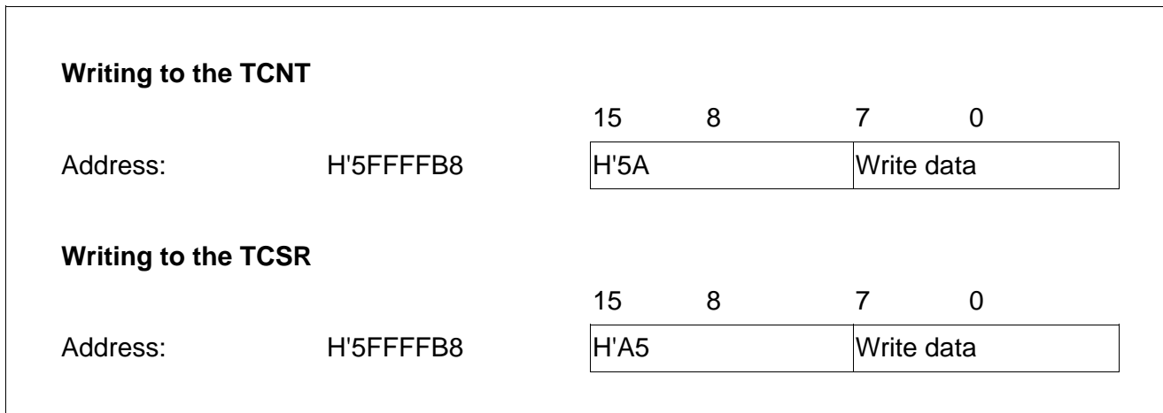
Figure 12.2 Writing to the TCNT and TCSR
