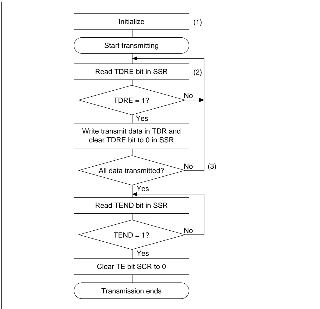
Figure 13.17 Sample Flowchart for Serial Transmitting
