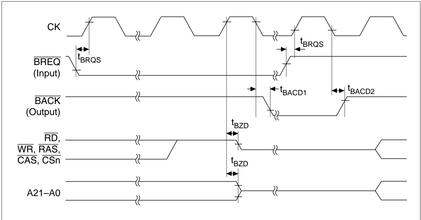
Figure 19.7 Bus Release Timing
