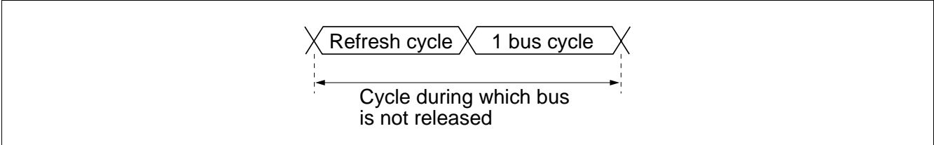
Figure 8.46 Refresh Cycle and Following Bus Cycle
