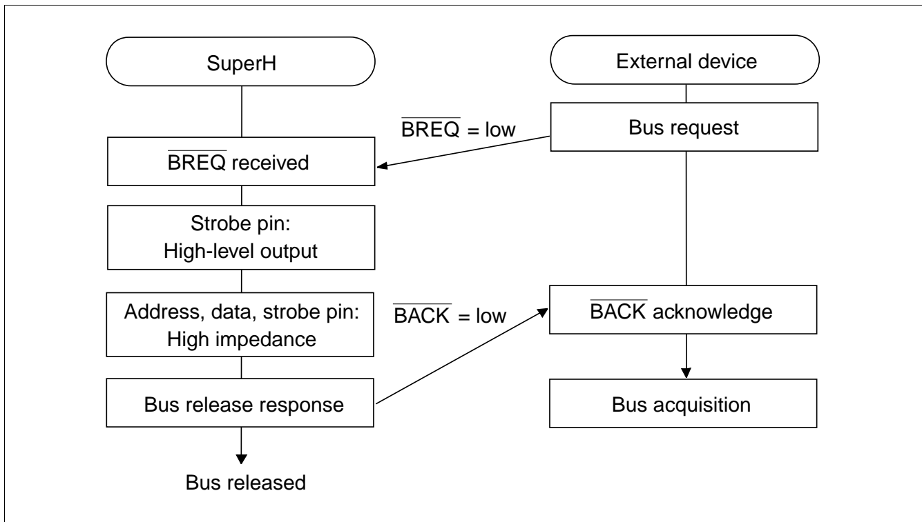
Figure 8.35 Bus Release Procedure
