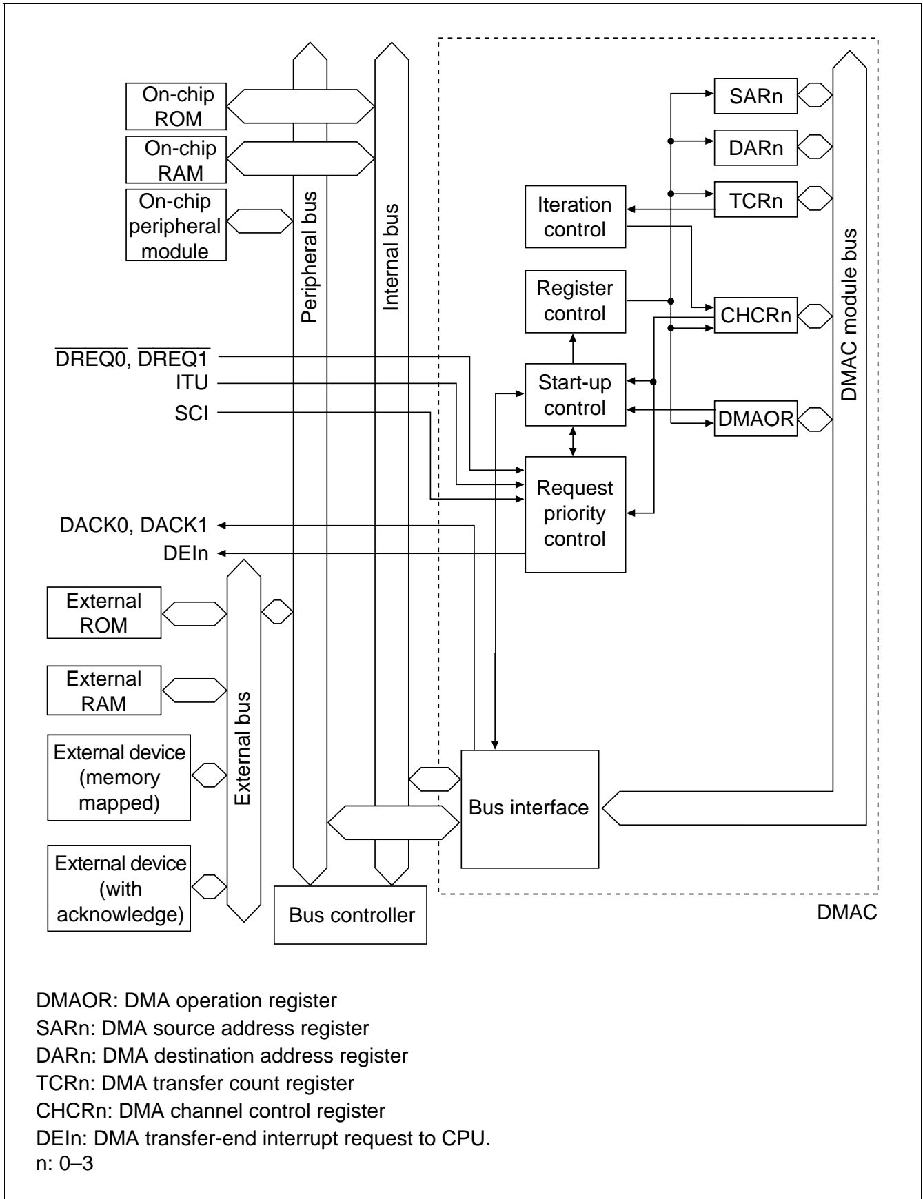
Figure 9.1 DMAC Block Diagram
