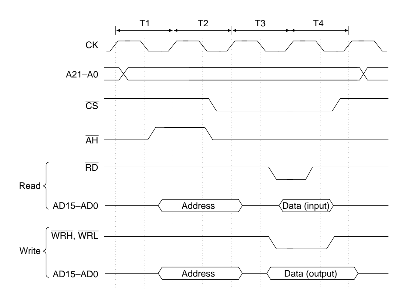
Figure 8.32 Access Timing For Address/Data Multiplexed I/O Space
