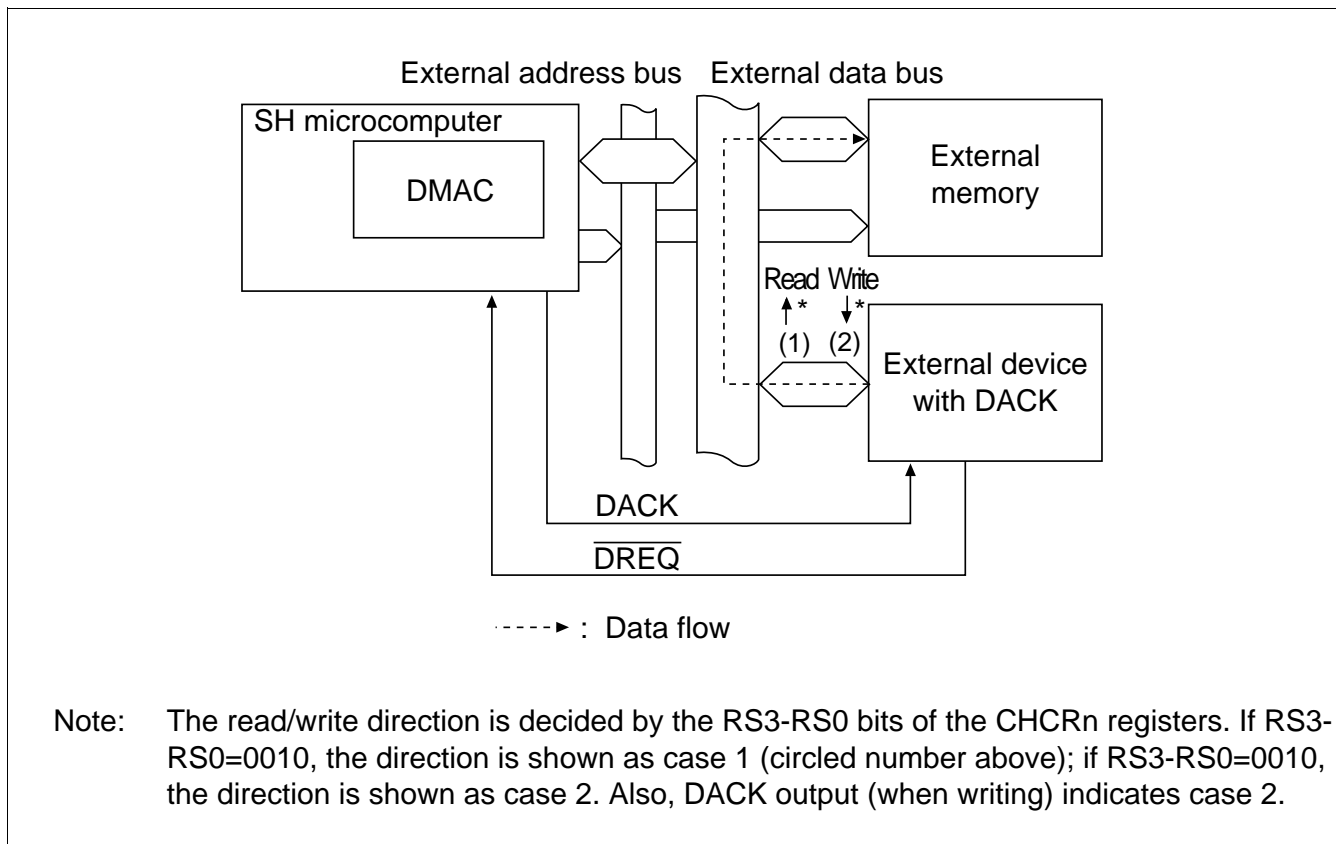
Figure 9.6 Data Flow in Single Address Mode
