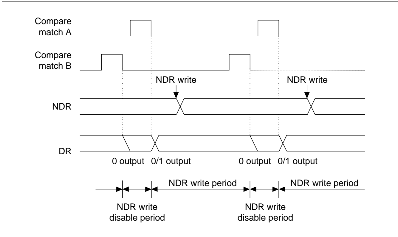
Figure 11.10 Non-Overlap Operation and NDR Write Timing
