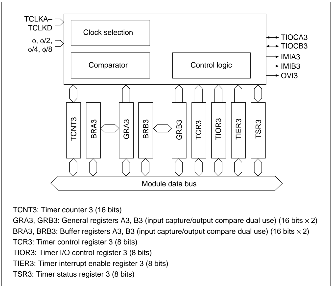
Figure 10.4 Channels 3 Block Diagram
