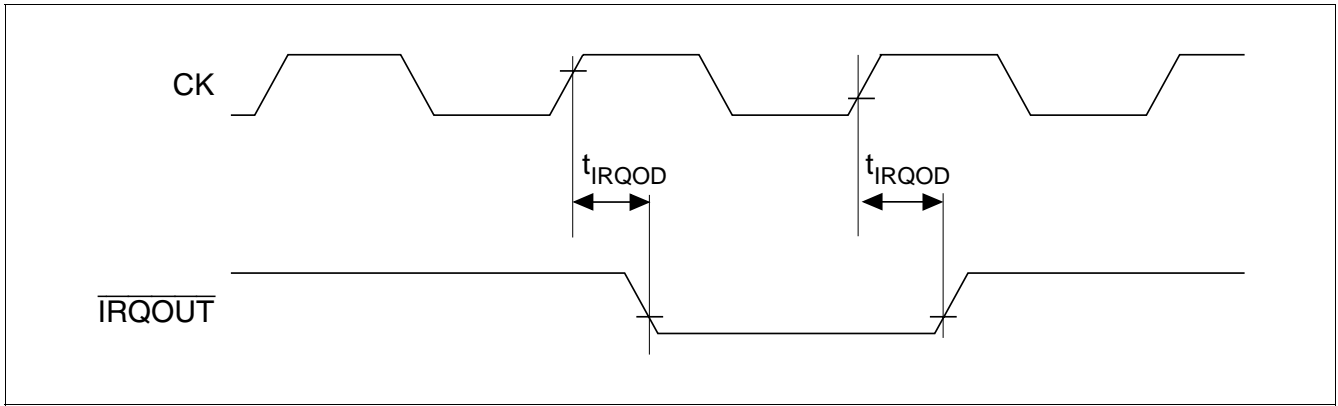
Figure 19.6 Interrupt Signal Output Timing
