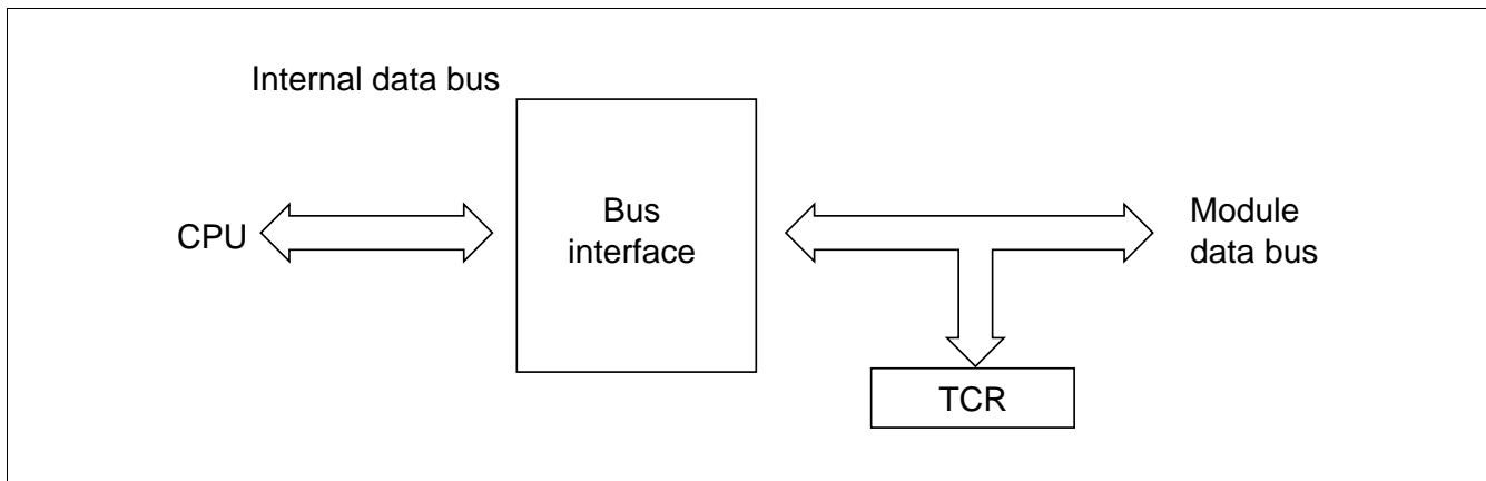
Figure 10.12 TCR Access (CPU-TCR)
