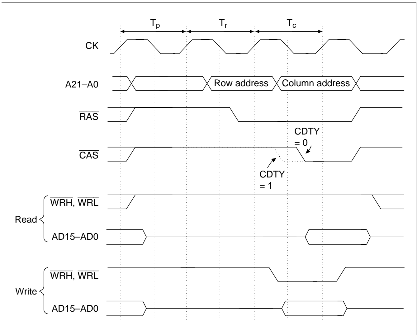
Figure 8.17 Short Pitch Access Timing
