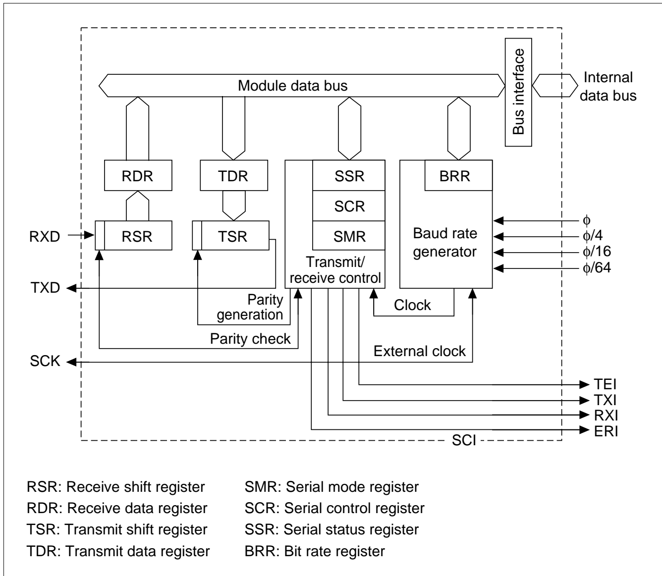
Figure 13.1 SCI Block Diagram
