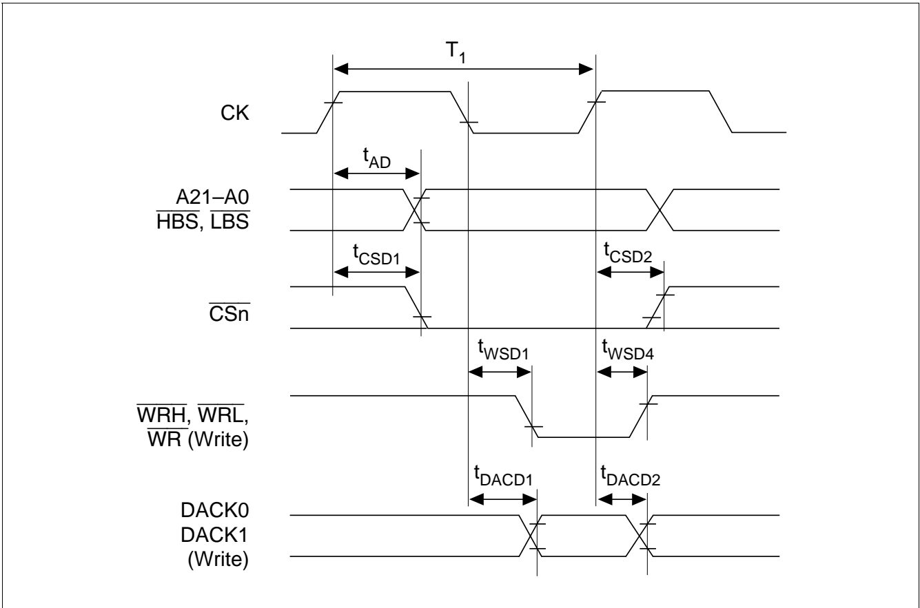
Figure 19.33 DMA Single Transfer/Single State Access Write
