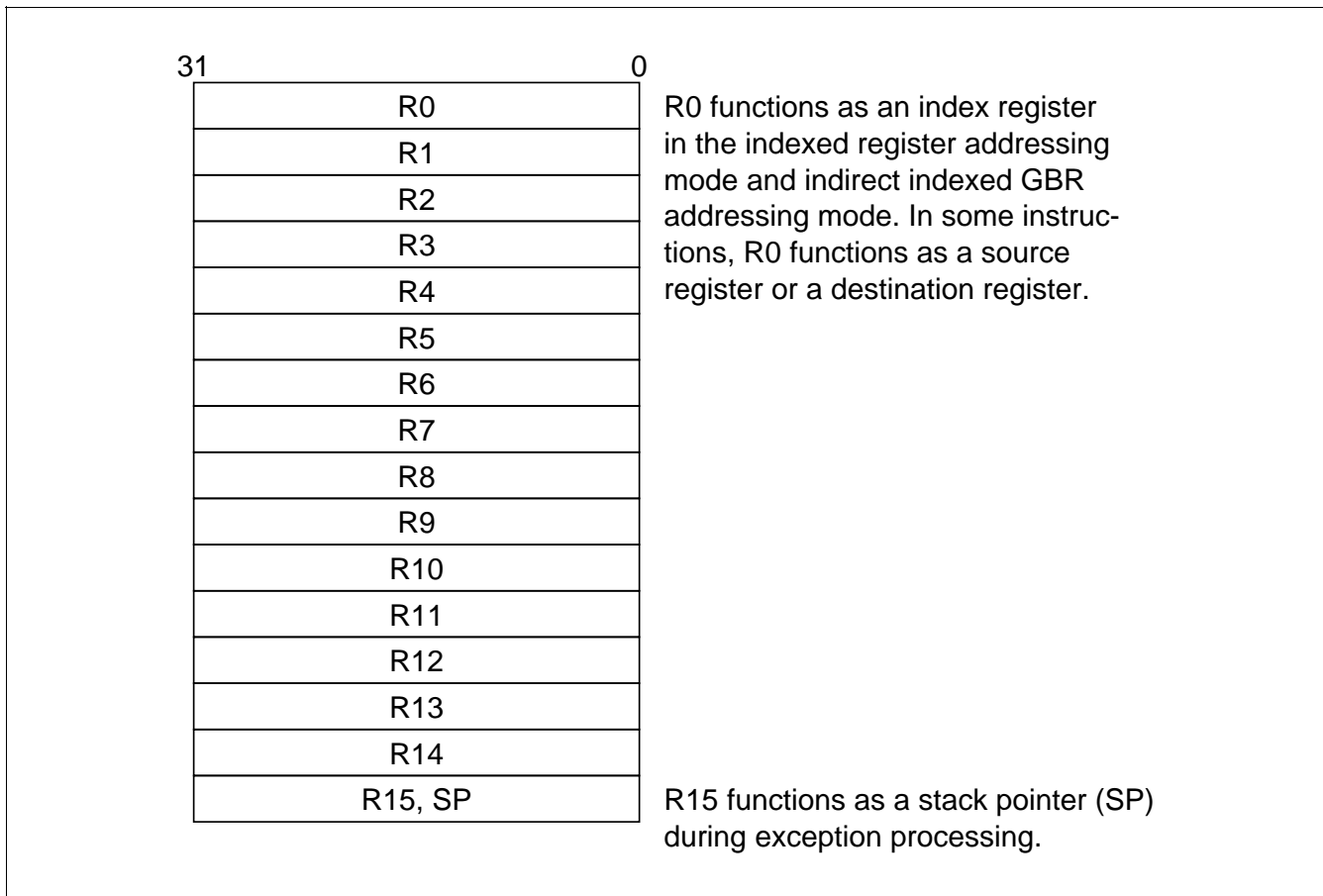
Figure 2.1 General Registers (Rn)
