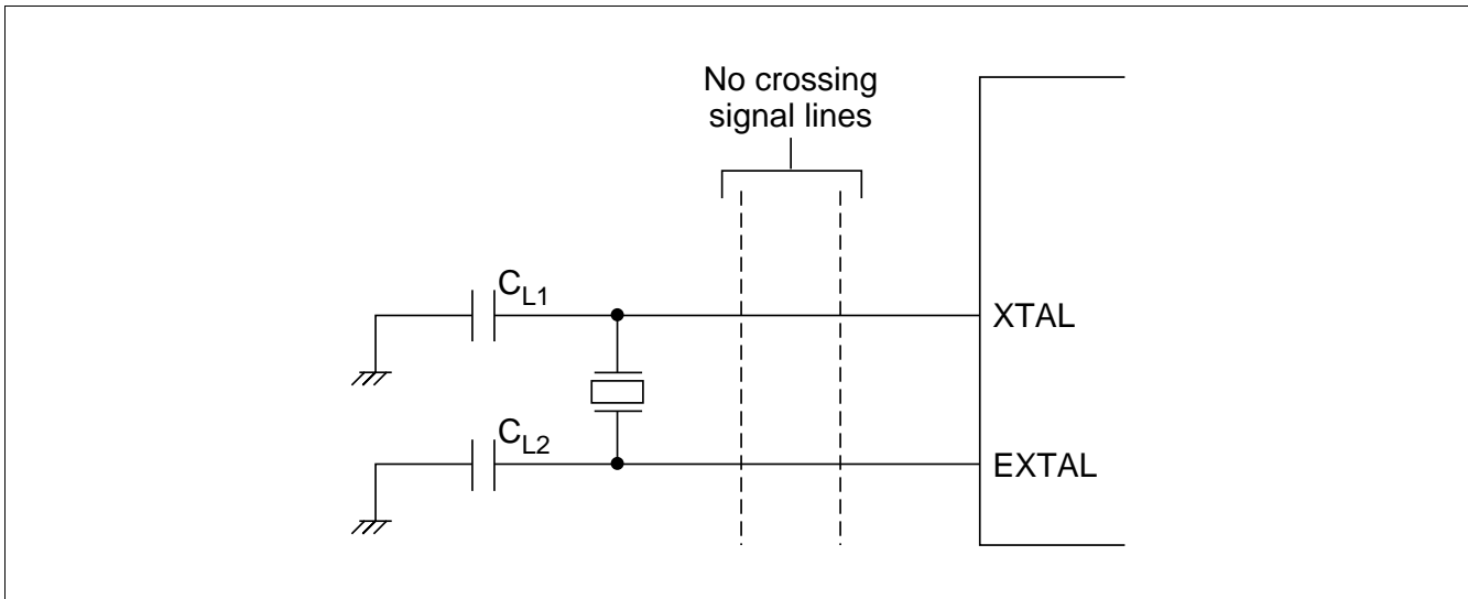
Figure 7.6 Precaution on Oscillator Circuit Board Design
