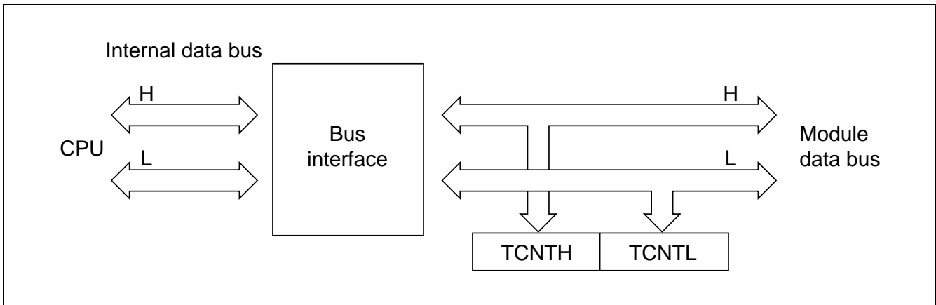
Figure 10.8 Accessing TCNT (CPU-TCNT (upper byte))
