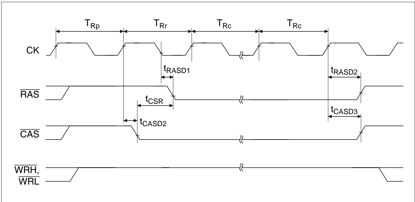
Figure 19.30 CAS-before-RAS Refresh (Long Pitch)
