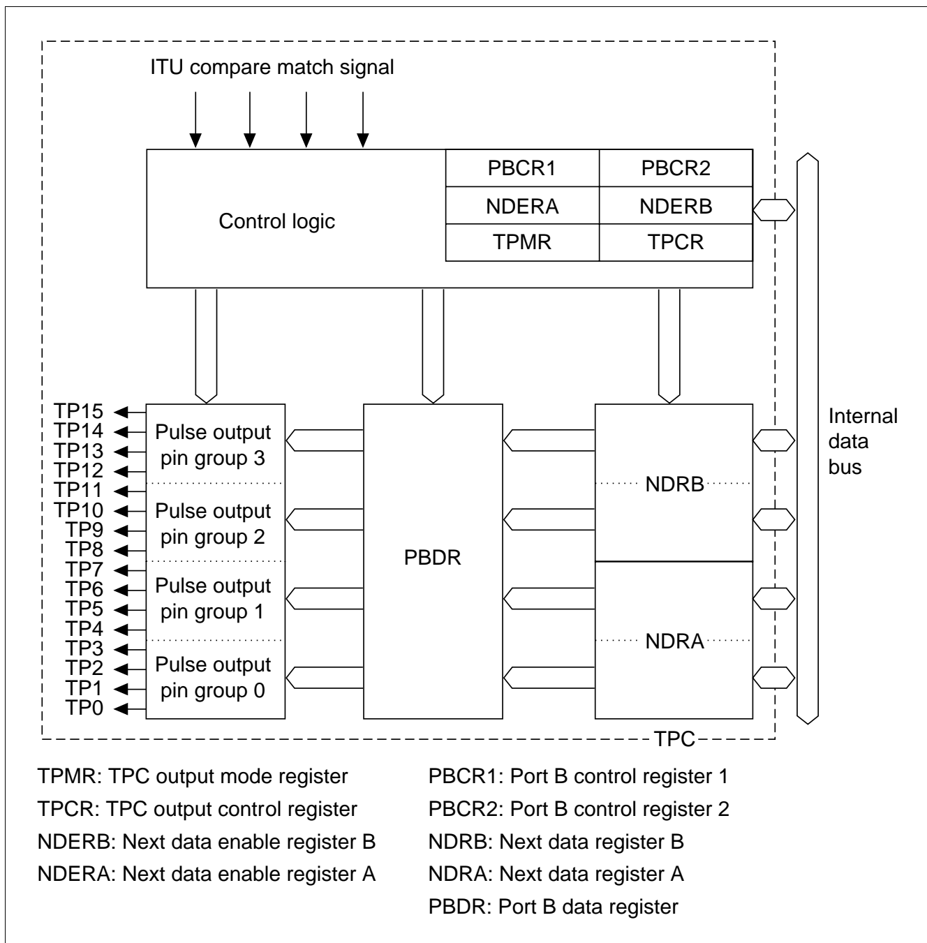
Figure 11.1 TPC Block Diagram
