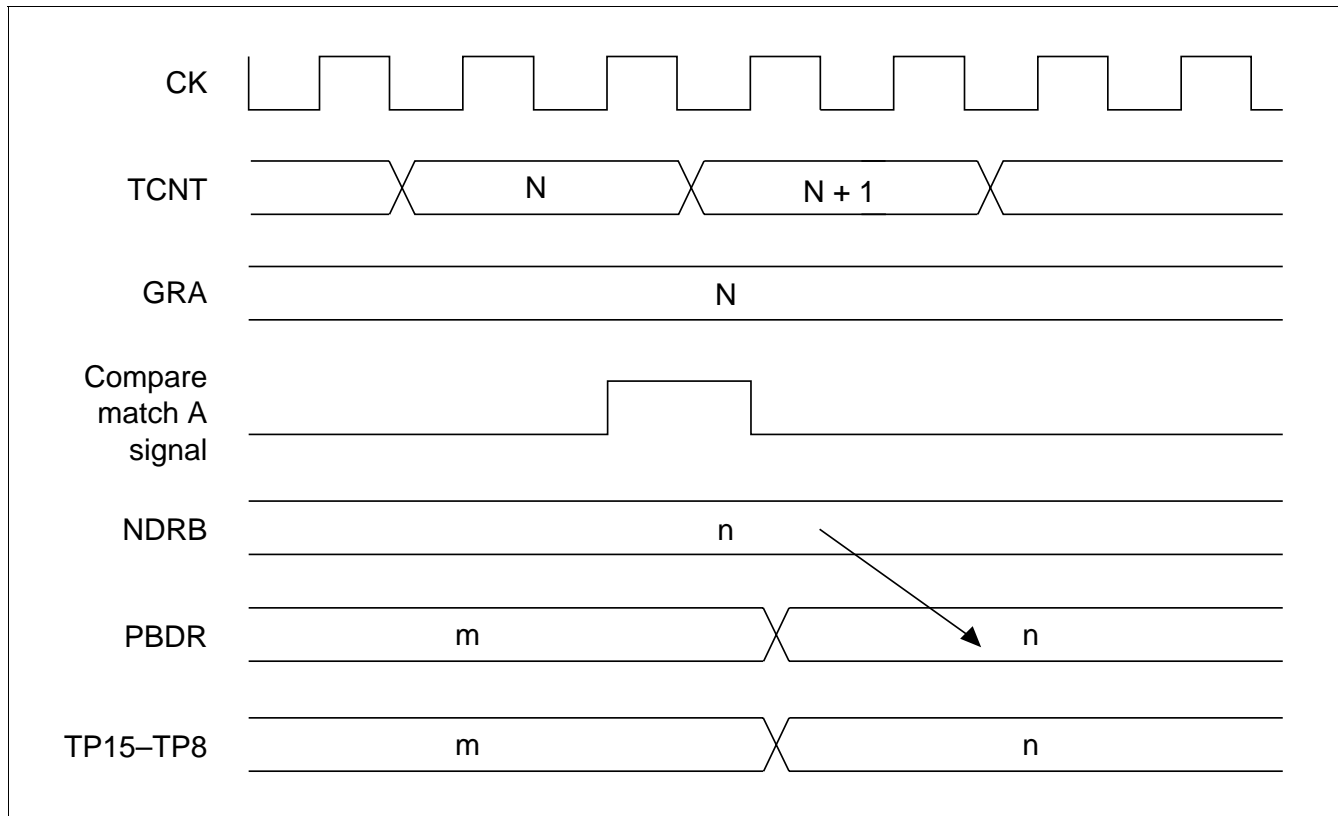
Figure 11.3 Transfer and Output Timing for NDR Data
