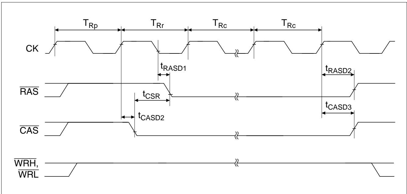
Figure 19.17 CAS-before-RAS Refresh (Long Pitch)
