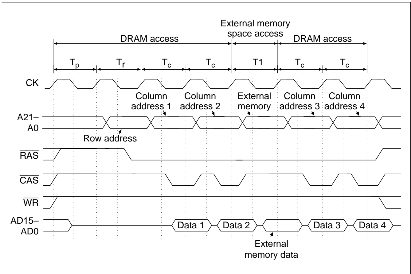
Figure 8.27 RAS Down Mode
