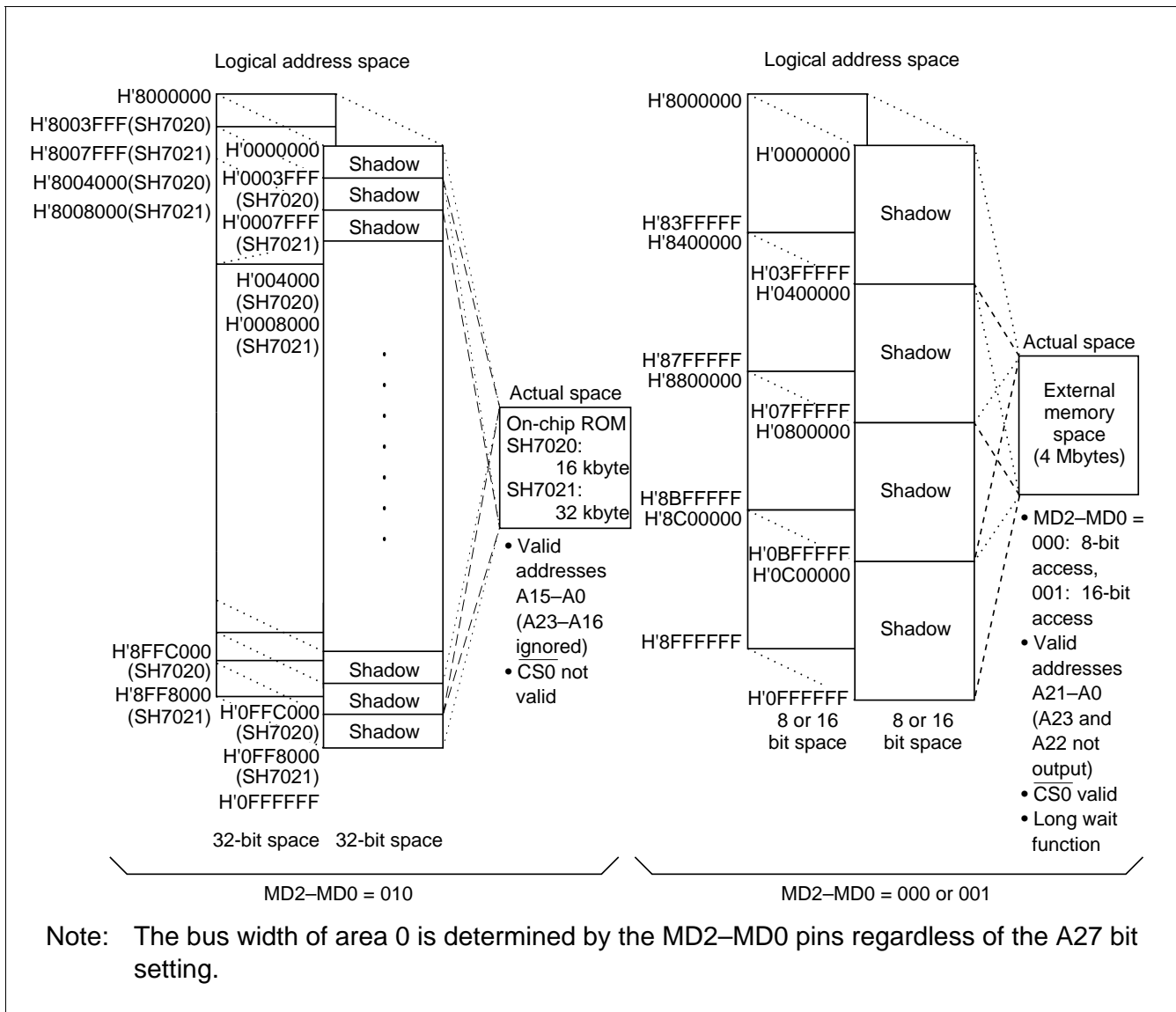
Figure 85 Memory Map of Area 0
