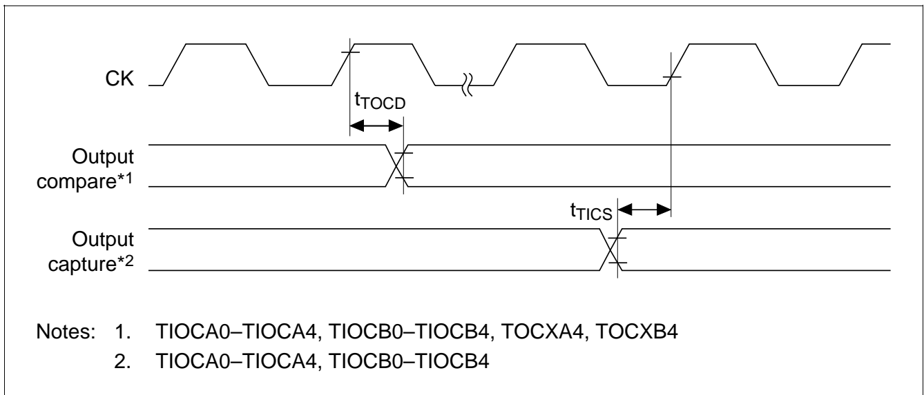
Figure 19.36 ITU Input/Output Timing
