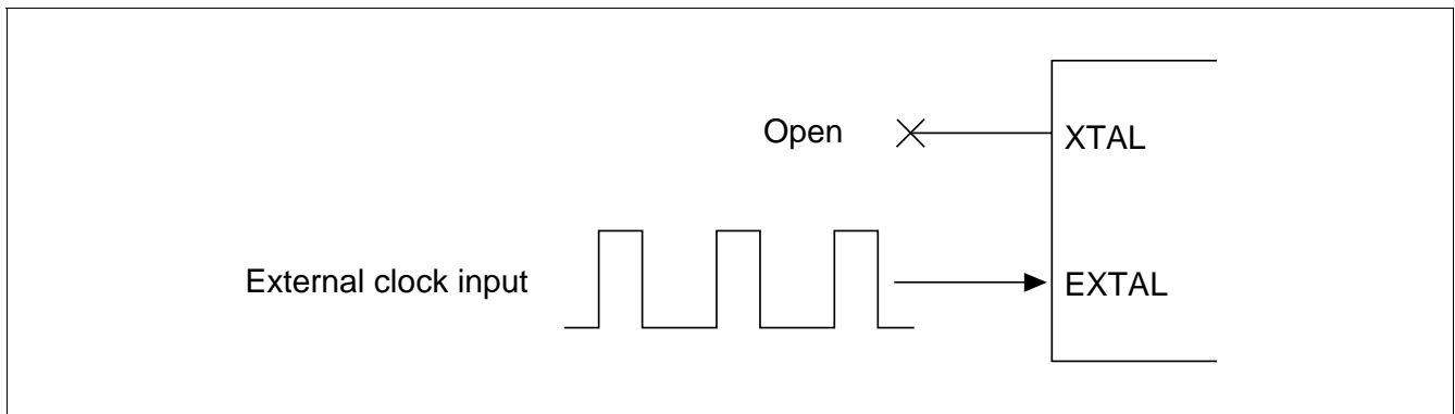
Figure 7.4 External Clock Input Method
