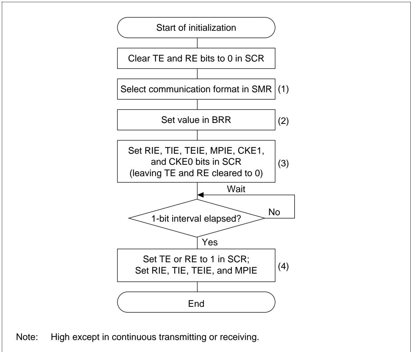
Figure 13.16 Sample Flowchart for SCI Initialization
