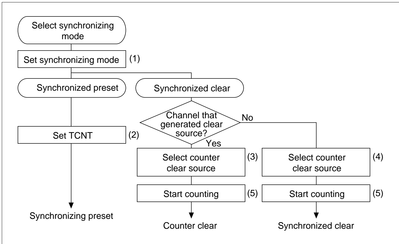
Figure 10.26 Procedure for Selecting the Synchronizing Mode
