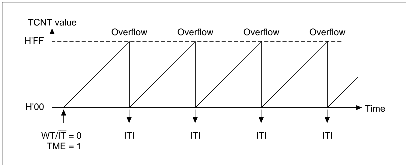
Figure 12.5 Operation in the Interval Timer Mode
