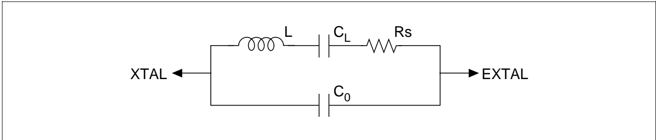
Figure 7.3 Crystal Resonator Equivalent Circuit
