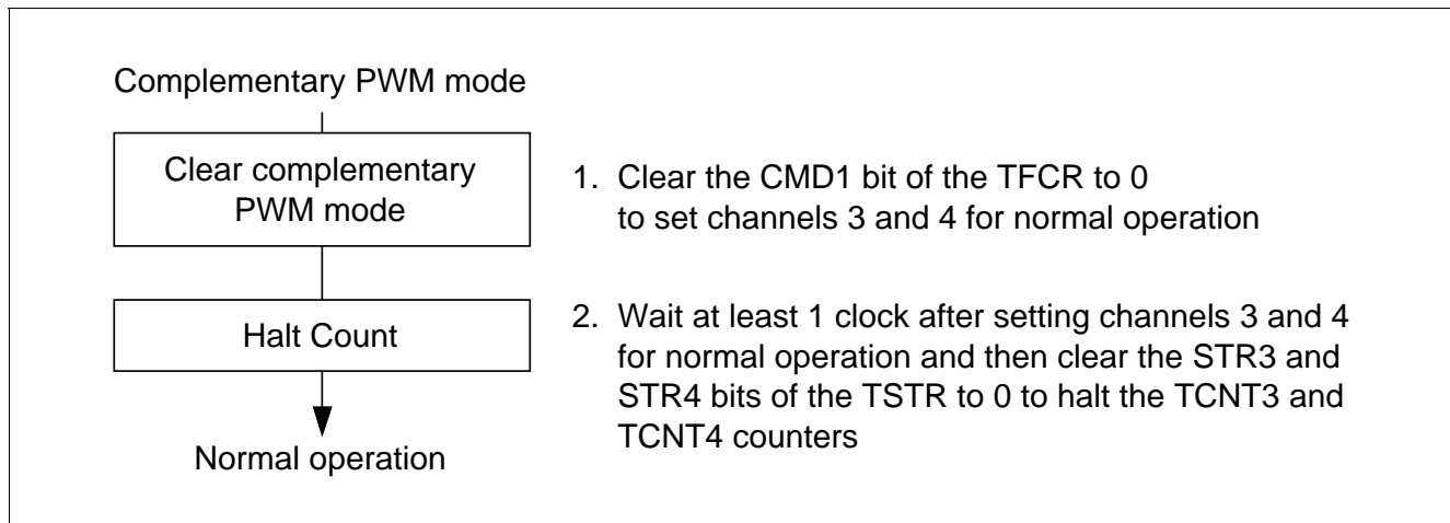
Figure 10.69 Clearing the Complementary PWM Mode
