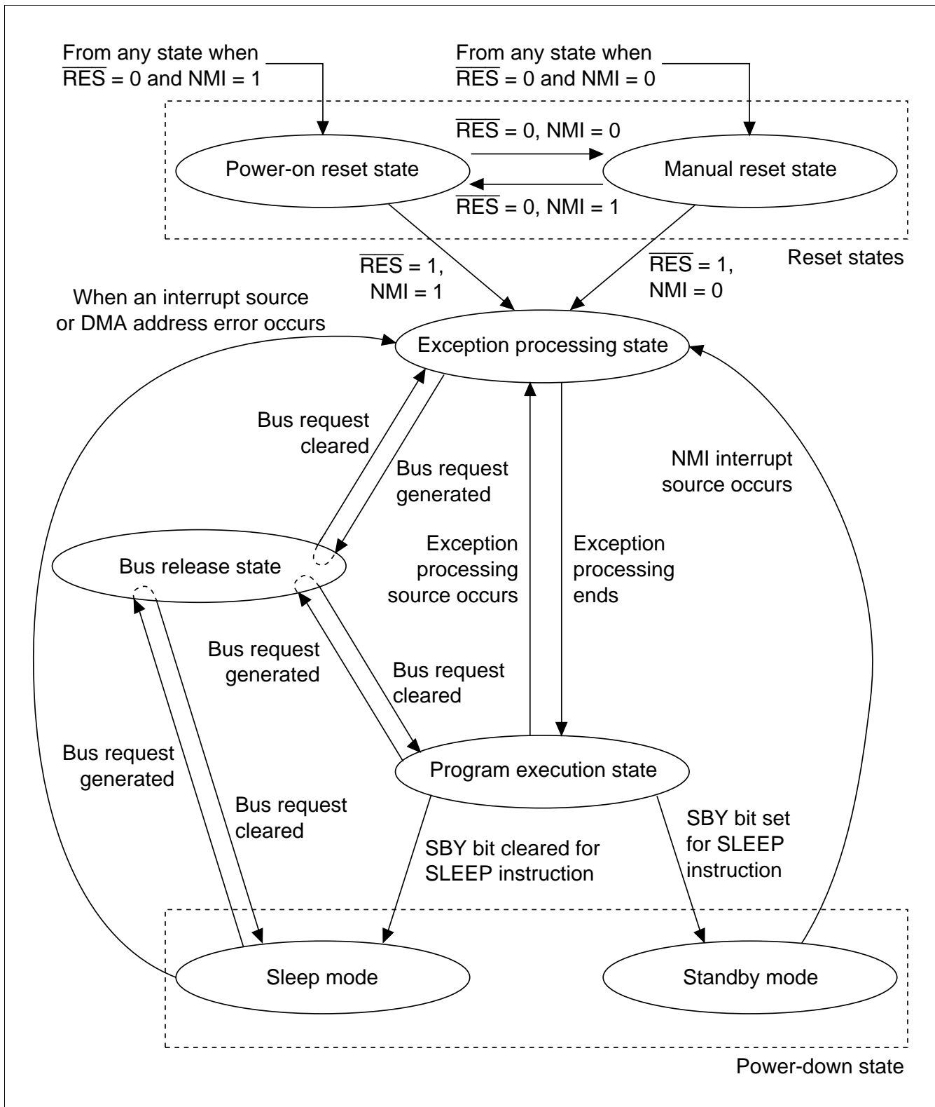
Figure 2.6 Transitions Between Processing States
