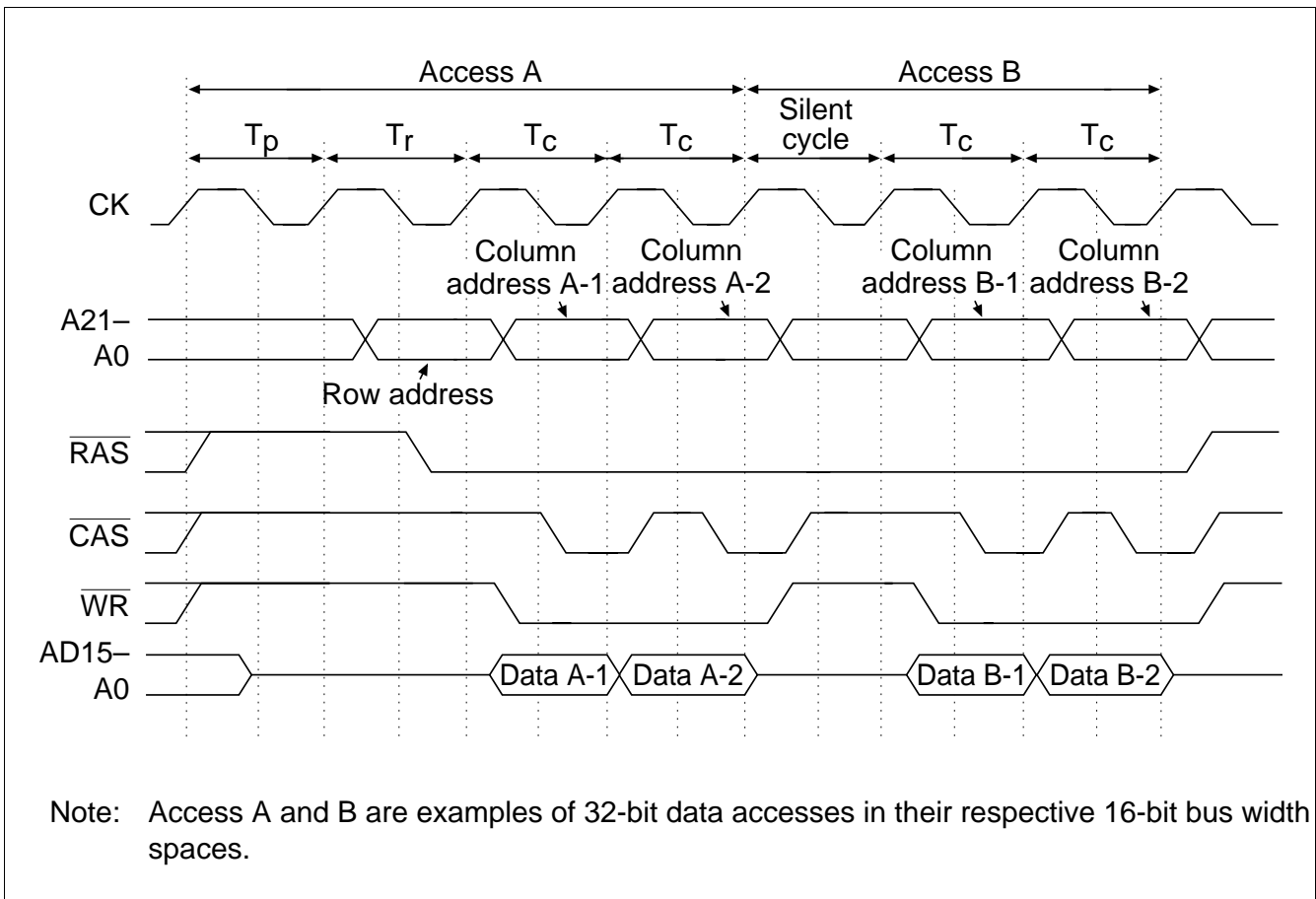
Figure 8.24 Short Pitch High-Speed Page Mode (Write Cycle)
