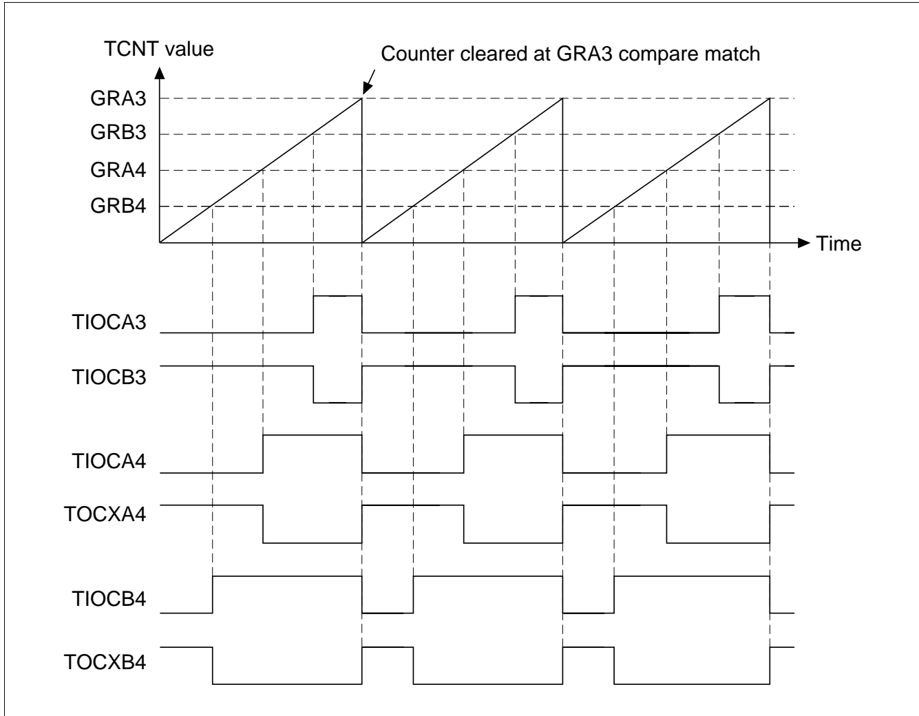
Figure 10.32 Reset-Synchronized PWM Mode Operation Example 1
