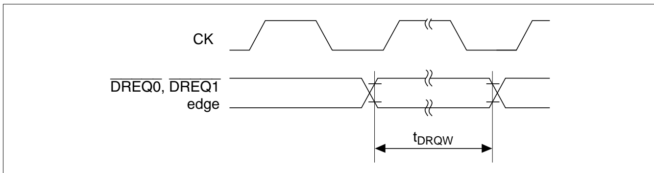
Figure 19.35 \overline{\text{DREQ0}}, \overline{\text{DREQ1}} Input Timing (2)
