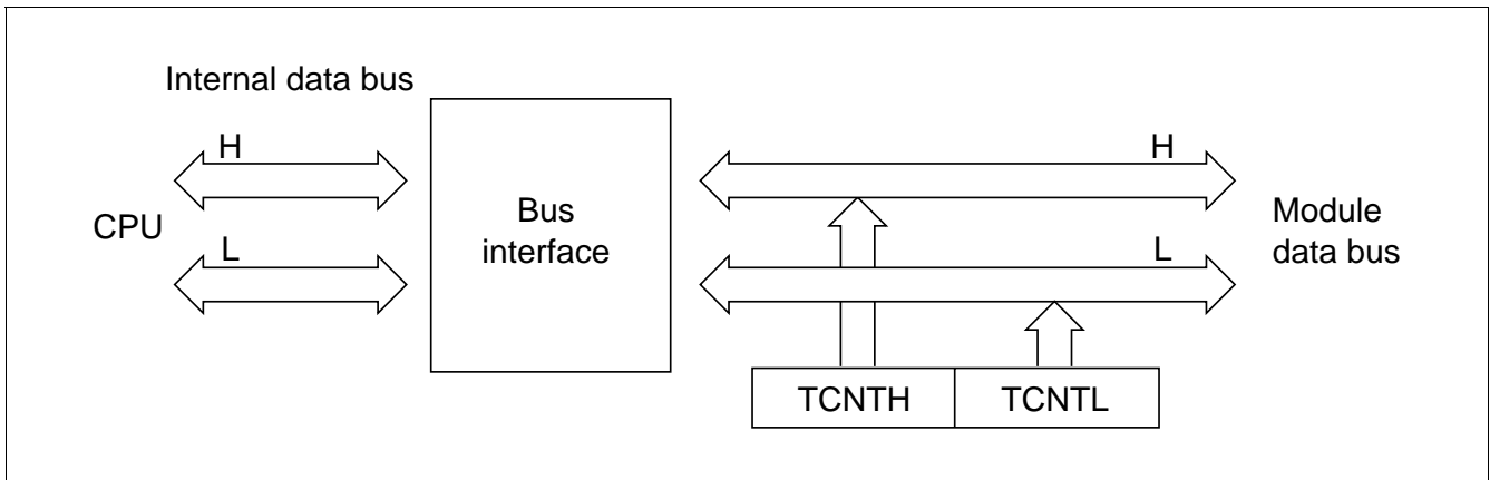
Figure 10.11 Accessing TCNT (TCNT–CPU (lower byte))
