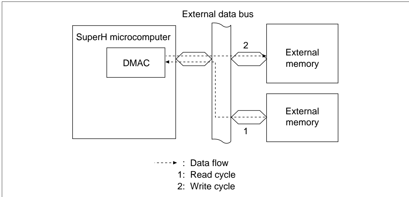
Figure 9.8 Data Flow in Dual Address Mode
