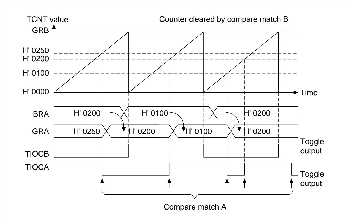
Figure 10.48 Buffer Mode Operation Example 1 (Output Compare Register)
