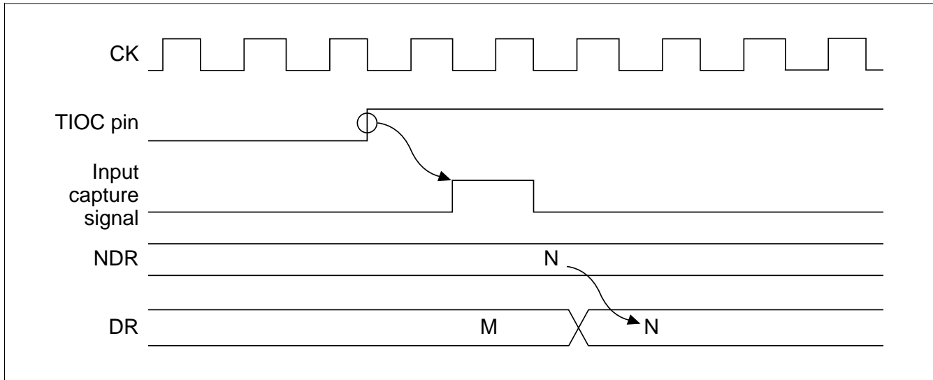
Figure 11.8 TPC Output by Input Capture
