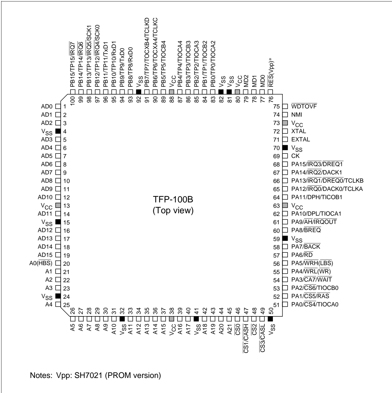
Figure 1.2 Pin Arrangement
