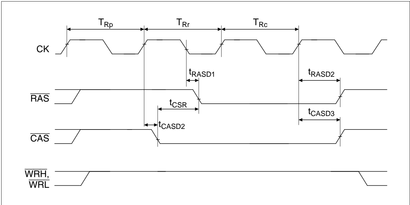
Figure 19.29 CAS-before-RAS Refresh (Short Pitch)
