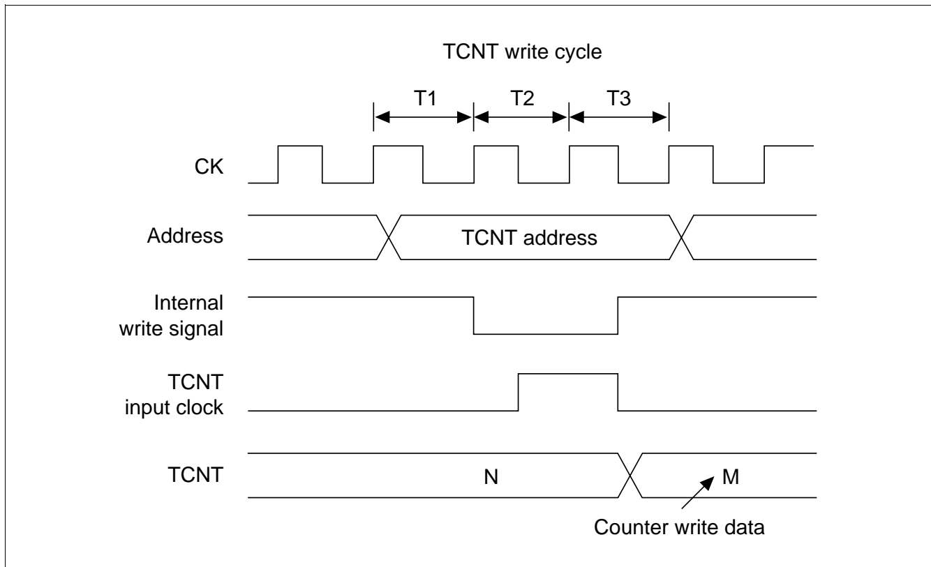
Figure 12.8 Contention between TCNT Write and Increment
