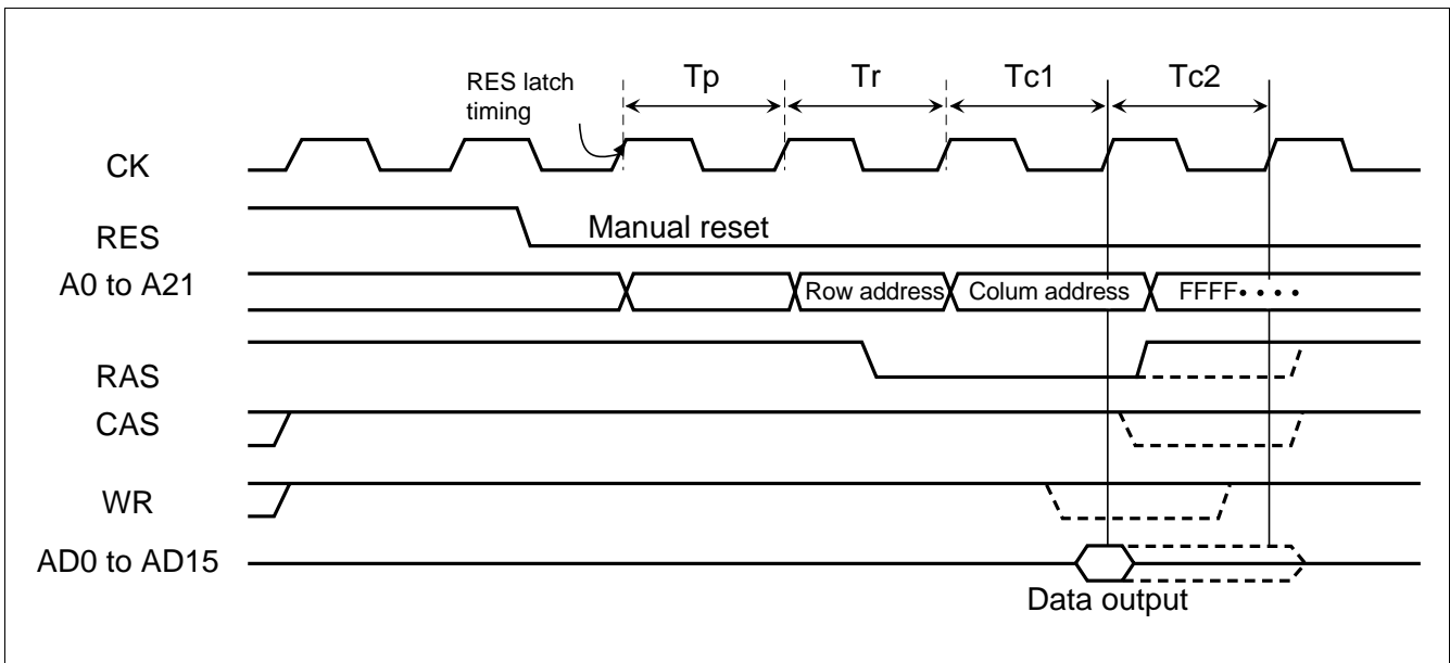
Figure 8.38 Long - pitch Mode Write (1)
