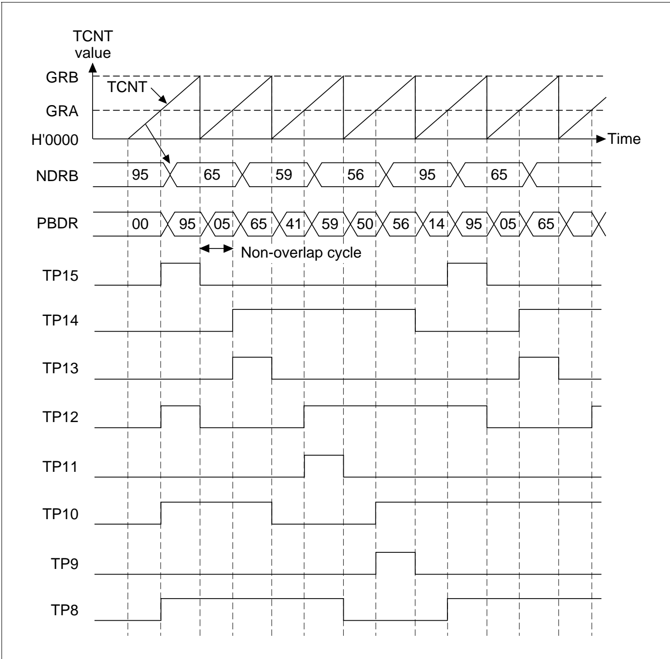
Figure 11.7 Non-Overlap Output Example (Four-Phase Complementary Output)
