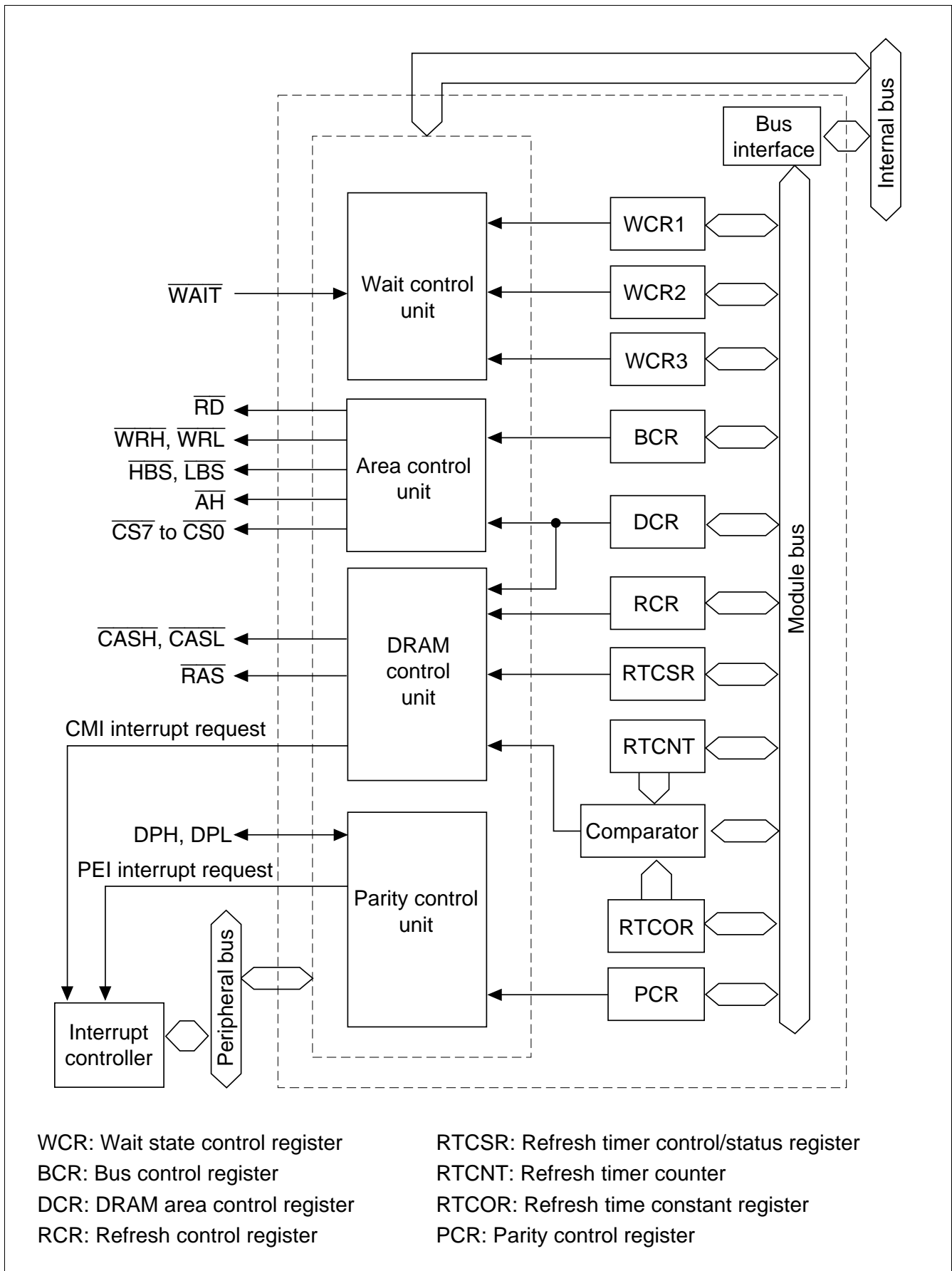
Figure 8.1 BSC Block Diagram
