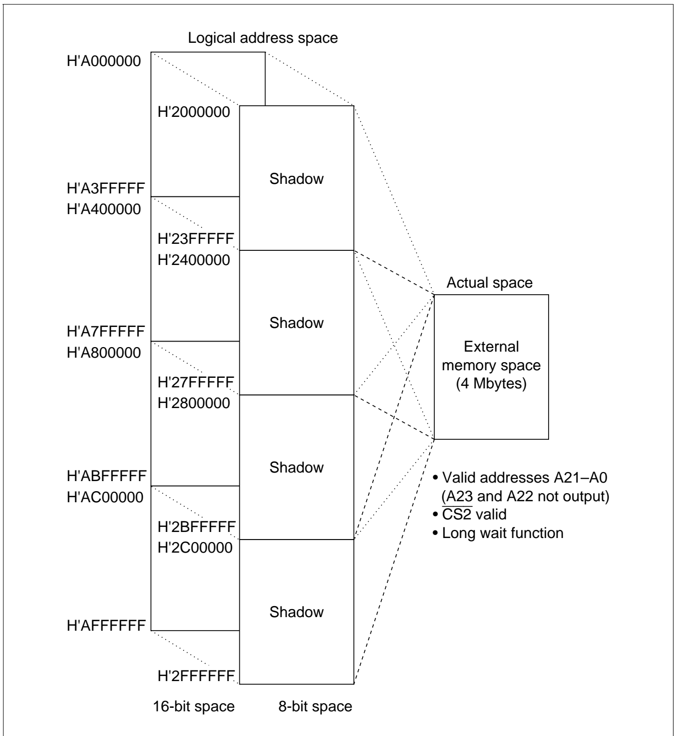
Figure 8.7 Memory Map of Area 2
