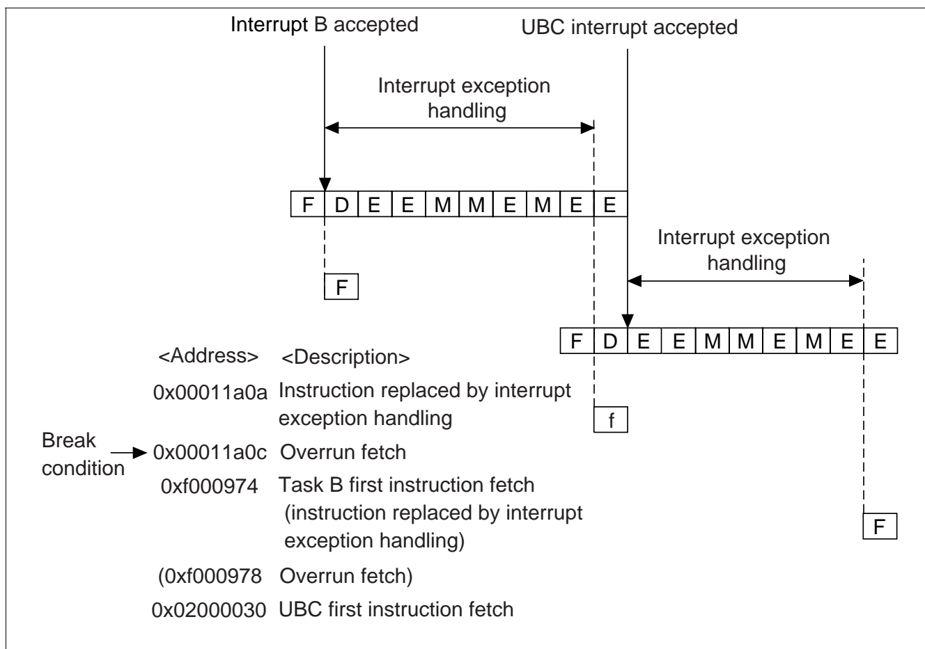
Figure 6.3 UBC Operation
