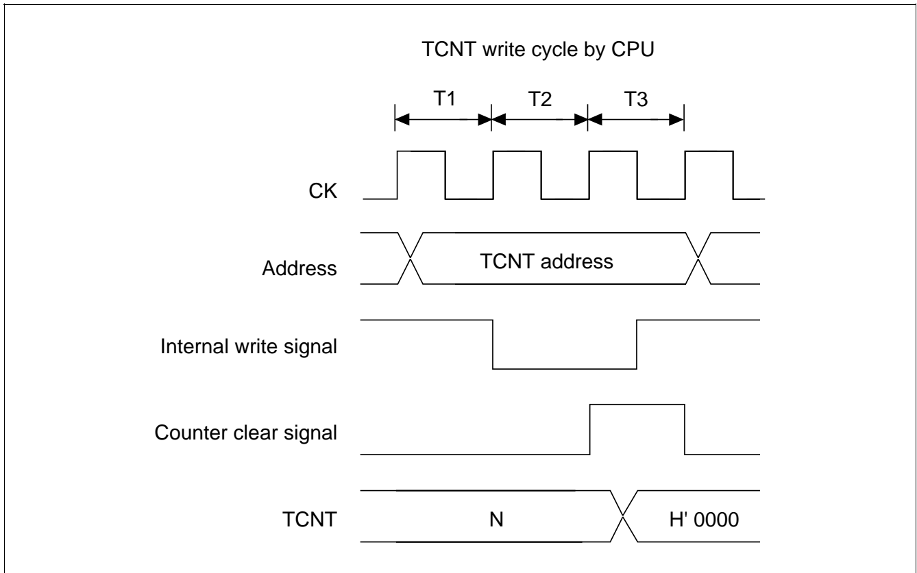
Figure 10.58 Contention between TCNT Write and Clear
