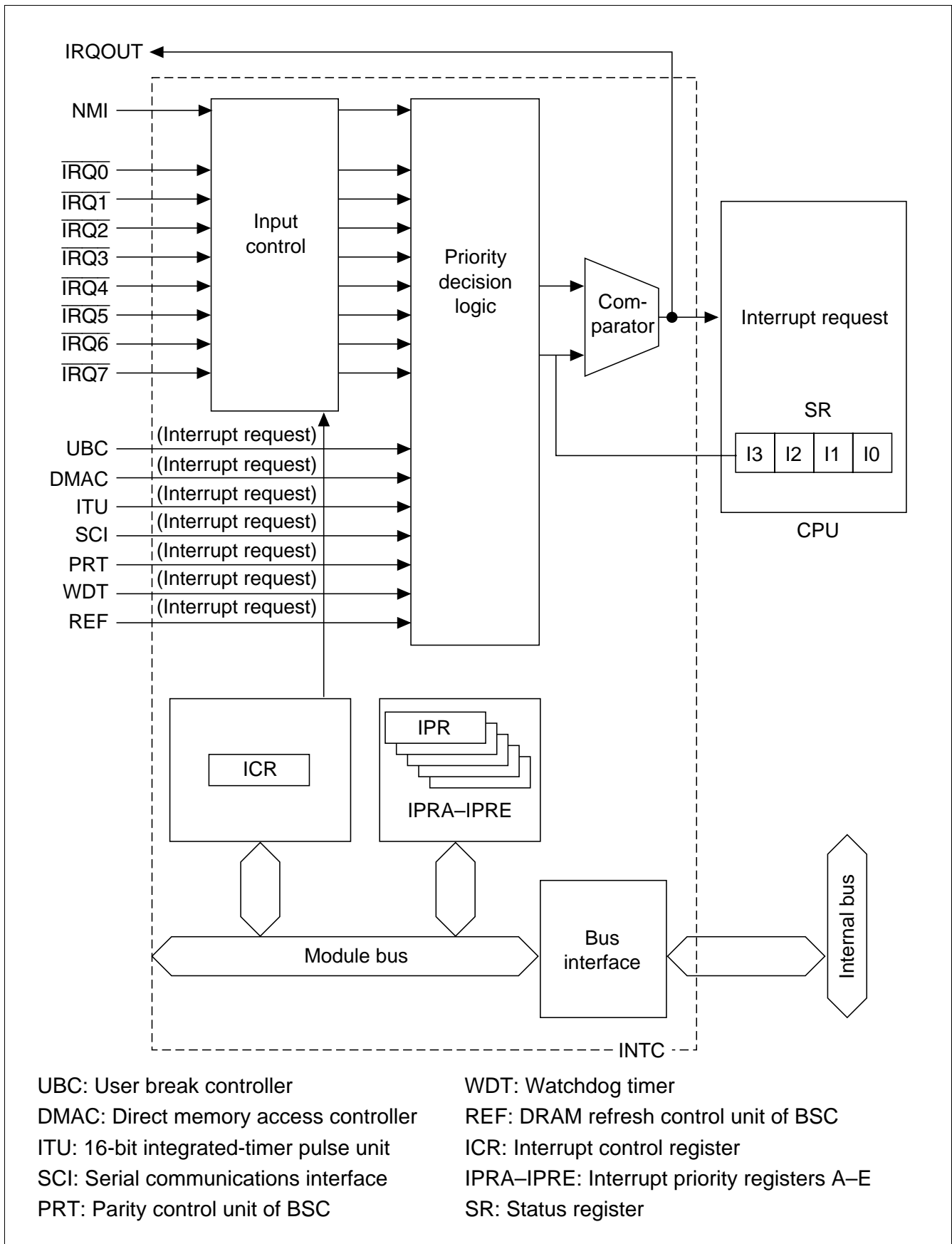
Figure 5.1 Block Diagram of the Interrupt Controller
