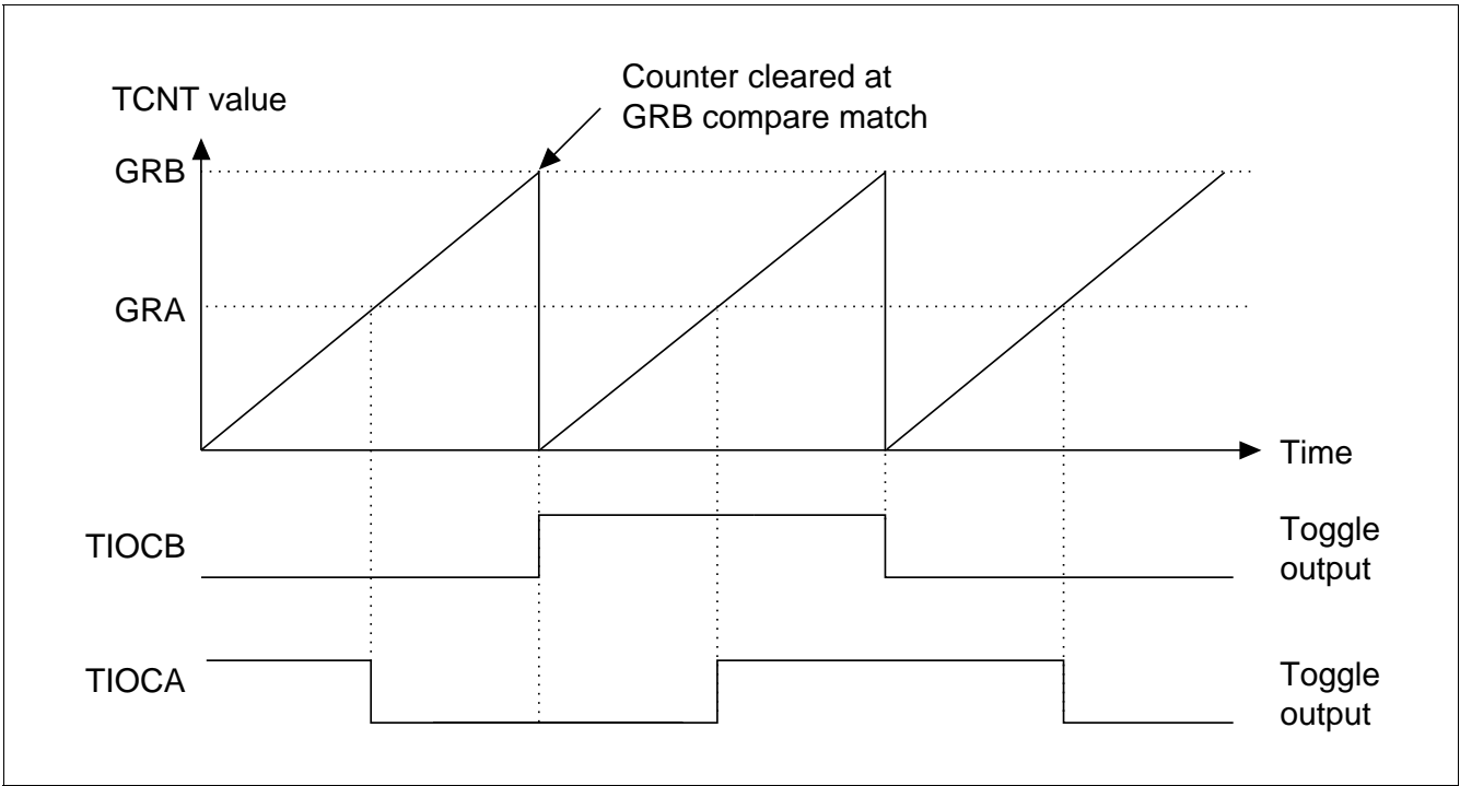
Figure 10.21 Example of Toggle Output
