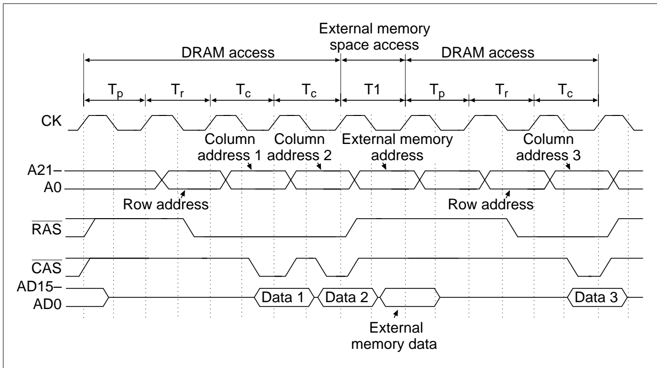
Figure 8.28 RAS Up Mode
