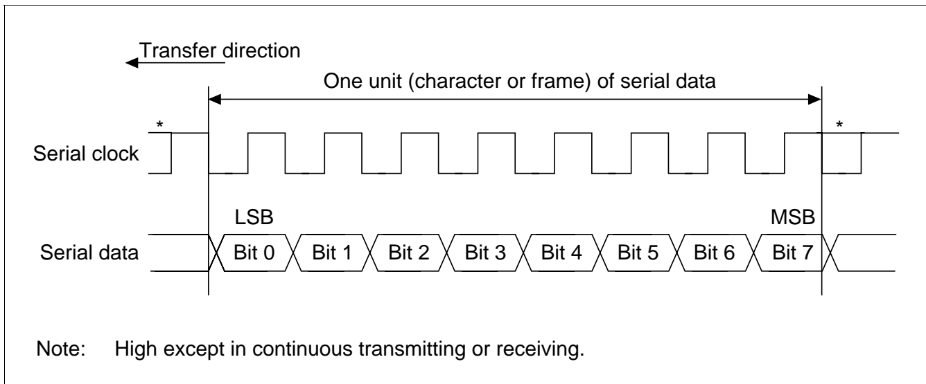
Figure 13.14 Data Format in Clocked Synchronous Communication
