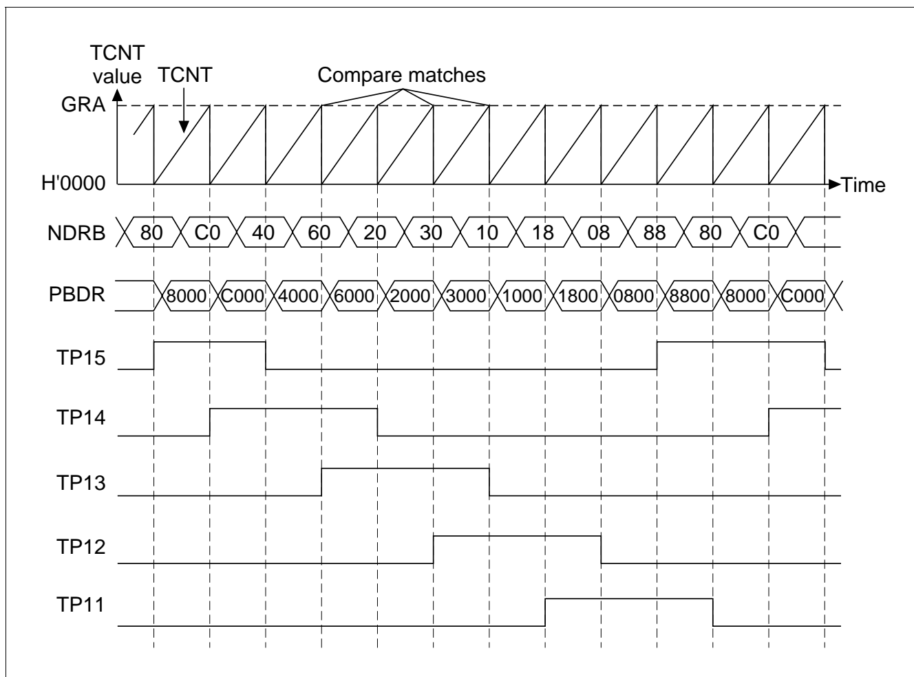
Figure 11.5 TPC Output Example (5-Phase Pulse Output)
