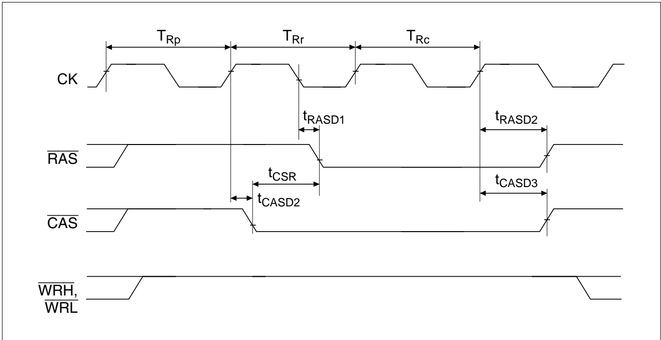
Figure 19.16 CAS-before-RAS Refresh (Short Pitch)
