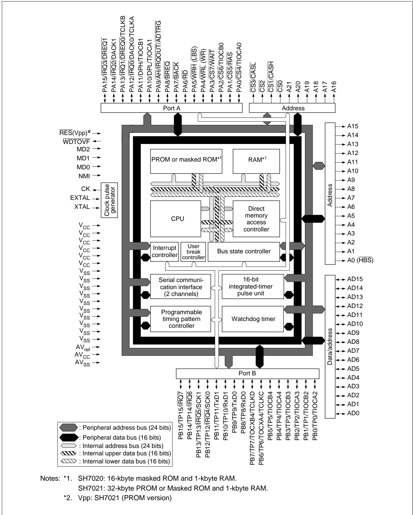
Figure 1.1 Block Diagram
