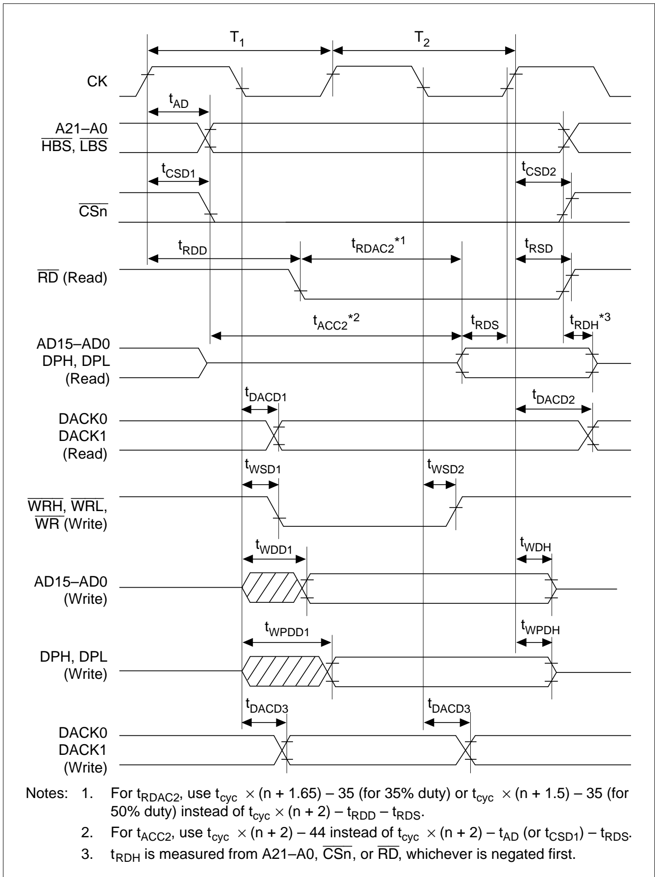
Figure 19.22 Basic Bus Cycle: Two-State Access
