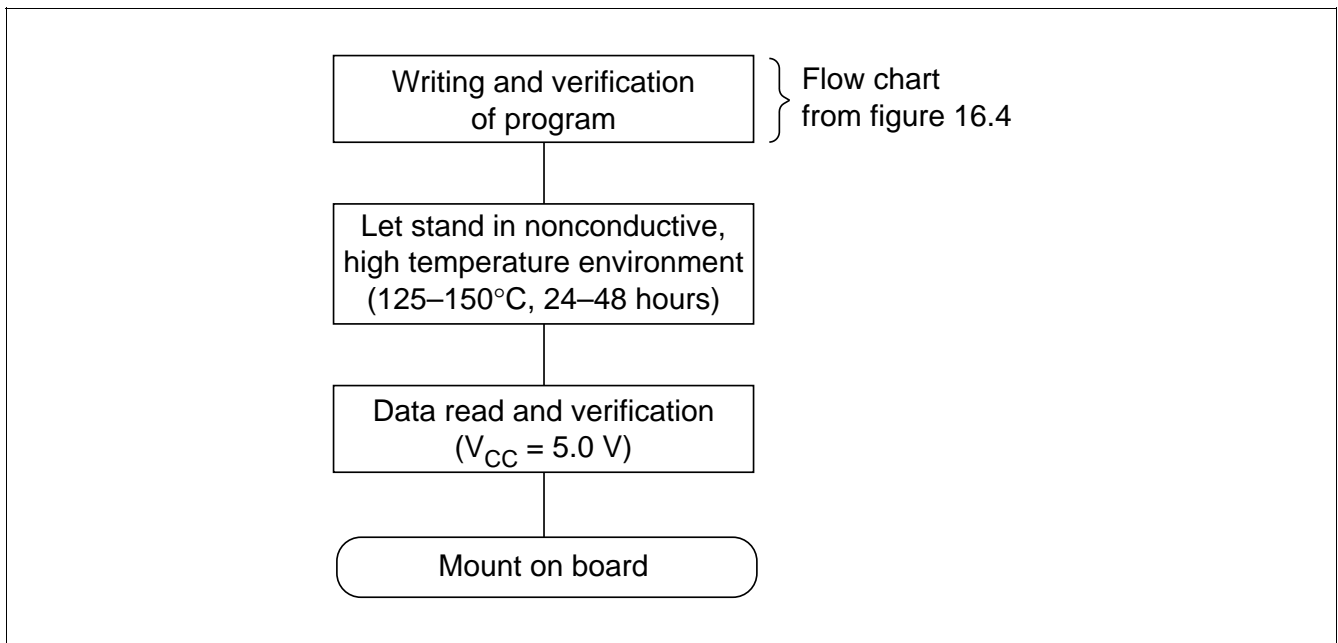
Figure 16.6 Screening Flow
