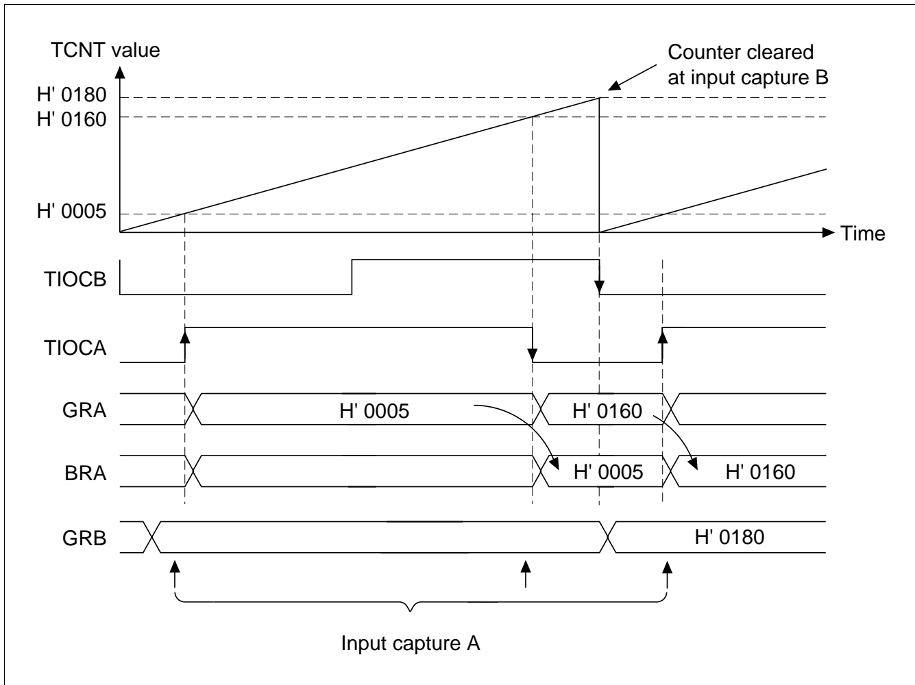
Figure 10.50 Buffer Mode Operation Example 2 (Input Capture Register)
