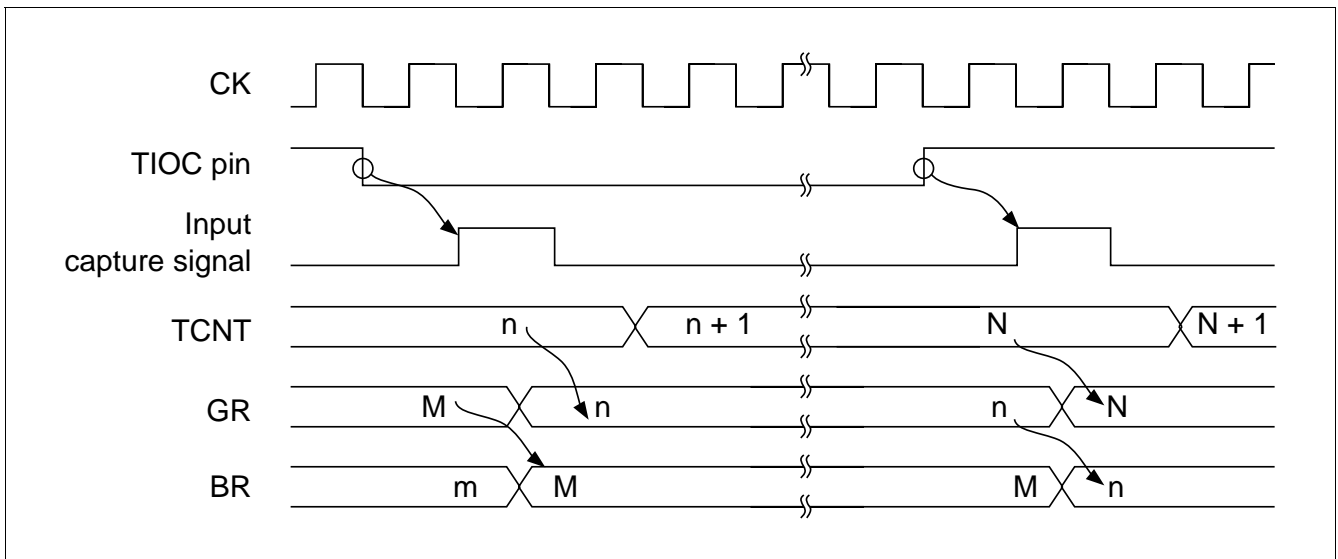
Figure 10.51 Input Capture Timing Example for Buffer Operation
