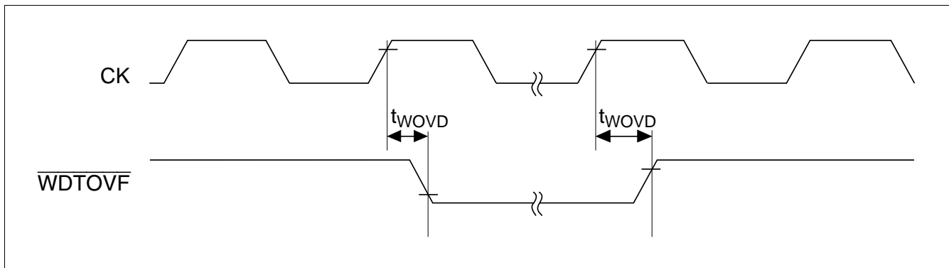
Figure 19.39 Watchdog Timer Output Timing
