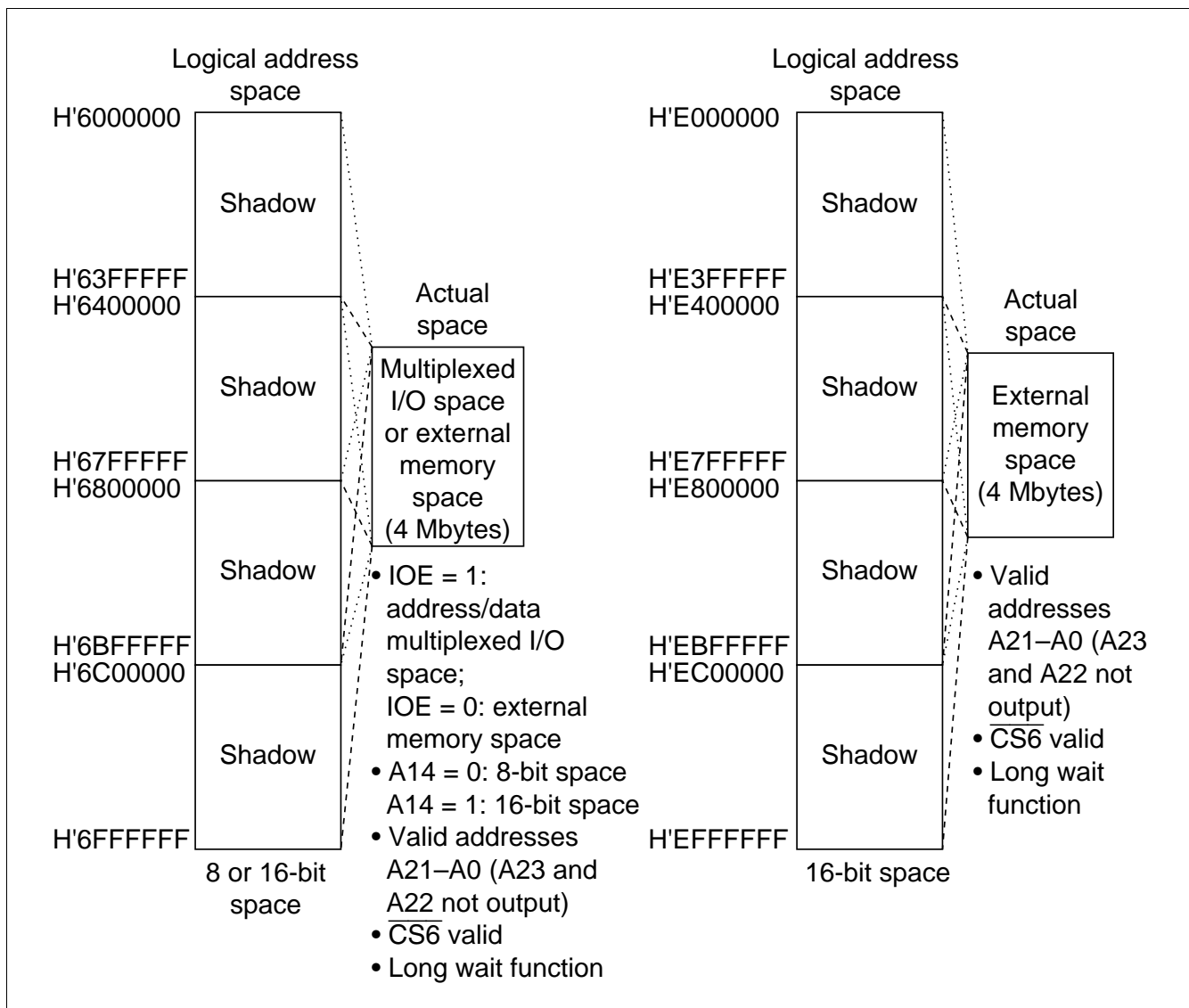
Figure 8.9 Memory Map of Area 6
