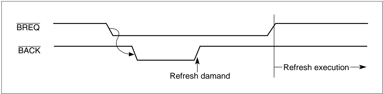
Figure 8.36 \overline{\text{BACK}} Operation by Refresh Demand (1)
