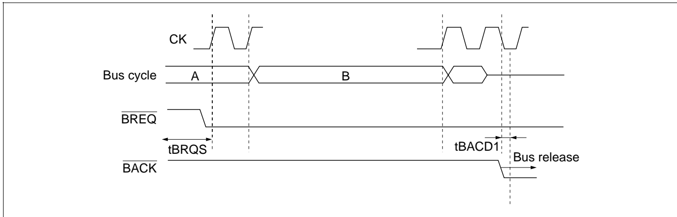
Figure 8.43 When \overline{\text{BREQ}} is Input without Satisfying t_{\text{BRQS}}
