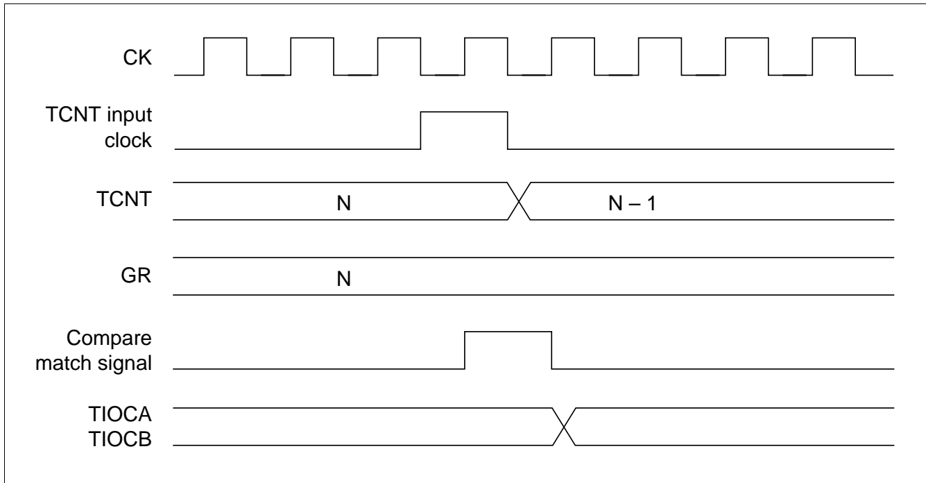
Figure 10.22 Compare Match Signal Output Timing
