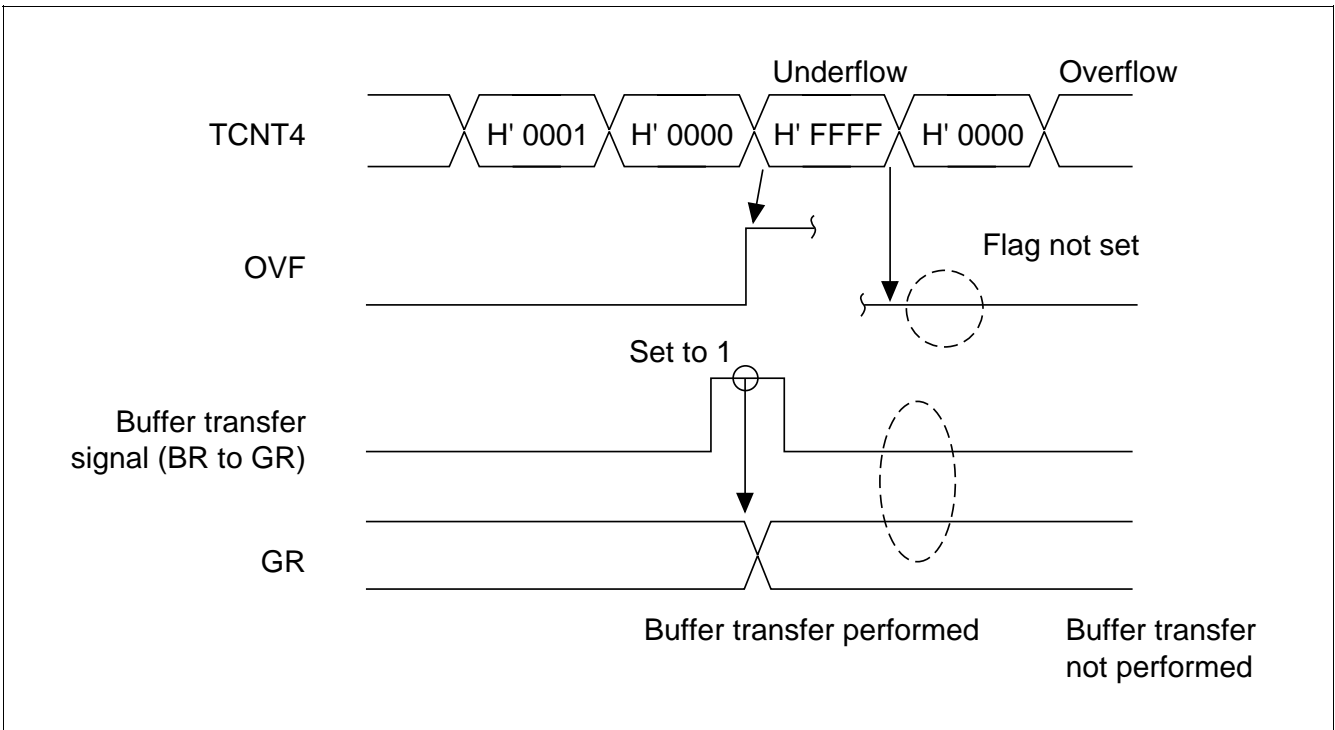
Figure 10.37 Undershoot Timing
