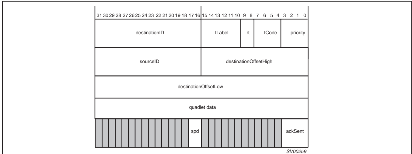
Figure 16. Quadlet Write Request Receive Format
