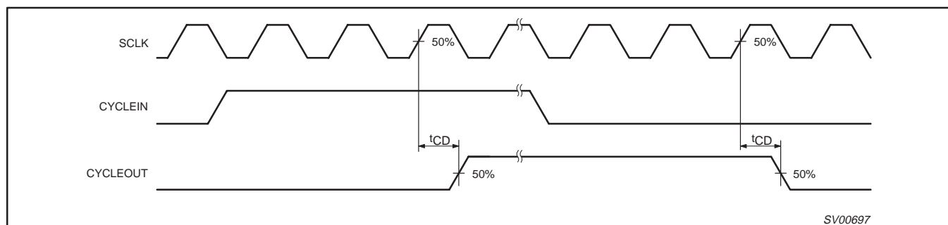
Figure 32. CYCLEOUT Waveforms
