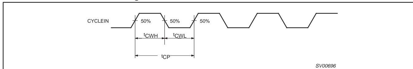
Figure 31. CYCLEIN Waveform
