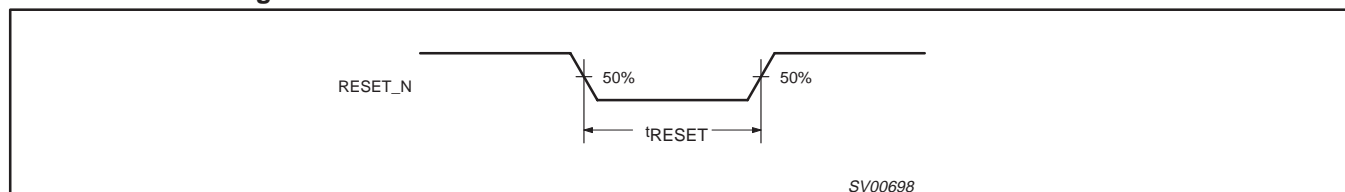
Figure 33. RESET_N Waveform
