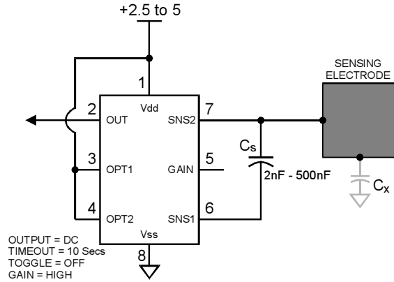
Figure 1-1 Standard mode options
