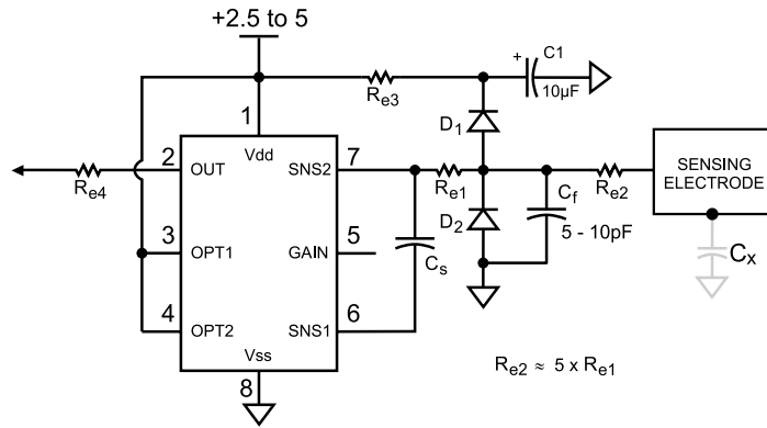
Figure 2-7 ESD Protection
