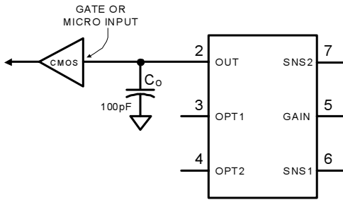
Figure 2-5 Eliminating HB Pulses
