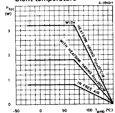
Fig. 5 - Maximum allowable power dissipation vs. ambient temperature
