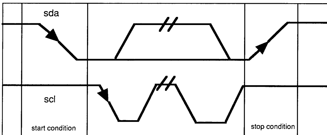
Figure 17. Start/Stop conditions
