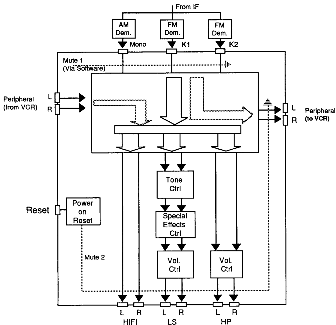
Figure 15. Input/Output Combinations
