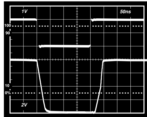
Figure 45. 6 dB Overload Recovery, G = +10 , ( R_L = 500 \Omega , R_F = 357 \Omega , V_S = \pm 5 V )
