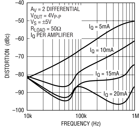
LT1795 G18
