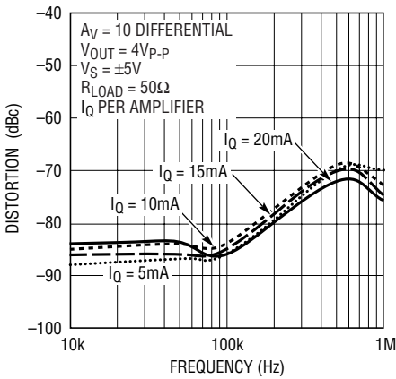
LT1795 G19
