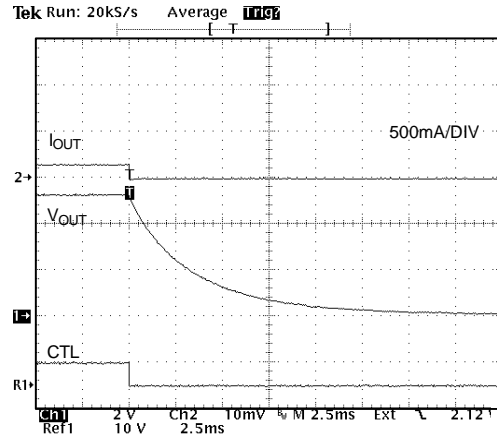
Turn Off Falling Time (35Ω, 100uF Loading)
