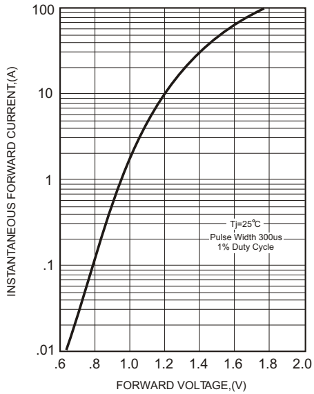
FIG.1-TYPICAL FORWARD CHARACTERISTICS
