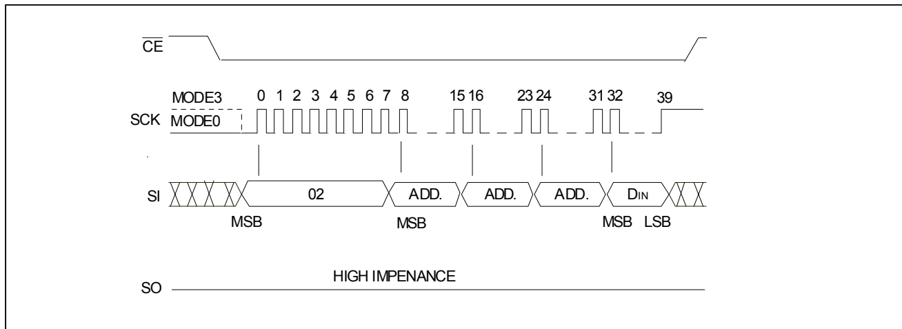
Figure 4 : BYTE-PROGRAM SEQUENCE
