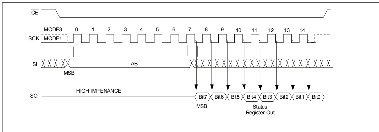
Figure 16 : Read-Electronic-Signature (RES)
