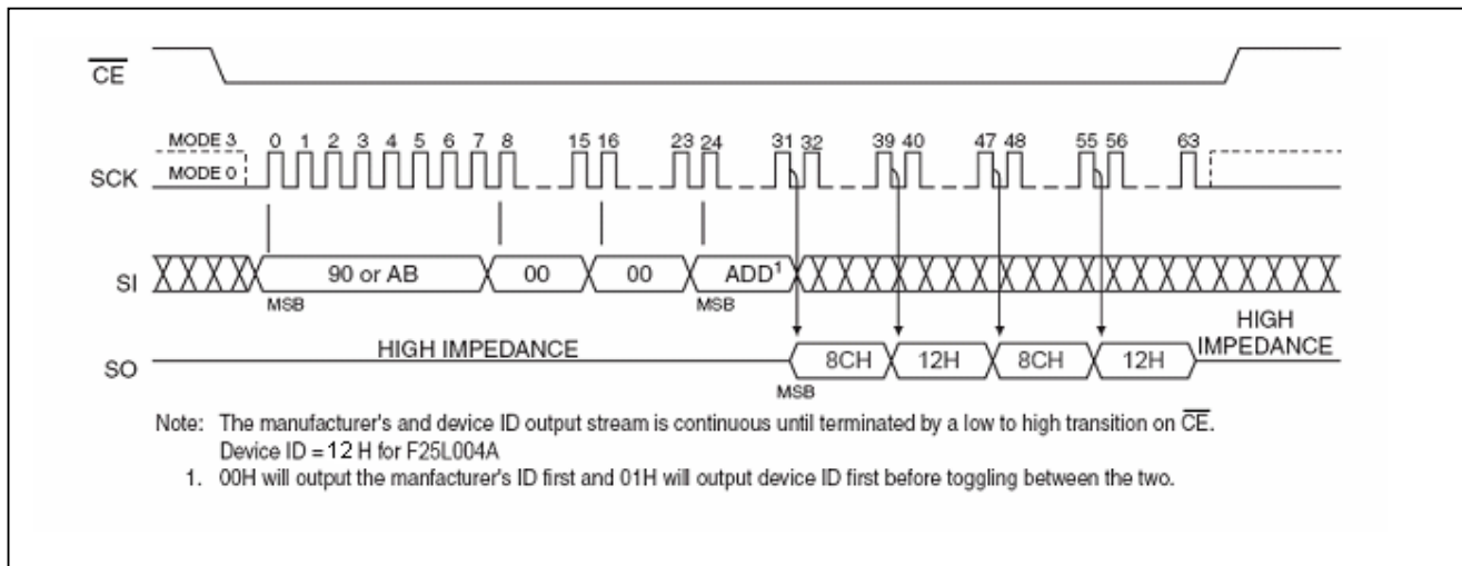
Figure 18 : Read-Electronic-Signature
