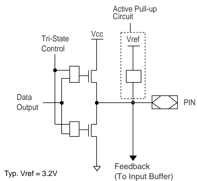
Typical Output
