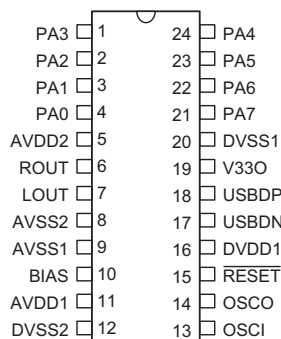
HT82A821R - 24 SSOP-A/SOP-A
