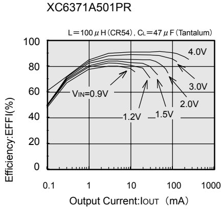
(2) Efficiency vs. Output Current
