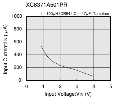
(4) NO LOAD, INPUT CURRENT vs. INPUT VOLTAGE
