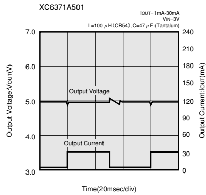
(6) LOAD TRANSIENT RESPONSE
