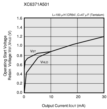
(5) OPERATING START VOLTAGE/RETAIN VOLTAGE vs. OUTPUT CURRENT
