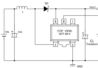
Fig.3 XC6371C Application
