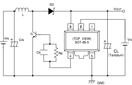
Fig.4 XC6371D Application
