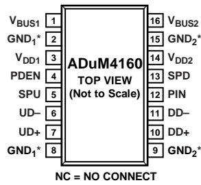
Figure 3. Pin Configuration
