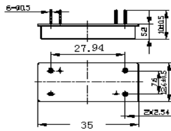
Package Outline
