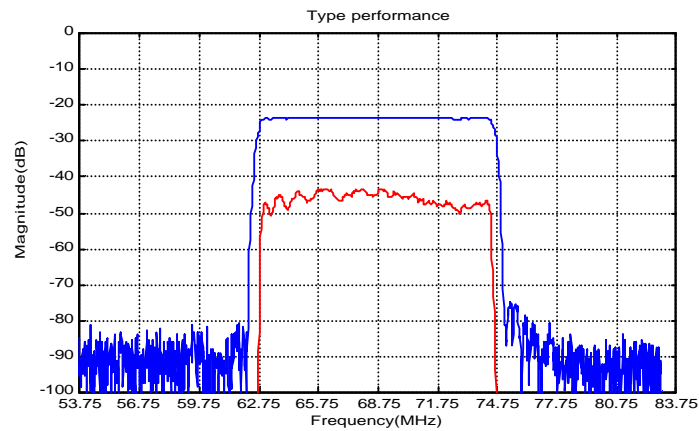
SP68B11 SAW Filter Typical Performance
