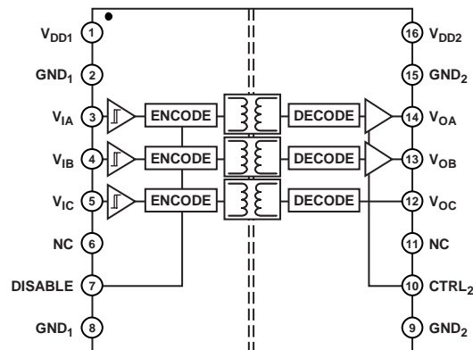
Figure 1. ADuM1310
