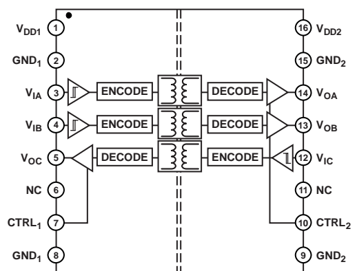
Figure 2. ADuM1311
