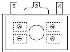
SOT-89-5 (TOP VIEW)
