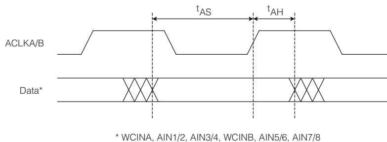
Figure 2-3: Audio Data Input Setup & Hold Time
