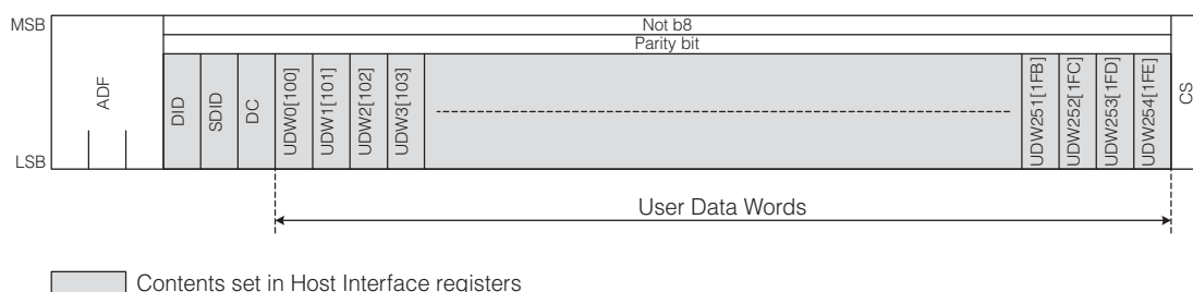
Figure 4-21: Arbitrary Data Packet Structure
