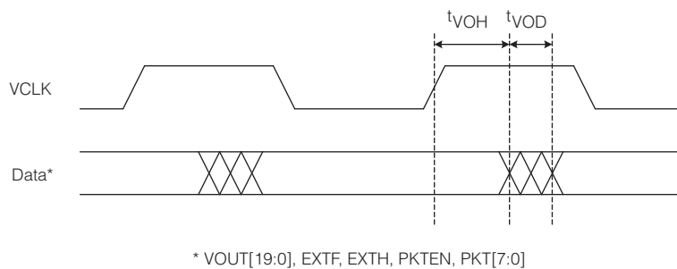
Figure 2-2: Video Data Output Delay & Hold Time
