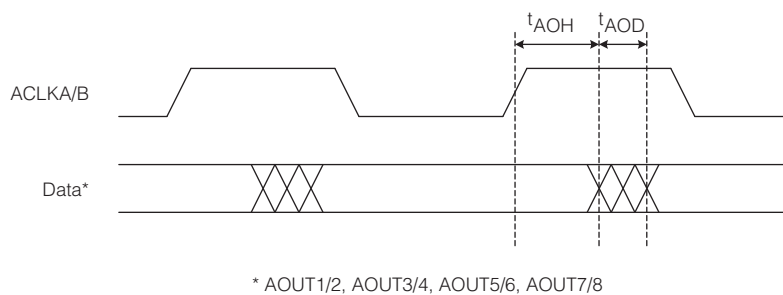
Figure 2-4: Audio Data Output Delay & Hold Time
