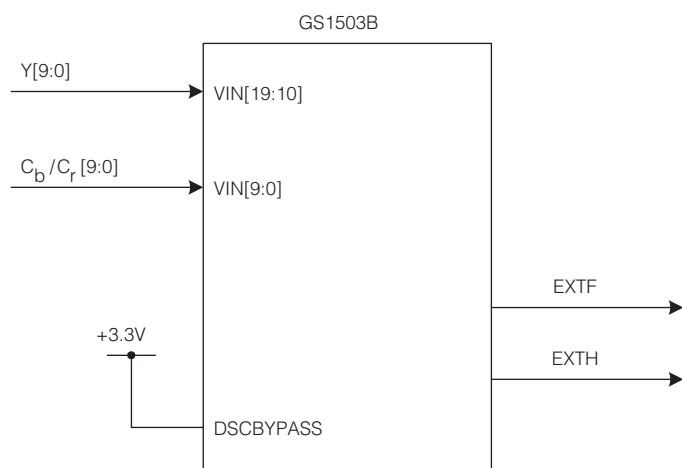
Figure 4-1: Configuration for 10-bit Y and C b /C r Input Video with TRS and Line Numbers
