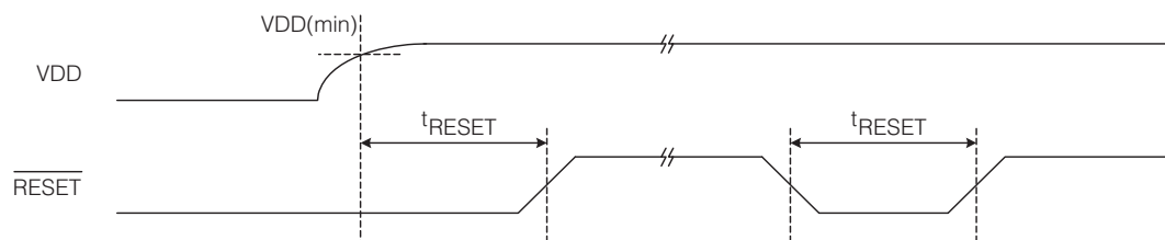
Figure 2-5: Reset Timing
