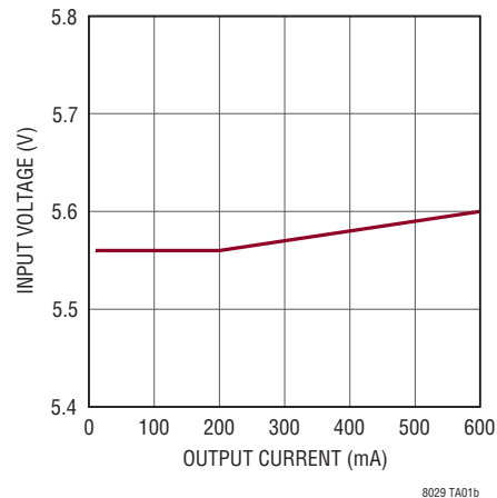
Minimum Input Voltage vs Output Current
