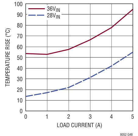
Temperature Rise vs Load Current 24V_{OUT}
