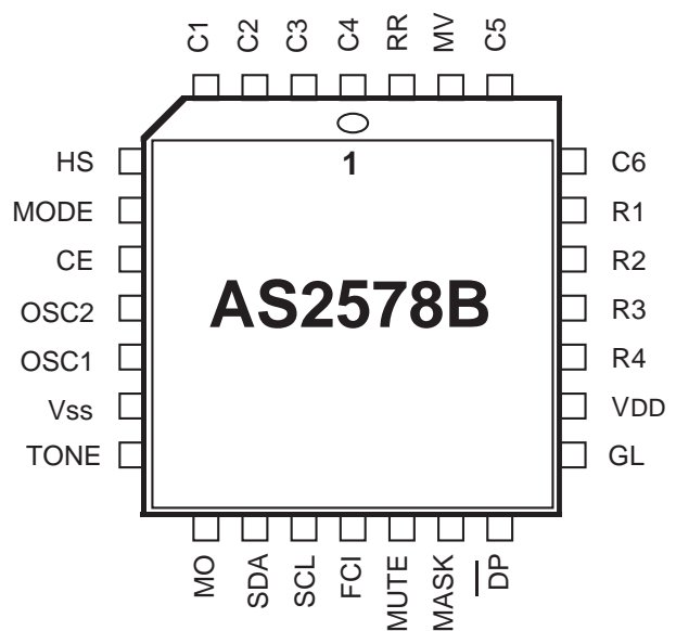
28 Pin PLCC
