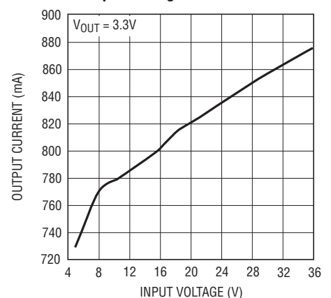
Output Short-Circuit Current vs Input Voltage
