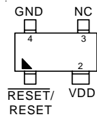
SC-82
