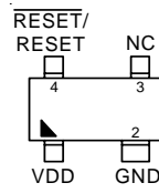
SC-82 (R-Type)
