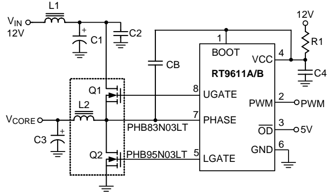
Figure 6. Synchronous Buck Converter Circuit
