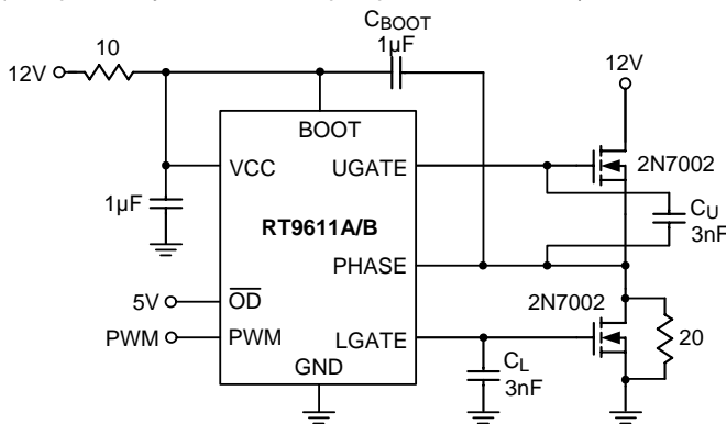
Figure 3. Test Circuit
