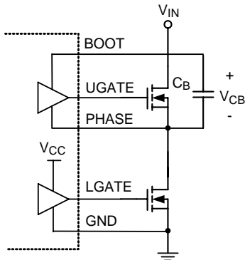
Figure 2. Part of Bootstrap Circuit of RT9611A/B
