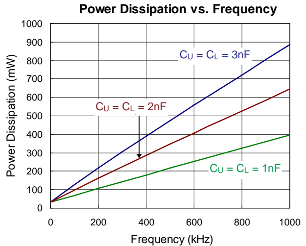
Figure 4. Power Dissipation vs. Frequency
