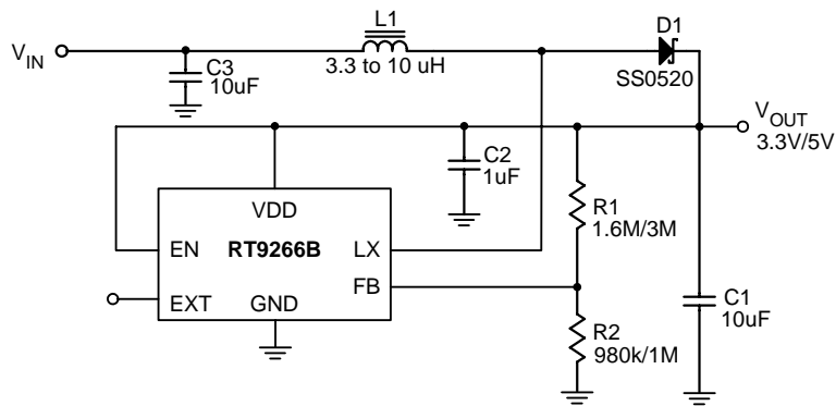
Figure 1. RT9266B Typical Application for Portable Instruments
