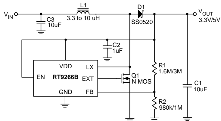
Figure 2. RT9266B for Higher Current Applications
