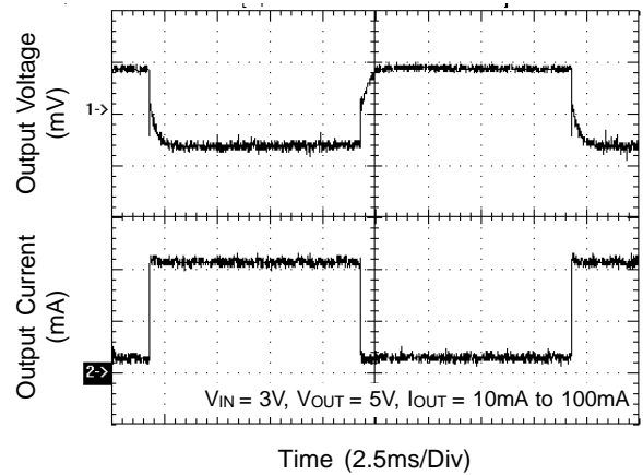
Load Transient Responses
