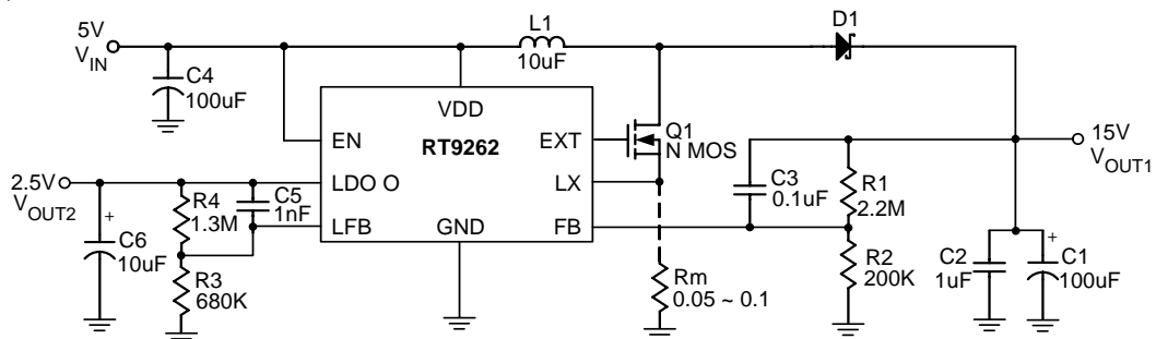
Figure 5. High Voltage Application ( R_m should be added when I_L > 100mA )
