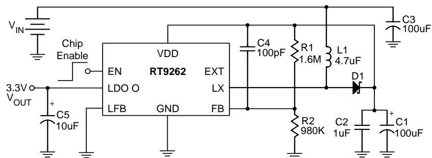
Figure 3. Application Circuit with Zero-Output-Current Shutdown Mode Control
