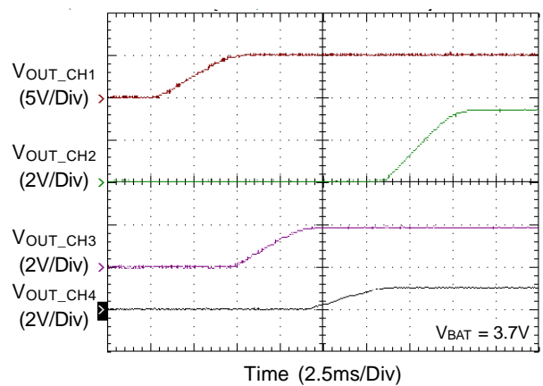
Power On Sequence
