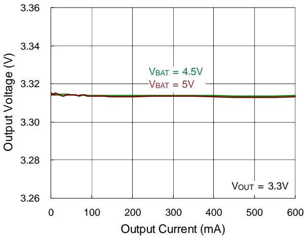
CH2 Step-Down Output Voltage vs. Output Current
