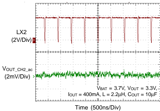
CH2 Output Voltage Ripple
