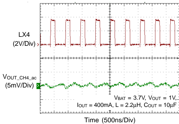
CH4 Output Voltage Ripple
