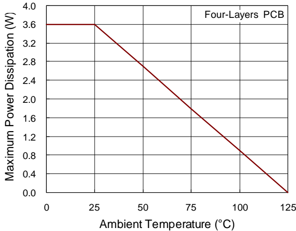
Figure 1. Derating Curves for RT9986 Packages
