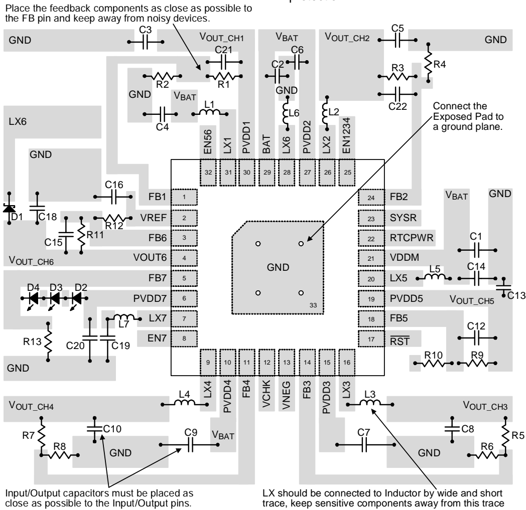
Figure 2. PCB Layout Guide
