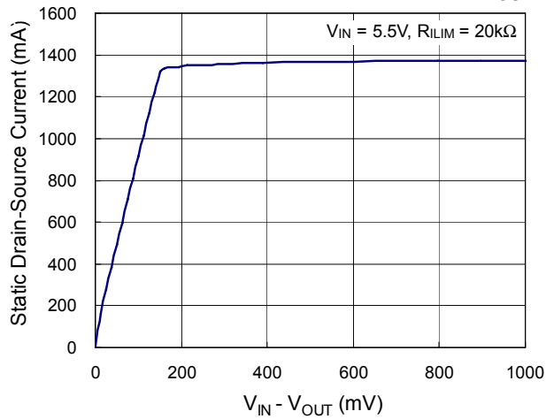
Static Drain-Source Current vs. V_{IN} - V_{OUT}
