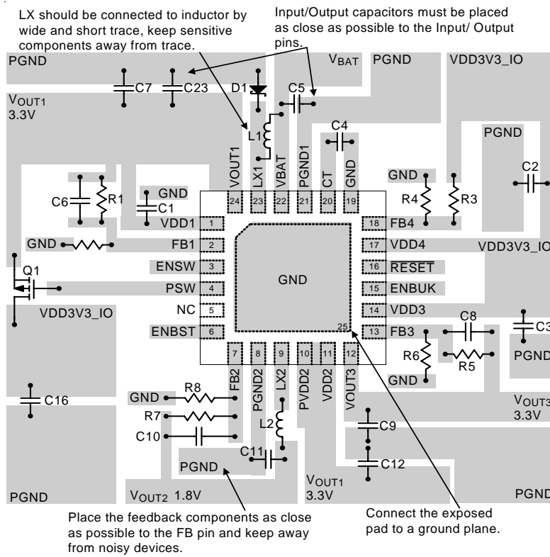
Figure 3. PCB Layout Guide
