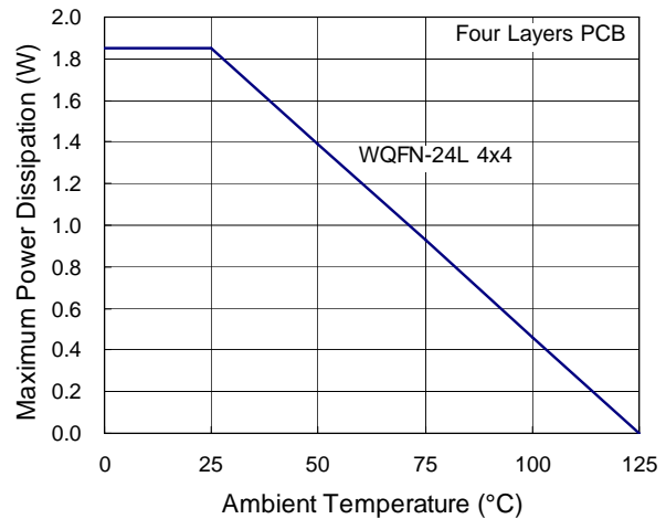
Figure 2. Derating Curves for RT9912A Packages
