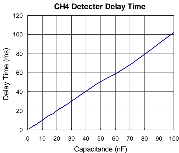
Figure 1. Detector Delay Time
