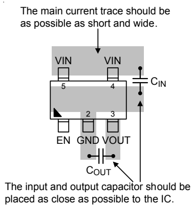
Figure 3. PCB Layout Guide for SOT-23-5 Package
