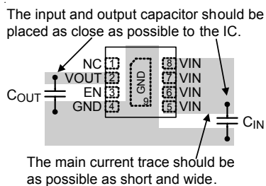
Figure 4. PCB Layout for WDFN Package
