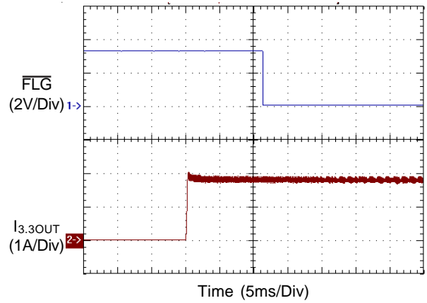
FLG Response In 3.3VOUT Short Circuit
