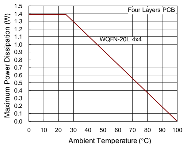
Figure 7. Derating Curves for RT9716A/B Packages
